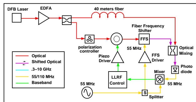
Figure 1: (color) Basic Proof-of-Principle Setup
