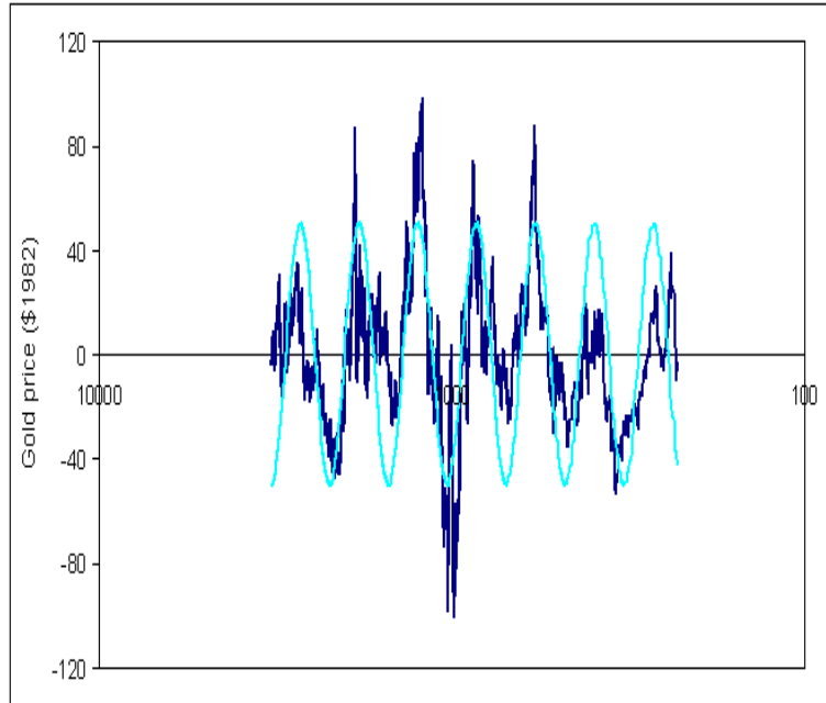
Fig. 7. Logarithmic scale deviations from hyperbolic trend in the gold price dynamics, 2002–2010 (X-axis indicates temporal distance in days from the critical time point)
