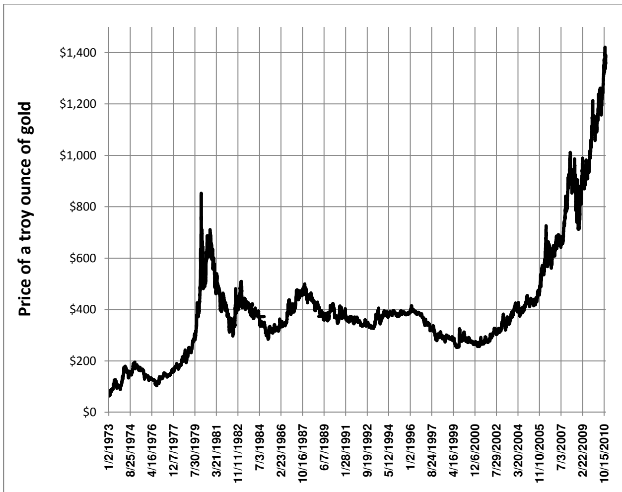
Fig. 3. Daily gold price dynamics, 1973–2010, US dollars
