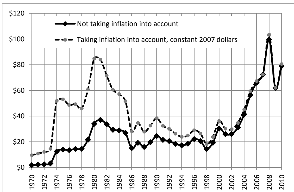
Fig. 2. Yearly oil price dynamics, 1970–2010
