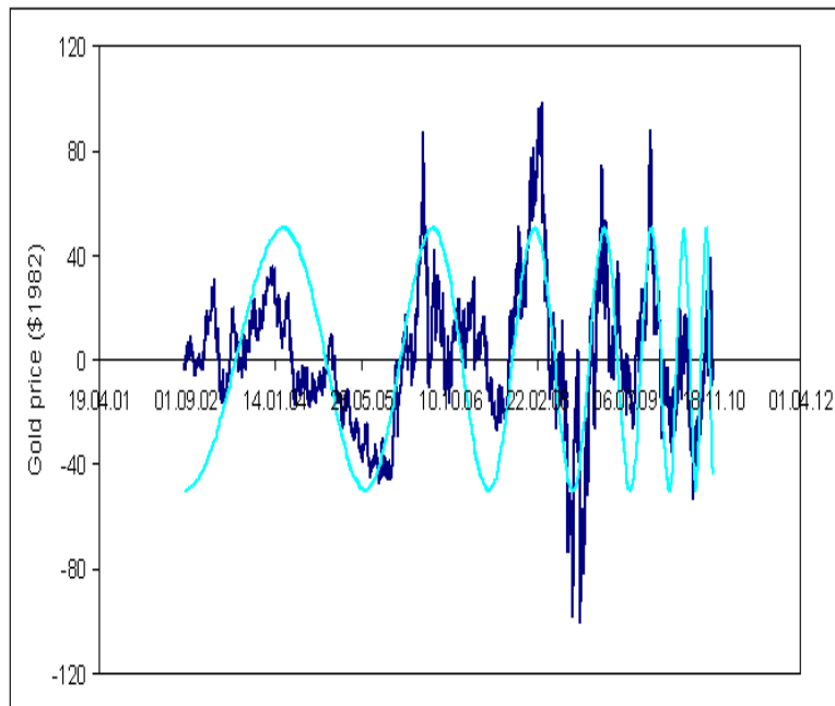
Fig. 6. Deviations from hyperbolic trend in the gold price dynamics, 2002–2010
