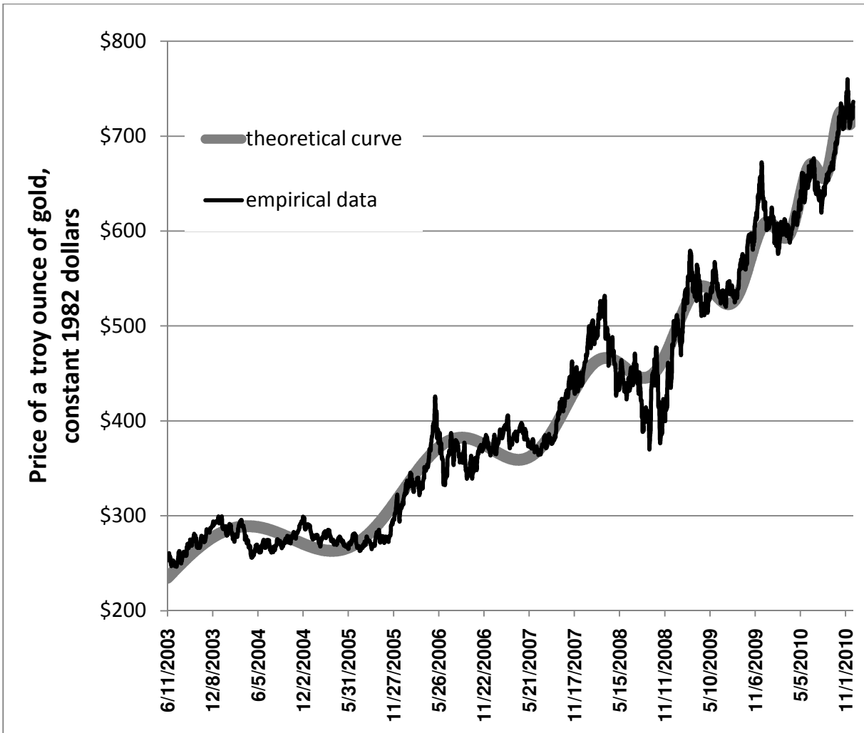
Fig. 4. Log-periodic oscillations in the gold price dynamics, daily prices, June 11, 2003 – December 2, 2010 (taking inflation into account; constant 1982 dollars)
