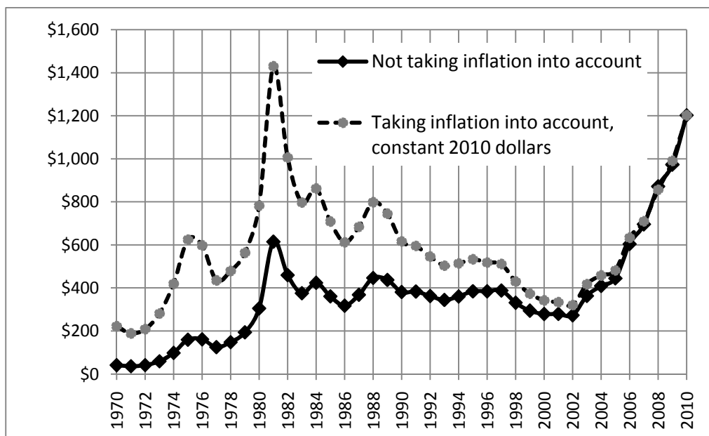
Fig. 1. Yearly gold price dynamics, 1970–2010
