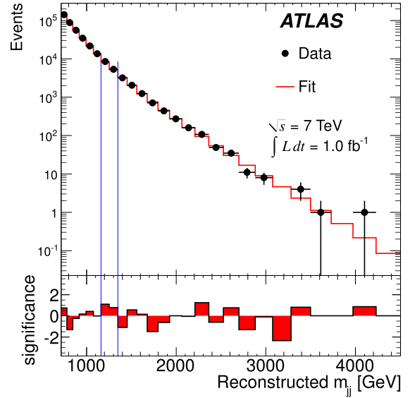
Fig. 1. The reconstructed dijet mass distribution (filled points) fitted with a smooth functional form describing the QCD background. The bin-by-bin significance of the data-background difference is shown in the lower panel. Vertical lines show the most significant excess found by the BUMPHUNTER algorithm (see text).
