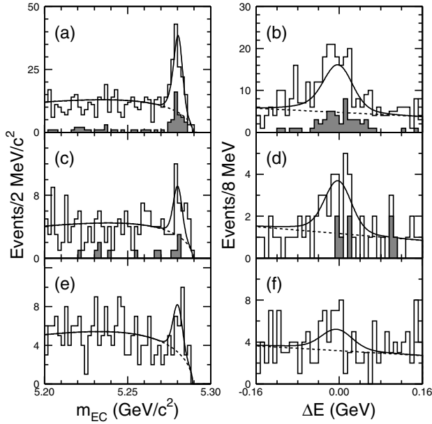
FIG. 2. B candidate m_{EC} and \Delta E for B^+ \rightarrow \eta' K^+ (a),(b), B^0 \rightarrow \eta' K^0 (c),(d), and B^+ \rightarrow \omega\pi^+ (e),(f). Histograms represent data, with the \eta' \rightarrow \eta\pi\pi subset shaded, the solid curves represent the full fit functions, and the dashed curves represent the background functions.
