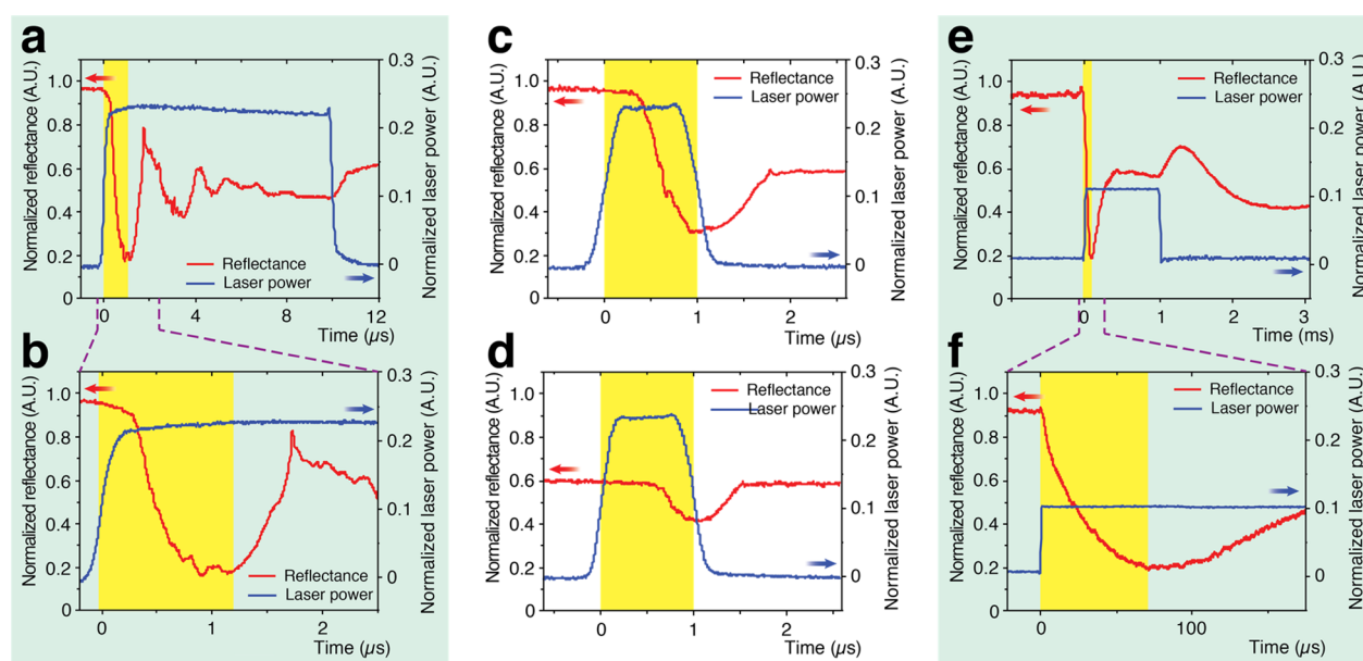
Figure 2. Results of time-resolved in situ optical probing. The dynamic response of the system upon exposure to 532 nm laser irradiation is characterized by the reflectance of the 633 nm laser signal (red traces), of which the initial drops (indicated by the yellow shadows) represent the dissolution process of the P3HT:F4TCNQ thin film within the probed region. Blue traces indicate the signal from the photodetector that collects the minor branch of the 532 nm processing laser, as a time reference. (a) Typical reflectance response of the system under high laser power (40 mW, 10 \mu s) with the enlargement (b) of the reflectance response, showing that the temperature-induced dissolution process takes 1.2 \mu s. (c,d) Reflectance response of the system to 532 nm laser pulses with a power of 40 mW and duration of 1 \mu s, verifying that the time needed for full dissolution is more than 1 \mu s. The first 1 \mu s pulse (c) induces a similar response, and the initial drop magnitude is close to but smaller than that of the 10 \mu s pulse case (87%). The second 1 \mu s pulse (d) also induces an observable drop, indicating that the first 1 \mu s pulse does not support the full dissolution of the probed region. (e) Typical reflectance response of the system upon exposure to low-intensity laser irradiation. The processing laser used is 15 mW, and the pulse duration is 1 ms. (f) The enlargement of the reflectance response in panel (e), showing that it takes around 70 \mu s for the dissolution process to finish.
