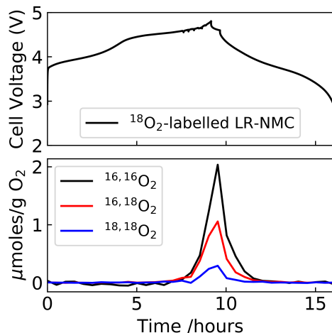
Figure S5. Charge-discharge profile and O 2 evolution in the 18 O 2 -labelled, as-received LR-NMC material as measured by DEMS.
