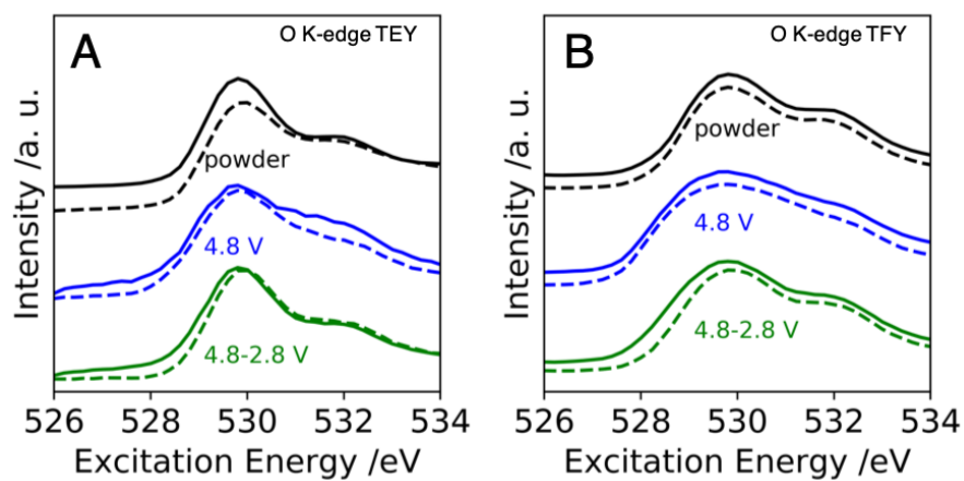
Figure S8. Soft X-ray absorption spectra of the LR-NMC oxide materials: O K-edge spectra (as-received as solid lines, surface-treated as dashed lines) of the powders (in black), and electrodes at different states of charge in the surface-sensitive TEY mode and bulk-sensitive TFY modes as indicated.
