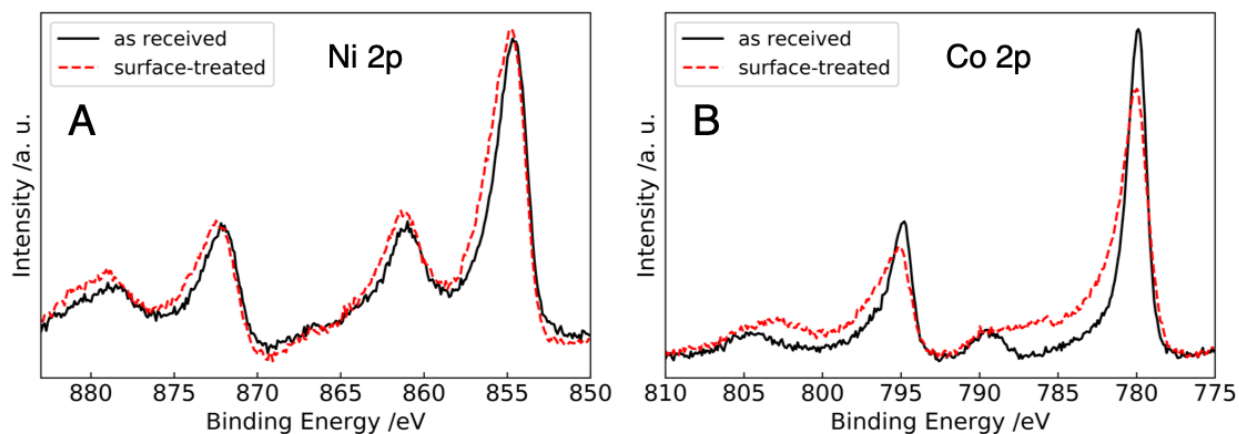
Figure S6. Comparison of the (A) Ni 2p and (B) Co 2p XPS spectra in the as-received and surface-treated Li-rich NMC oxide materials.
