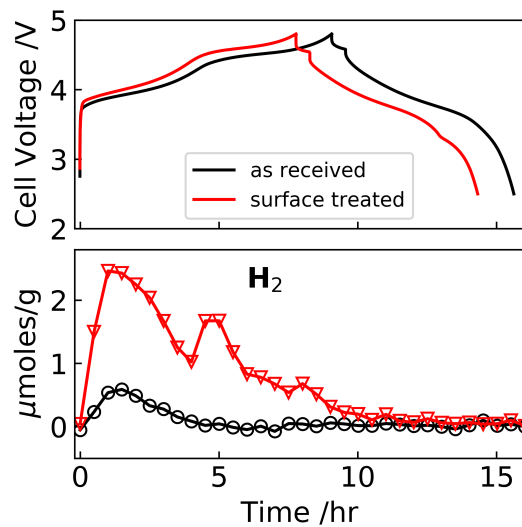
Figure S1. H 2 evolution during the first charged/discharge cycle of the as-received and surface-treated LR-NMC electrodes, as measured by DEMS.
