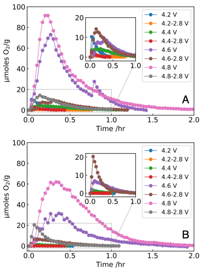
Figure S2. O 2 evolution during ex-situ titrations of the charged/discharged electrodes of the (A) as-received and (B) surface-treated samples with 3.5 M H 2 SO 4 , as measured by DEMS.
