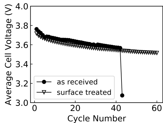
Figure S9. Variation of the average cell voltage during coin-cell cycling with a Li-foil anode.
