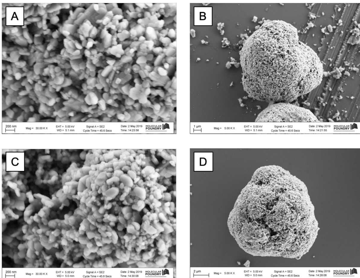
Figure S10. Scanning electron micrographs of (A)-(B) the as-received Li-rich NMC oxide powder, and (C)-(D) after surface acidic treatment.
