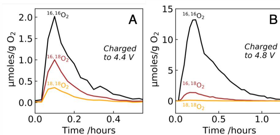
Figure S4. O 2 evolution from ex-situ titrations of 18 O-labelled Li-rich NMC oxide electrodes charge to A) 4.4 V and B) 4.8 V.
