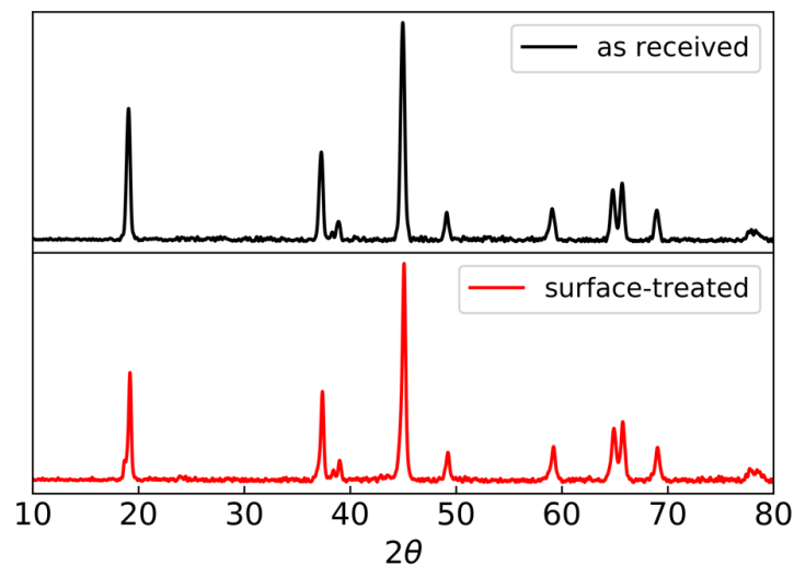
Figure S7. Powder X-ray diffraction pattern (Cu K \alpha ) of the as-received and surface-treated materials.
