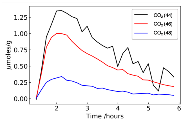
Figure S3. CO 2 evolution from the titration of the 18 O-enriched Li-rich NMC oxide powder with 10 M H 2 SO 4 , as measured by DEMS. The C 16,16 O 2 , C 16,18 O 2 and C 18,18 O 2 evolved are denoted by their M/Z values of 44, 46 and 48 respectively.
