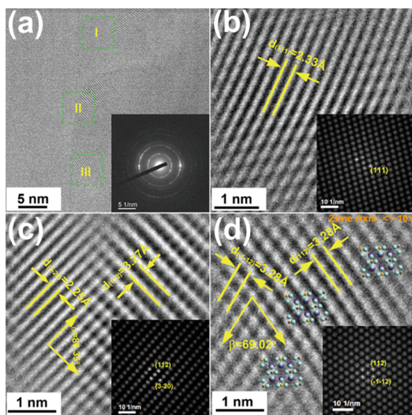
Figure 1. (a) HRTEM image of the K 2 SiF 6 :Mn 4+ phosphor. The inset shows the selected area electronic diffraction patterns. (b–d) enlarged HRTEM regions (I–III) in (a), respectively, and their corresponding FFT patterns.
