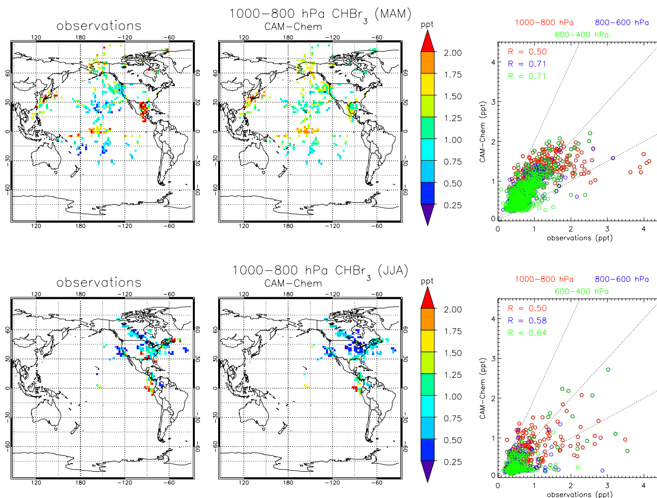
Fig. 3. Composite of (left) aircraft observations of \text{CHBr}_3 and (centre) simulated \text{CHBr}_3 in the lower-troposphere (1000–800 hPa) during (top) March–May and (bottom) June–August. The corresponding scatter-plots of simulated vs. observed \text{CHBr}_3 during the same periods are shown on the right-hand side for 1000–800 hPa (red) as well as for two additional tropospheric layers (800–600 hPa, blue; 600–400 hPa, green); R represents the Pearson correlation coefficient for those layers. The 1:2, 1:1 and 2:1 lines are illustrated by dots. Model output was sampled at the same location and month as the observations, which in turn are averaged over the 1.9^\circ (lat) \times 2.5^\circ (lon) horizontal grid cells of CAM-Chem.
