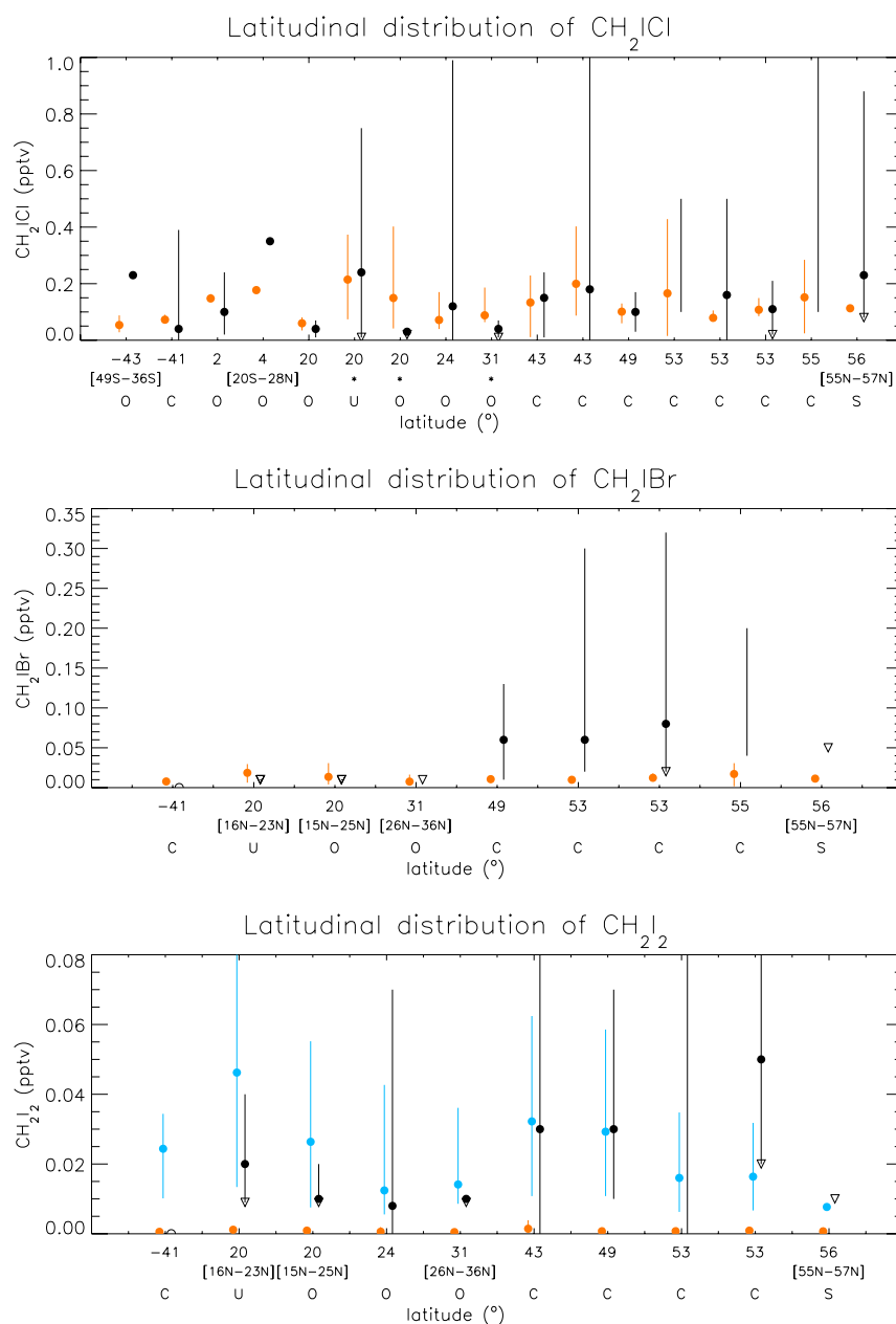
Fig. 11. Comparison of observed (black) and modelled (orange) mixing ratios of \text{CH}_2\text{ICl} (top), \text{CH}_2\text{IBr} (middle) and \text{CH}_2\text{I}_2 (bottom). The observations, which are also summarised in Table 2, have been ordered along the x-axis according to their latitude from South to North. The range of latitudes is shown in brackets if the observations cover a region instead of a single point (this is sometimes indicated by stars in the case of \text{CH}_2\text{ICl} due to reasons of space). They have been classified as open ocean (O), upwelling (U), shelf (S), and coast (C). The full black circles represent the average of the observed values and the black bars correspond to their range, given by the minimum–maximum or by the 10th–90th percentiles depending on the dataset. The minimum observed value is indicated by an open triangle when it corresponds to an upper limit, while some very low observations on a cliff-top location (expected to be lower estimates) are depicted by an open circle. Orange circles represent the average modelled fields for the location and month(s) of the observations. When observations cover a geographical region the minimum and maximum monthly modelled values over that area are also depicted by orange bars; otherwise the mean, minimum and maximum of the monthly modelled fields on the 9 model grid cells closest to the location of the measurements are plotted. In the case of \text{CH}_2\text{I}_2 , results from an additional model simulation are shown in blue to reflect the importance of the daily cycle of emissions for these species (see details in text).
