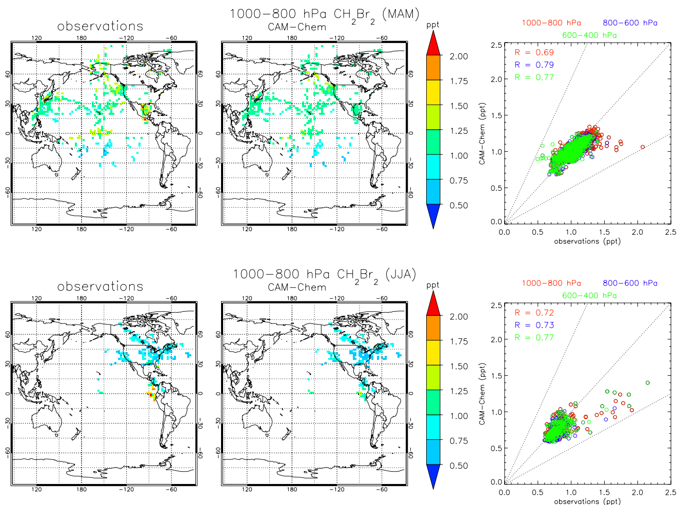
Fig. 4. Same as Fig. 3 but for \text{CH}_2\text{Br}_2 .
