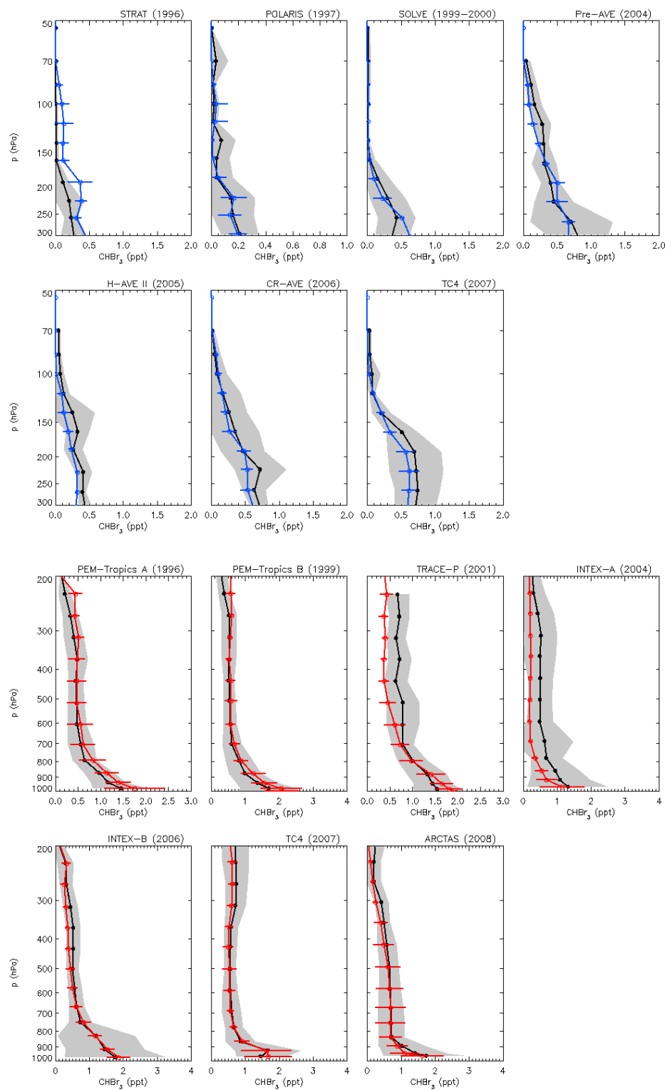
Fig. 7. Comparison of observed and simulated vertical profiles of \text{CHBr}_3 for a number aircraft missions in the UTLS region and the troposphere. Black lines and grey shaded areas indicate the mean and one standard deviation of the observations. Blue (red) lines and horizontal bars show the mean and one standard deviation of the simulated \text{CHBr}_3 field at the same locations and during the same months as the observations in the UTLS (troposphere).
