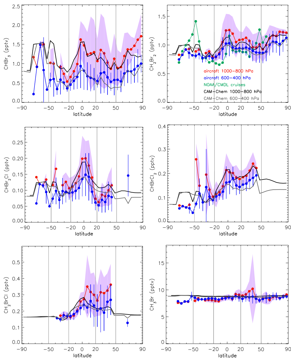
Fig. 5. Latitudinal dependence of the observed and modelled bromocarbons \text{CHBr}_3 , \text{CH}_2\text{Br}_2 , \text{CHBr}_2\text{Cl} , \text{CHBrCl}_2 , \text{CH}_2\text{BrCl} and \text{CH}_3\text{Br} averaged for each 2.5^\circ latitudinal band within 1000–800 hPa and 600–400 hPa. When at least two data points are available for a given latitudinal band, shaded areas and vertical bars indicate standard deviations of the aircraft observations for 1000–800 hPa and 600–400 hPa, respectively. Model output corresponds to the location and month of the aircraft observations when available, otherwise all CAM-Chem output for that latitude is used. In the case of \text{CH}_2\text{Br}_2 , observations from NOAA/CMDL vessels from 1994 to 2004 are also shown in green colour.
