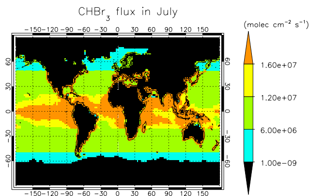
Fig. 2. Global emission distribution of \text{CHBr}_3 estimated for July.
