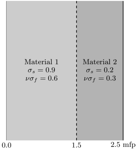
Figure 6.3: Heterogeneous Multiplying Slab Benchmark Problem Domain from [47]
