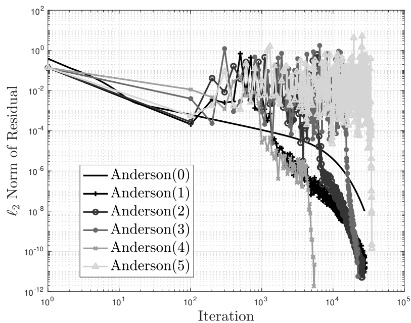
Figure 8.4: Anderson Acceleration Convergence for Sood Criticality Problem 73 ( \beta_n = 0.5 ), No Initial Fixed-Point Iterations
