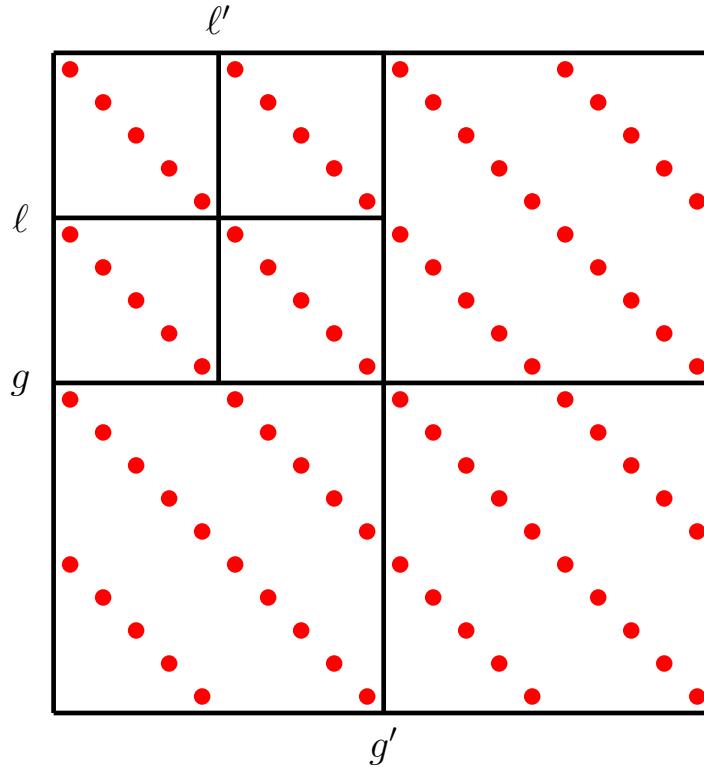
Figure 3.2: Structure of \Sigma_{\mathbf{f}} for Two Energy Groups, Five Spatial Cells, and Fission in All Energy Groups
