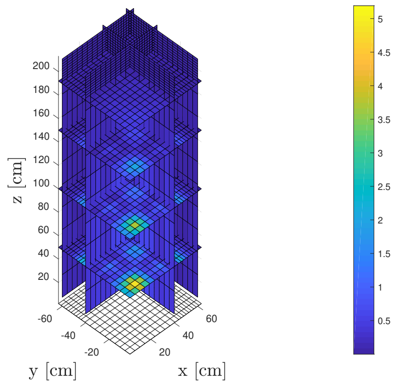
(g) Scalar Flux for Energy Group Six
