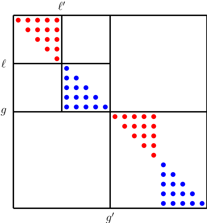
Figure 3.1: Structure of \mathbf{H}_z^{-1}
