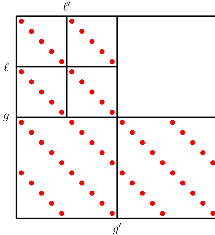
Figure 3.3: Structure of \Sigma_{\mathbf{s}} for Two Energy Groups, Five Spatial Cells, and Downscattering Only
