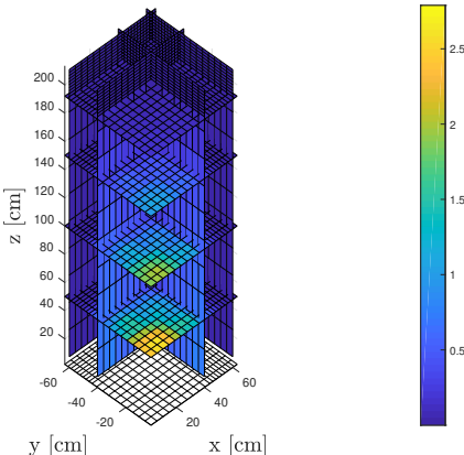
(e) Scalar Flux for Energy Group Four
