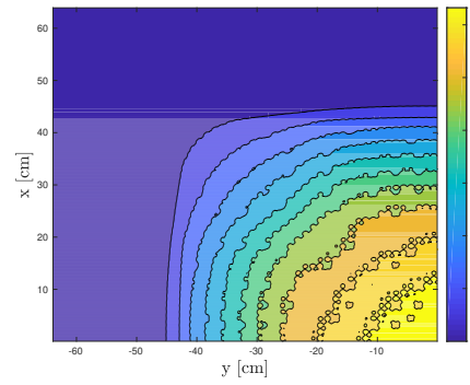
(b) Scalar Flux for Energy Group One
