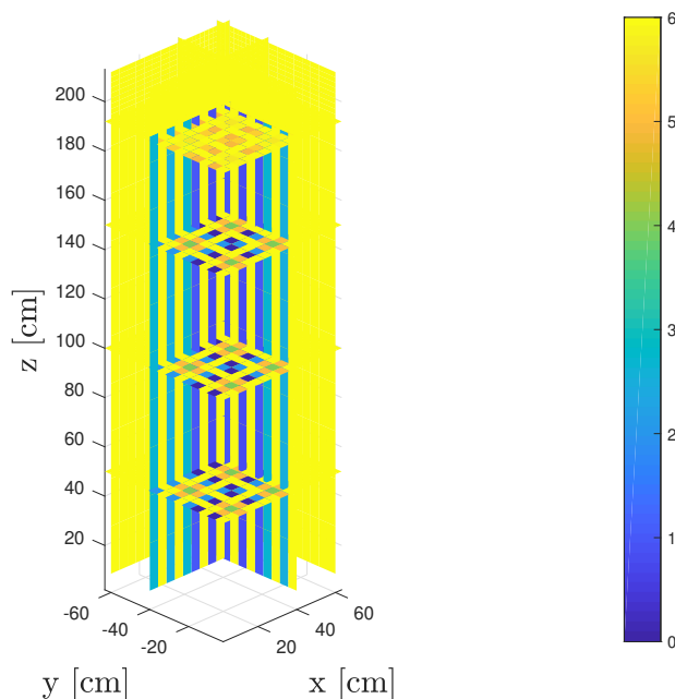
Figure 7.11: Coarse Spatial Homogenization of Three-Dimensional MOX Fuel Assembly Benchmark Problem
