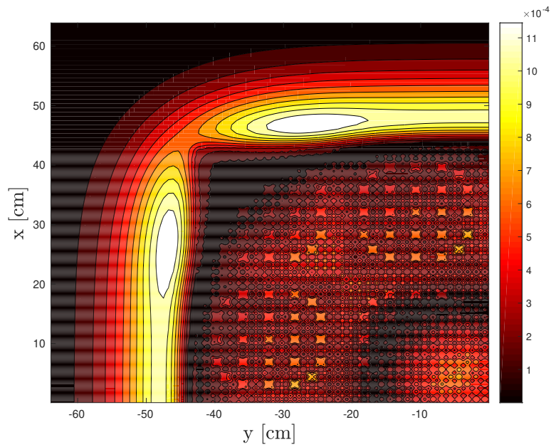
Figure 7.10: Absolute Difference between Alpha- and k -Effective Eigenvalue Group Six Scalar Fluxes (Fine Homogenization)
