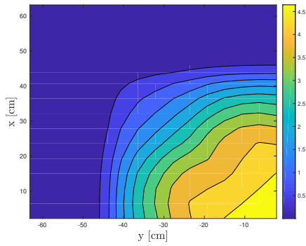
(a) Scalar Flux for Energy Group Zero
