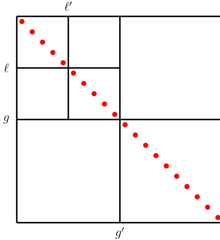
Figure 3.4: Structure of \mathbf{V}_z^{-1} for Five Spatial Cells
