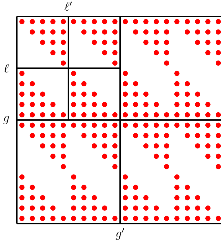
Figure 3.5: Structure of \mathbf{H}_z^{-1}\Sigma_f for Two Energy Group Example
