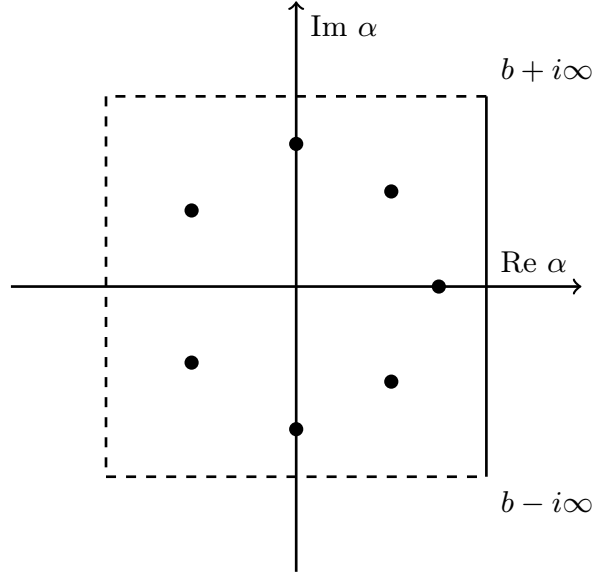
Figure 2.2: Contour Integration in Complex Plane of the Operator \mathcal{A}
