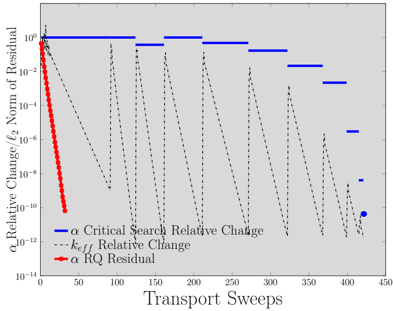
(a) Convergence of Rayleigh Quotient Fixed Point and Critical Search Methods for Sood Prob. 1 Cross Section Set
