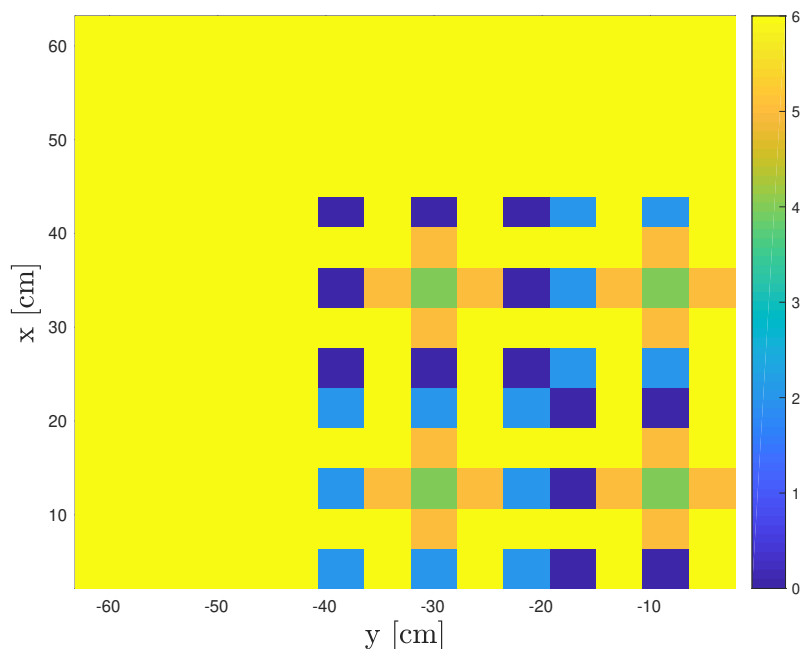
Figure 7.5: Coarse Spatial Homogenization of MOX Fuel Assembly Benchmark Problem. Each material is given a number which corresponds to the color shown in the figure: UO_2 = 0 , 4.3% MOX Fuel = 1, 7.0% MOX Fuel = 2, 8.7% MOX Fuel = 3, Guide Tube = 4, Fission Chamber = 5, Moderator = 6.
