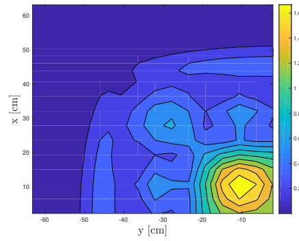
(f) Scalar Flux for Energy Group Five
