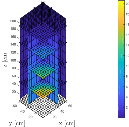
(b) Scalar Flux for Energy Group One
