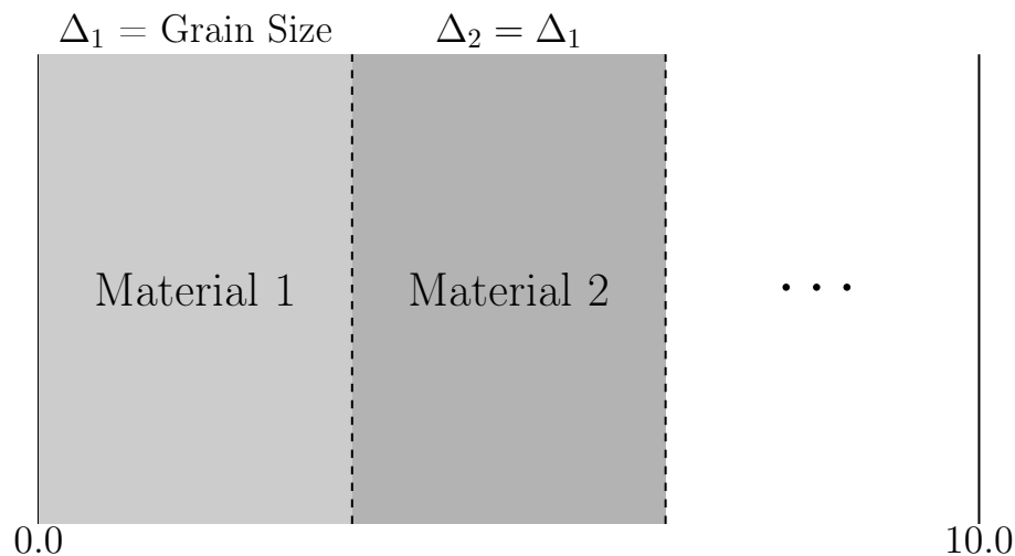
Figure 6.1: Heterogeneous Slab Benchmark Problem Domain
