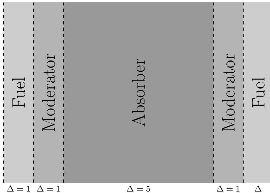
Figure 6.5: Five Region Heterogeneous Slab Benchmark Problem Domain
