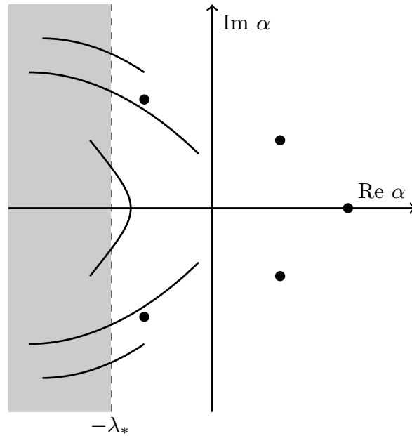
Figure 2.3: Example Spectrum of the Transport Operator for the One-Speed Slab Geometry Problem
