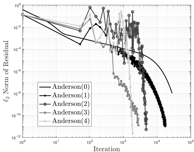
Figure 8.3: Anderson Acceleration Convergence for Sood Criticality Problem 73 ( \beta_n = 1 ), No Initial Fixed-Point Iterations
