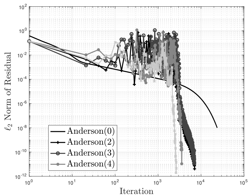
Figure 8.1: Anderson Acceleration Convergence for Sood Criticality Problem 68 ( \beta_n = 1 ), No Initial Fixed-Point Iterations
