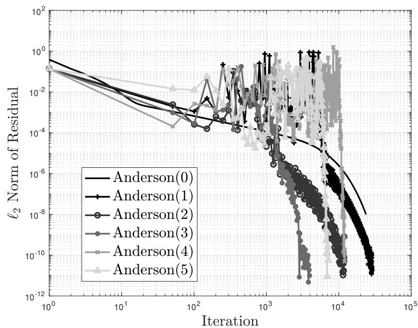
Figure 8.2: Anderson Acceleration Convergence for Sood Criticality Problem 68 ( \beta_n = 0.5 ), No Initial Fixed-Point Iterations
