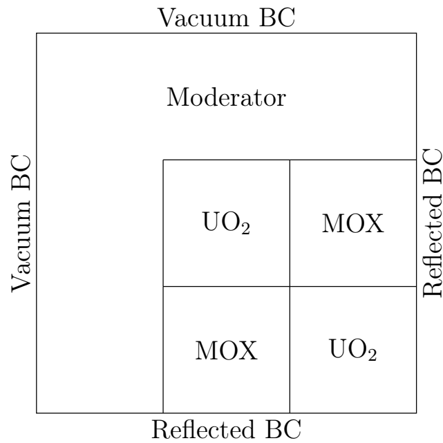
Figure 7.3: Assembly Layout for MOX Fuel Assembly Benchmark
