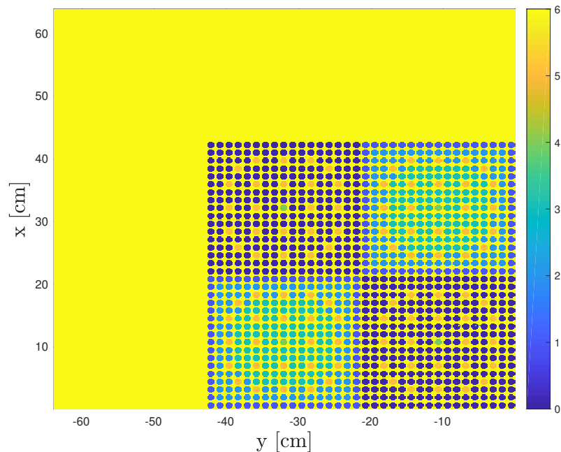
Figure 7.8: Fine Spatial Homogenization of MOX Fuel Assembly Benchmark Problem. The color in each cell corresponds to the material in that cell. Each material is given a number which corresponds to the color shown in the figure: UO_2 = 0 , 4.3% MOX Fuel = 1, 7.0% MOX Fuel = 2, 8.7% MOX Fuel = 3, Guide Tube = 4, Fission Chamber = 5, Moderator = 6.
