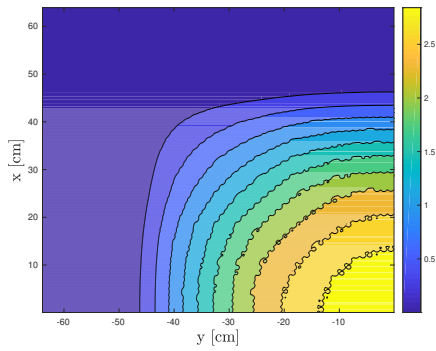
(c) Scalar Flux for Energy Group Two
