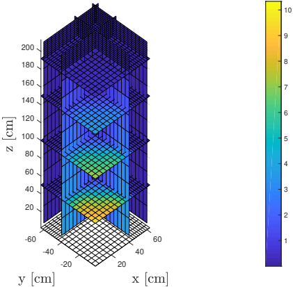
(a) Scalar Flux for Energy Group Zero
