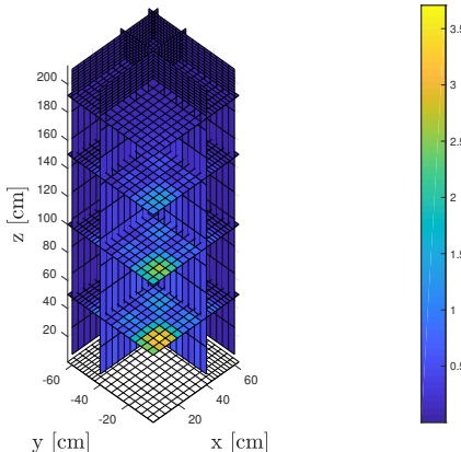
(f) Scalar Flux for Energy Group Five
