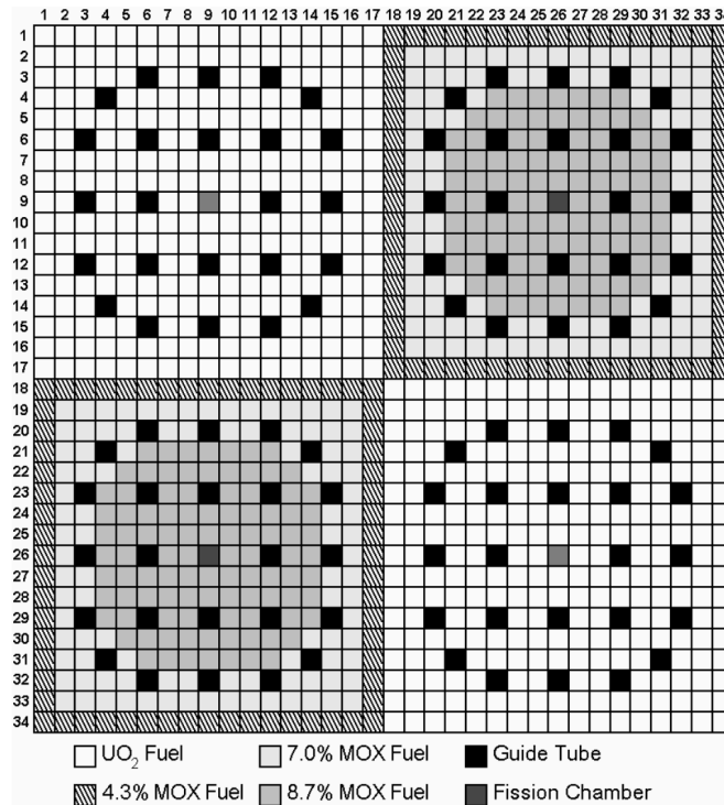
Figure 7.4: Fuel Pin Layout for MOX Fuel Assembly Benchmark from [49]
