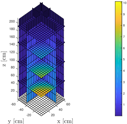
(c) Scalar Flux for Energy Group Two
