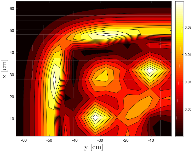
Figure 7.7: Absolute Difference between Alpha- and k -Effective Eigenvalue Group Six Scalar Fluxes (Coarse Homogenization)
