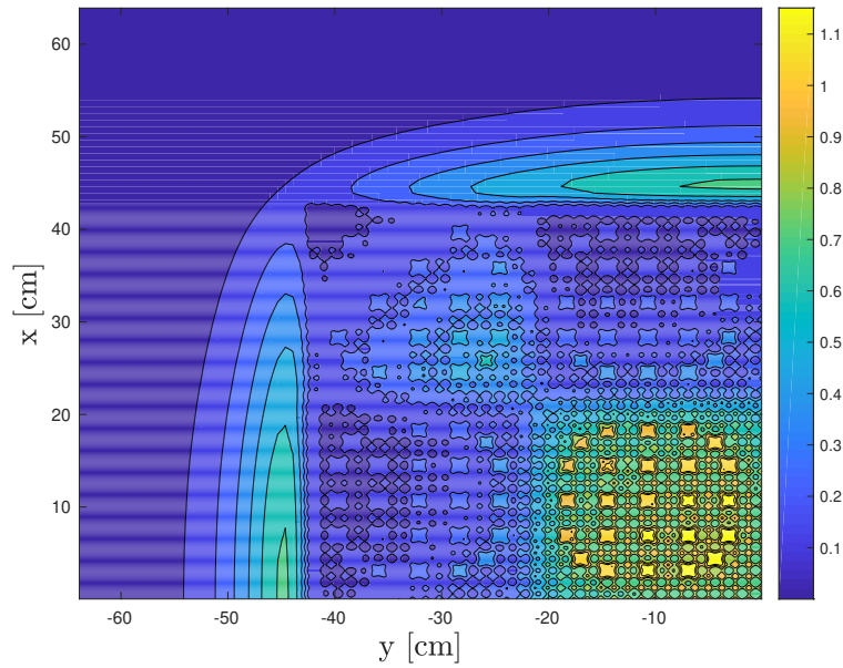
(g) Scalar Flux for Energy Group Six
