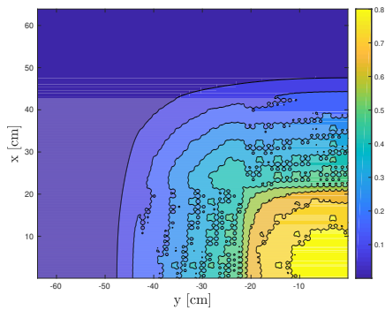
(e) Scalar Flux for Energy Group Four
