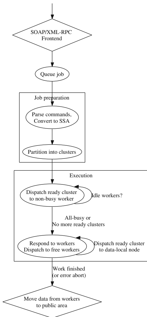
Fig. 5 Simplified flowchart
