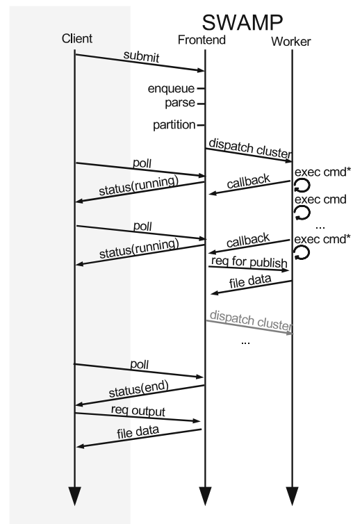
Fig. 2 Simplified timeline for a SWAMP task
