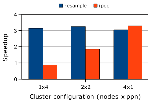
Fig. 10 Speedup in three cluster configurations
