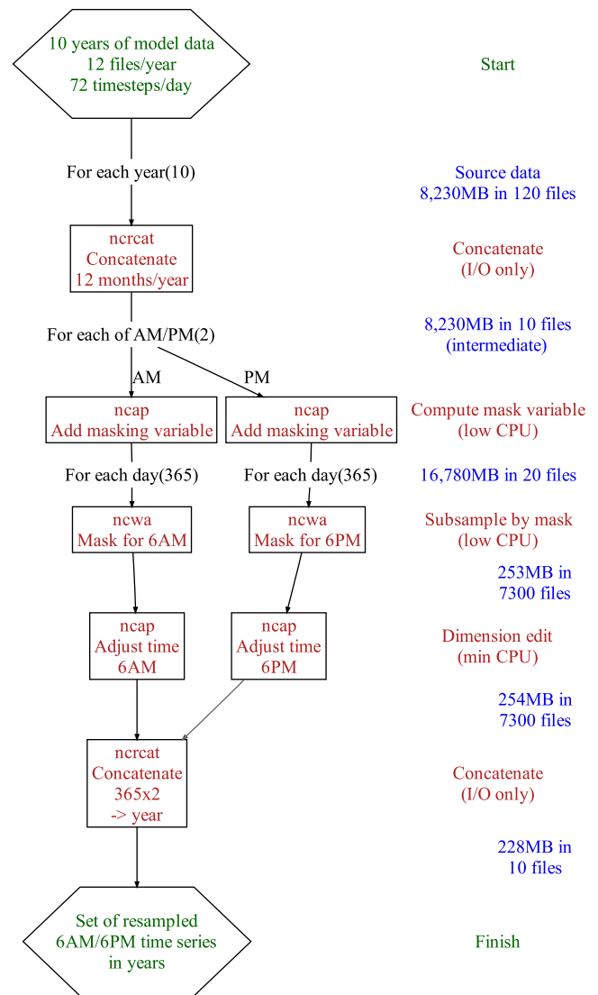
Fig. 6 Benchmark 1: resample —data resample
