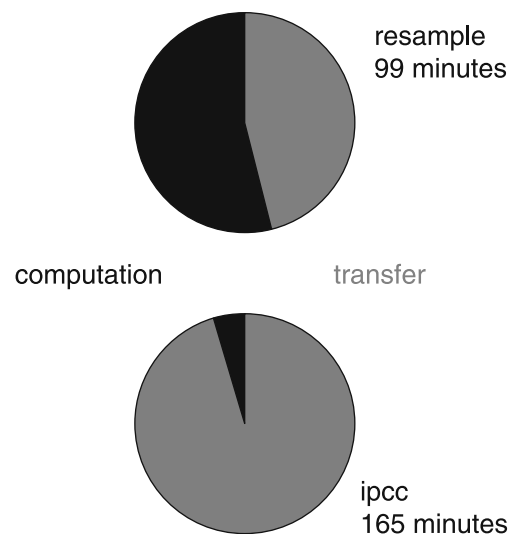
Fig. 4 Components of total wall-clock time for the benchmarks
