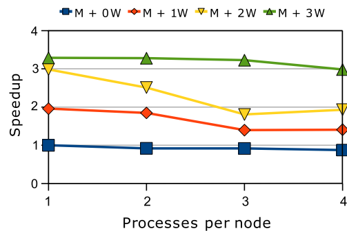
Fig. 11 ipcc speedup by PPN for various cluster configurations
