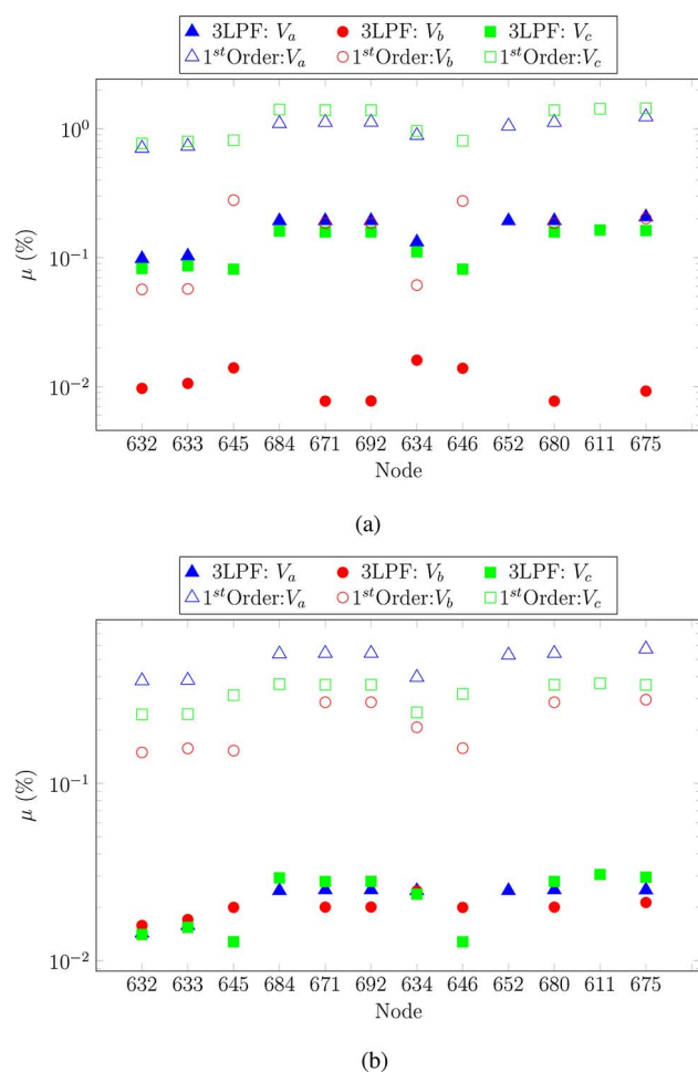
Fig. 11. Relative error of power flow solutions obtained by the 1st Order method of [20] and the 3LPF for the IEEE 13-Node system. (a) Tap changer set at \{1.0625, 1.05, 1.0687\} , (b) Tap changer set at \{1, 1, 1\} .
