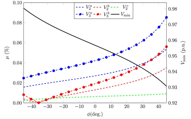
Fig. 7. Relative error of the 3LPF versus loads power factor.
