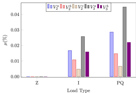
Fig. 8. Relative error of the 3LPF versus loads voltage dependence.
