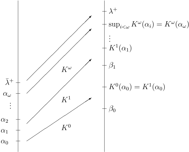
Figure 3.1: The game G(\langle \alpha_i \mid i < \omega \rangle, E) , where K^\omega is the common part of \langle K^i \mid i < \omega \rangle .
