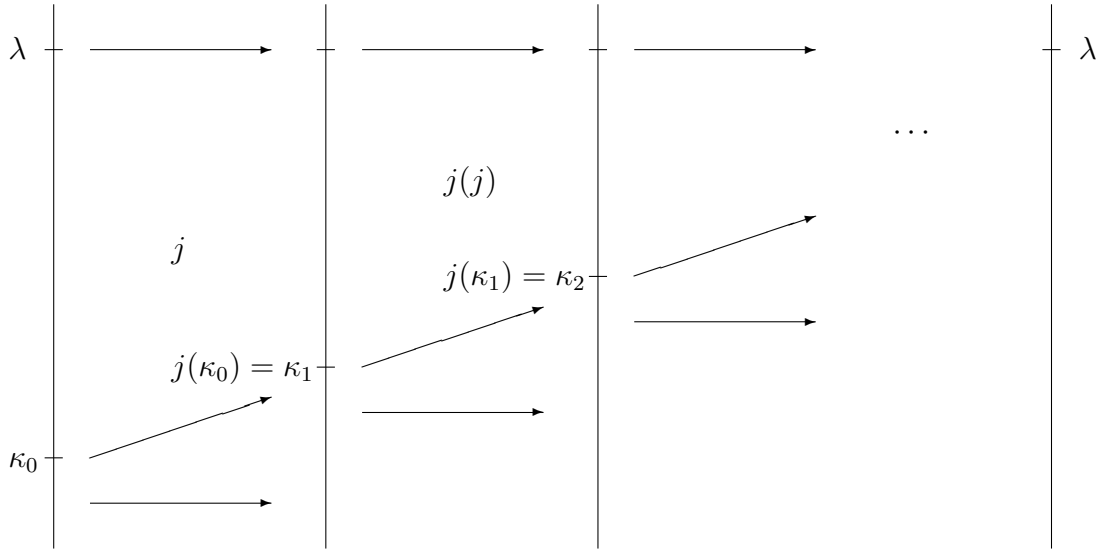
Figure 1.1: Rank-into-rank embeddings.
