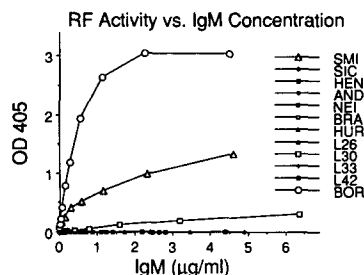
Figure 4. RF activity of each transfectoma protein compared with BOR. Ordinate is OD at 405 nm of the ELISA for RF activity measured on plates coated with total human IgG. The abscissa describes the IgM κ concentration (μg/ml) of the assayed sample. Symbols representing titration of each sample are indicated. In particular, (O) BOR, (Δ) SMI, and (□) binding activity of L30.
