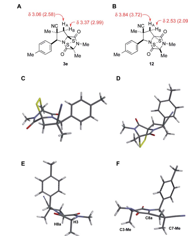
Fig. 3 Representative data used to assign the relative configuration of the disulfide bridge in ETP products, X-ray model of dioxopiperazine 8e , and a computation model of the derived angular enolate. (A and B) show the observed (in CDCl 3 ) and calculated (in parentheses) chemical signals of the methylene hydrogens of the pyrrolidine ring of ETP diastereomers 3e and 12 . (C) is the X-ray model of 3e . (D) is the computational model (B3LYP/631-G*) of 12 . (E) is the X-ray model of dioxopiperazine 8e . (F) is the predominant conformer (B3LYP/631-G*) of the angular enolate formed from dioxopiperazine 8e .
