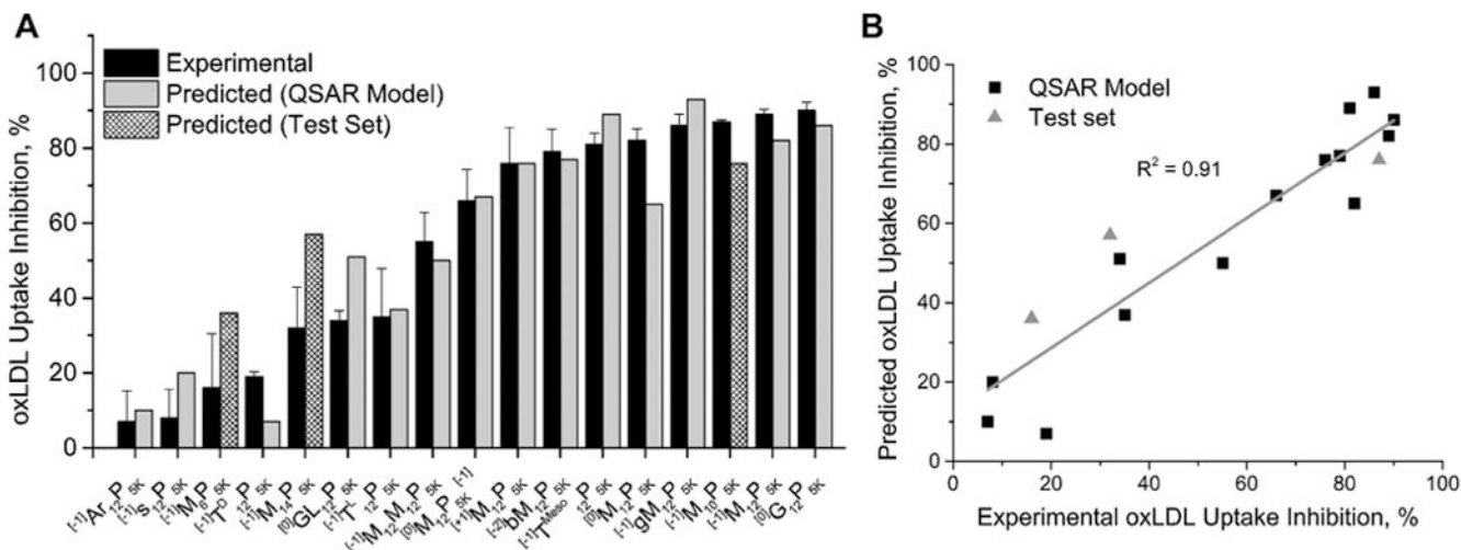
Fig. 6. The final QSAR model was successful at predicting the bioactivity (oxLDL uptake inhibition) of the new, three member AM test set. A) The QSAR fit showing that the residual from simulation is often within the S.E.M. from the experimental data. B) The linear fit of experimental vs. predicted outcomes with R^2 = 0.91 .
