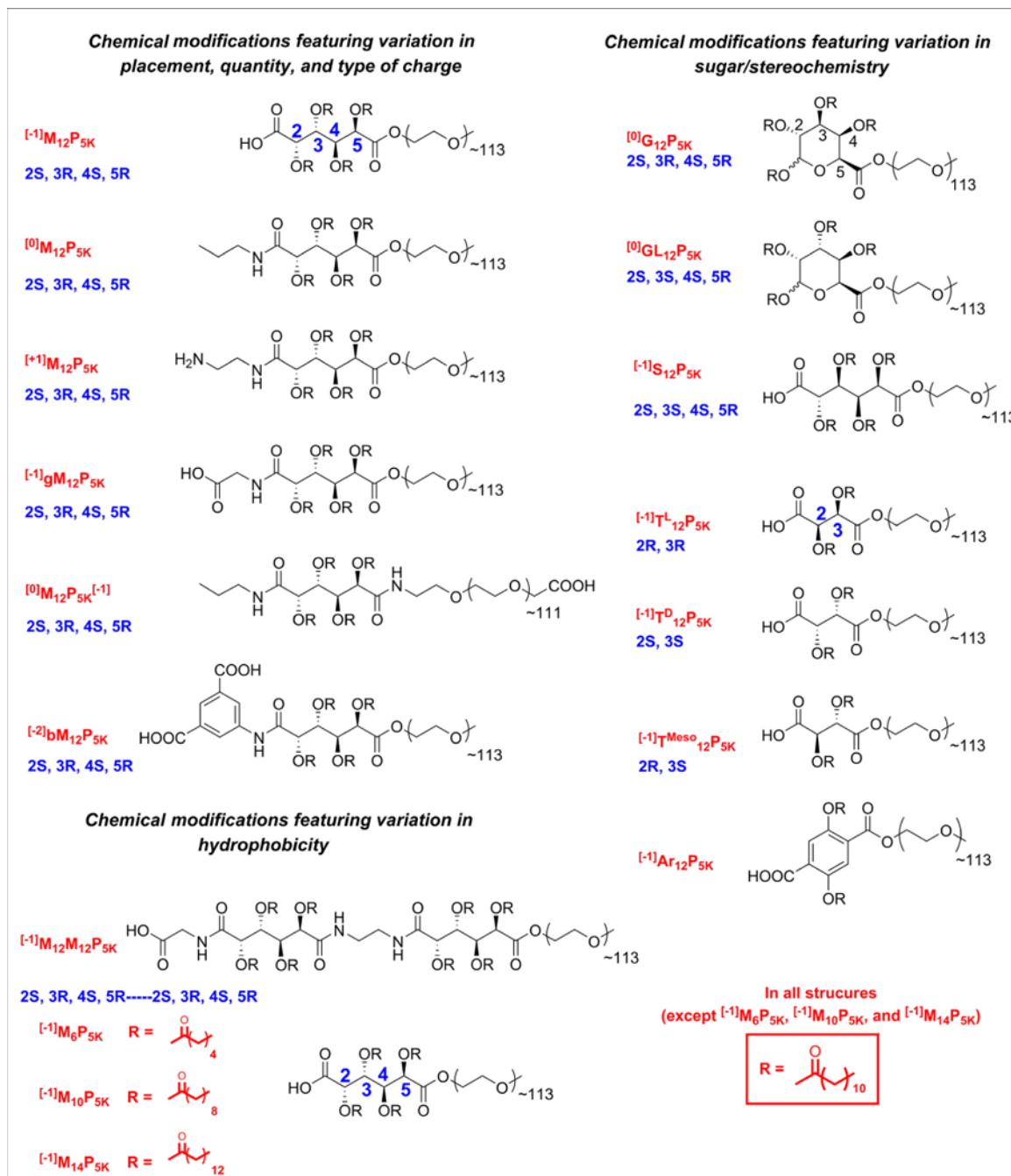
Fig. 1. Chemical compositions, stereochemistry, and associated abbreviations for AMs in this study. Nomenclature methodology: [\text{charge}]_{\text{Backbone}}^{\text{Stereochemistry}}_{\text{chain length}}P_{\text{PEG length}} . Backbone and functional group abbreviations: M = mucic acid, S = saccharic acid, T = tartaric acid, Ar = 2,5-dihydroxyterephthalic acid, G = D-galacturonic acid, GL = D-glucuronic acid, b = benzene, g = glycine.
