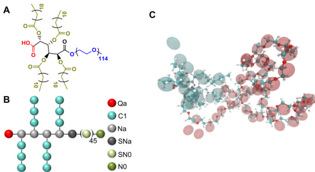
Fig. 4. A) The molecular and B) coarse grained structure of ^{[-1]}M_{12}P_{5K} shown in a ball-and-stick representation. C) The conformation of ^{[-1]}M_{12}P_{5K} along with its CG representation in the MARTINI force field where CG beads are shown as transparent spheres.
