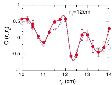
FIG. 3 (color online). Radial structure of zonal flow. The structure is estimated from correlation between potential differences at different toroidal locations. In this experiment, the observation radius of the second HIBP is varied around r_2 = 12 cm with the observation point of the first HIBP being fixed at r_1 = 12 cm. The closed circles represent the traditional correlation coefficient as a function of the observation radius of the second HIBP, while the open circles do coherent structure from FFT analysis.
