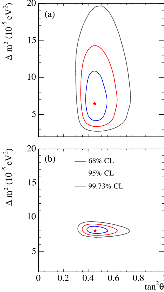
FIG. 35: (a) Global neutrino oscillation analysis using only solar neutrino data, and (b) including KamLAND 766 ton-year data. The solar neutrino data included SNO’s pure D 2 O phase day and night spectra, SNO’s salt phase extracted day and night CC spectra and ES and NC fluxes, the rate measurements from the CI, SAGE, Gallex/GNO, and SK-I zenith spectra. The 8 B flux was free in the fit; hep solar neutrinos were fixed at 9.3 \times 10^3 \text{ cm}^{-2} \text{ s}^{-1} . The stars are plotted at the best-fit parameters from the \chi^2 analysis, listed in Table XXVIII.
