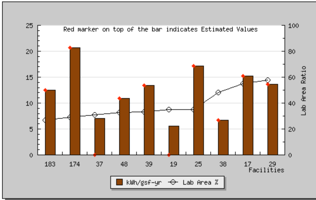
Figure 24. Plug load energy use intensity for a subset of buildings in the Labs21 database, with the following filters applied: lab type: biological, chemical, chemical/biological; occupancy hours: <=14 per typical workday
