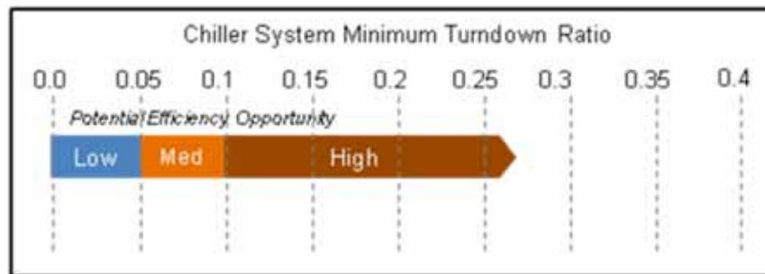
Figure 16. Benchmarks for chiller system minimum turndown ratio
