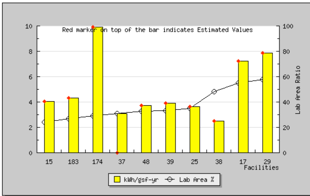
Figure 29. Lighting energy use intensity for a subset of buildings in the Labs21 database, with the following filters applied: lab type: biological, chemical, chemical/biological; occupancy hours: <=14 per typical workday
