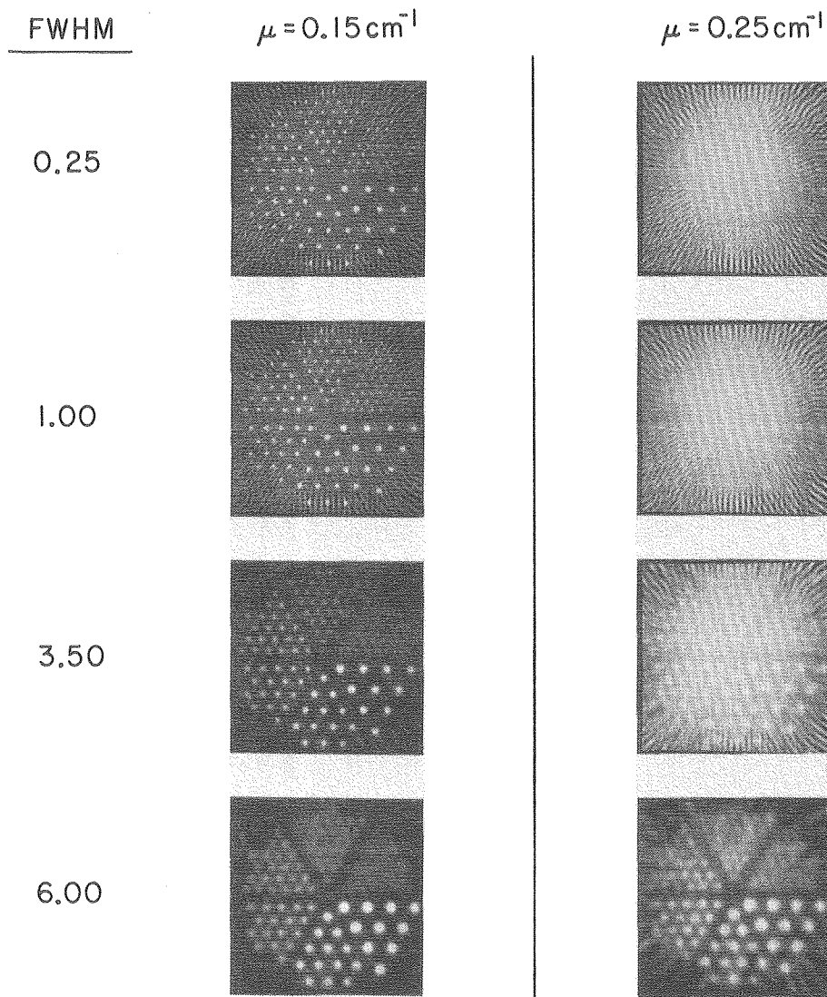
Fig. 9. Reconstructions of a 20-cm hot spot phantom. The pixel and projection bin sizes are 1.56 mm. The phantom was reconstructed by applying a GAUSS filter with FWHM = 0.25, 1.00, 3.50 and 6.00 projection bin widths to 180 projections equally sampled over 360°.
