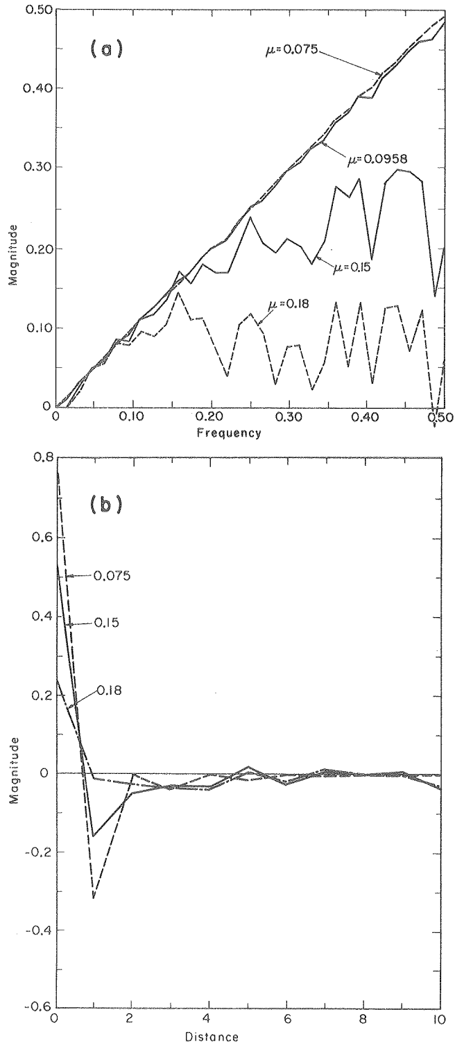
Fig. 3. Convolver in (b) evaluated by a least-squares fit of (23) for \mu = 0.075, 0.0958, 0.15, 0.18 (projection bin widths) -1 . The point response function h_{\mu} was determined by back-projecting over 360° using (3) and \mu = 0 , 360 equal projections of the Ramachandran and Lakshminarayanan convolver (36) into a 64 × 64 pixel array. In (a) are shown the filter functions that are the discrete Fourier transform of the convolvers in (b).
