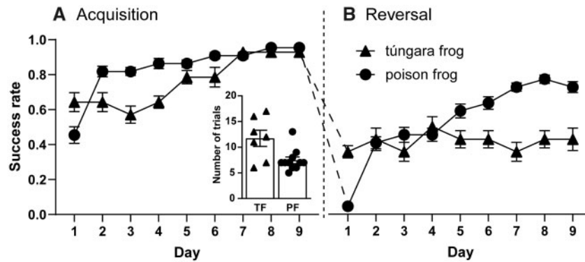
Fig. 2 Performance in a two-choice discrimination task when beacons and position cues were available (Experiment 1). During initial acquisition of the task (A), poison frogs had a steeper learning curve and reached the learning criterion earlier than túngara frogs (inset; t_{16} = 2.9 , P = 0.011 ). During reversal learning in which the reward contingencies were reversed compared to acquisition (B), poison frogs were able to learn the new association but túngara frogs were not (species \times day: F_{8,128} = 2.24 , P = 0.028 ). TF, túngara frog; PF, poison frog.
