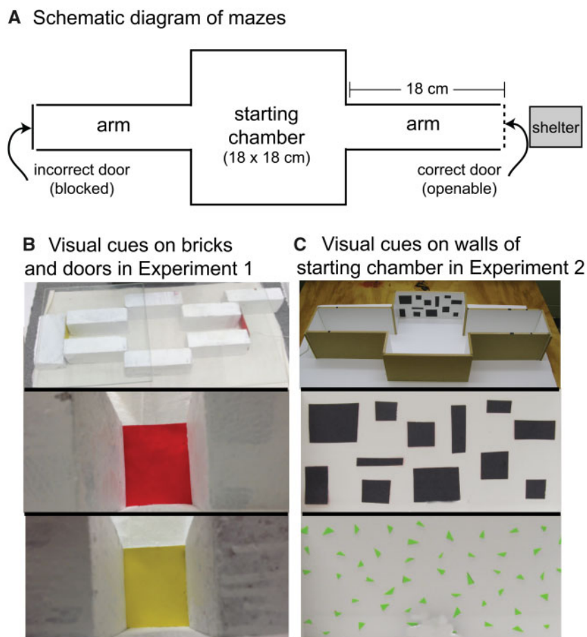
Fig. 1 Maze and cues used to test learning and flexibility in a two-option discrimination task. In the task, frogs were released in a starting chamber and could choose one of two arms to locate an exit leading to a shelter and return to the home cage ( A ). In Experiment 1, the maze was constructed of painted bricks and frogs could use cues on the bricks and/or on the doors leading out of the maze to choose the correct exit ( B ). In Experiment 2, the maze was constructed of uniform fiberboard and cues were only provided on the walls of the starting chamber ( C ).
