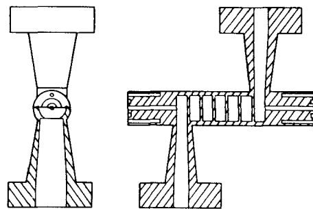
Fig. 6 The high-gradient accelerator test section drawings.
