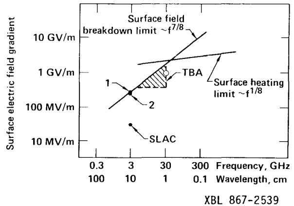
Fig. 5 Theoretical curves, two experimental points, and the operating point of SLAC showing the maximum expected surface field as a function of frequency. Point 1 is by Wang & Loew 24 and point 2 by Tanabe. 25
