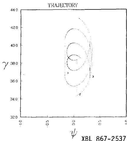
Fig. 3 This shows the actual phase space trajectory of an electron in a TBA. The trajectory begins at the top of the picture. The dashed vertical lines indicate when the electron passes through an induction linac. The numbers indicate the order of the jumps.
