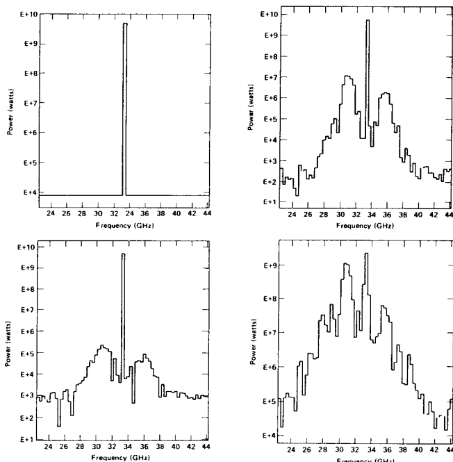
Fig. 4 A numerical simulation, by W. M. Fawley using the program GINGER, which shows the growth of sidebands in only going from 0 m (a) to 6.9 m (b) to 13.5 m (c) to 20.0 m (d) down a TBA. The parameters are those of Ref. 2.
