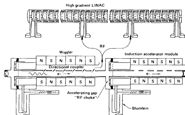
Fig. 1 Schematic of a two-beam accelerator that transfers energy from a high current low-energy beam to a low current high-gradient structure.
