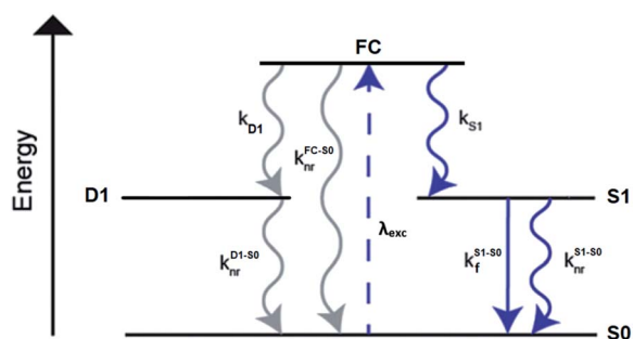
Fig. 14 General phenomenological model for \text{Ag}_N -DNAs. S0 and S1 represent the ground and emissive states, respectively, FC indicates the initially populated Franck-Condon state, and D1 is the dark state. The dashed blue line stands for the absorption process, wavy lines represent non-radiative pathways, and the straight line defines the emissive decay. Adapted from Cerretani, et al. , (ref. 185) with permission from the Royal Society of Chemistry.
