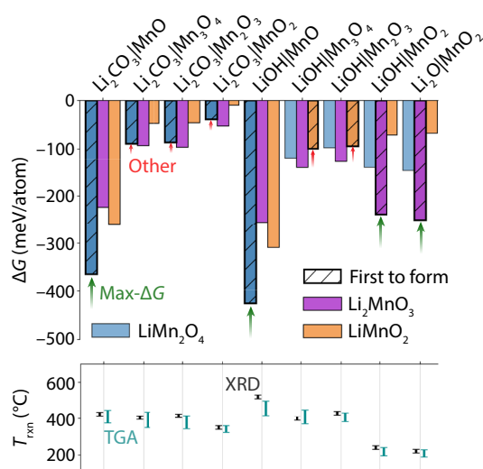
Fig. 3. Reaction selectivity in the Li-Mn-O space. The top panel shows the driving force ( \Delta G ) to form each ternary phase, represented by the bar heights corresponding to different reactant combinations. Each driving force was computed at the temperature where the starting materials began to react. These onset temperatures (bottom panel) were determined using in situ XRD (left, black) and TGA (right, cyan), whose uncertainties are represented by the range of each bar (see Methods). The first product observed in the reach reaction is denoted in the top panel by hashed bars with diagonal lines. In four cases, the first product to form is the one with the largest driving force (max- \Delta G ). The remaining five cases form products with a smaller driving force (other).
