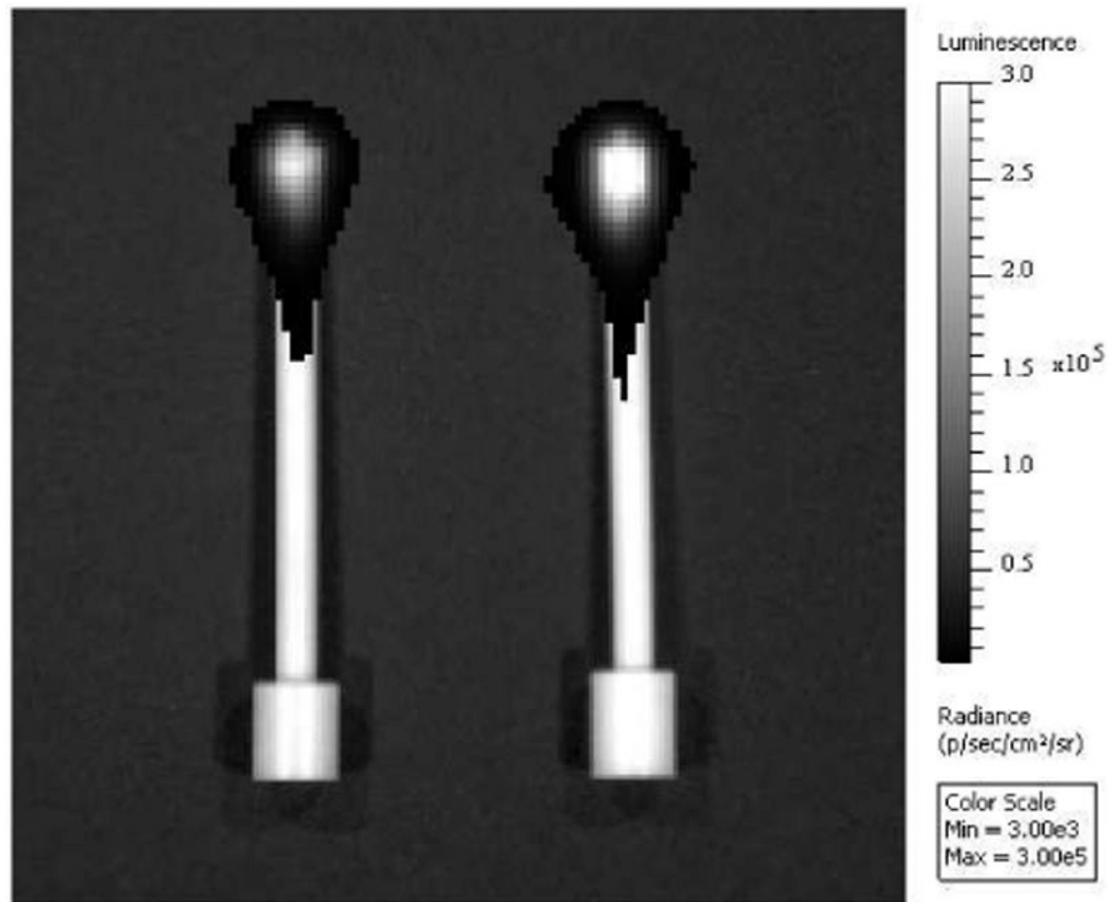
Figure 2. Inserts (of 50 mm length) with ^{90}\text{Y} activity, imaged in the optical system. The luminescence image (thresholded grey color scale) is overlaid on a photograph.
