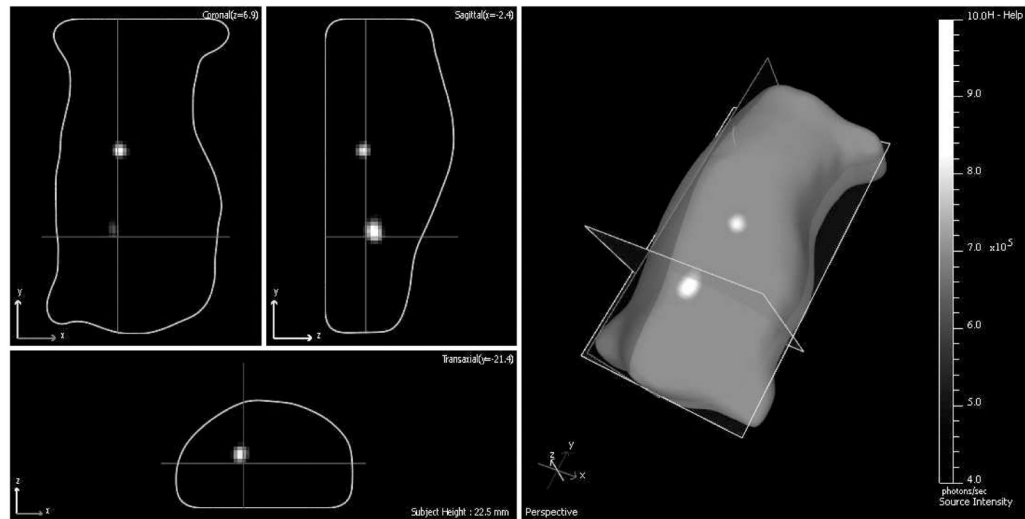
Figure 8. Sample display of tomographic reconstruction result from CLT data set. In this background-free case in a homogenous medium, the imaging is successful as the two insert targets are clearly reconstructed and resolved as individual sources. This shows the reconstruction from the first time point acquired, where the inserts each had 150 \mu\text{Ci } ^{90}\text{Y} .
