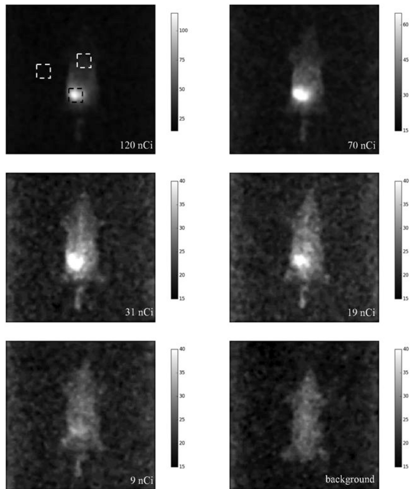
Figure 3. Sample single Cerenkov luminescence images from five timepoints, and an image of the phantom with no inserts. Each 120x120 pixel image is the raw luminescence image from a 2 min exposure, and has been background subtracted with a constant value (of 550 counts for all pixels), outlier pixels removed, and the image smoothed by a 3x3 pixel median filter. Three 10x10 pixel regions of interest (background, phantom background, target) are indicated on the first image. The colorscales represent counts per pixel and are thresholded at 15 counts. The activity per insert in the first five images (left to right, top to bottom) is 120, 70, 31, 19, and 9 nCi. The afterglow of the plastic material, even with minimized handling in room light, is apparent in the background image.
