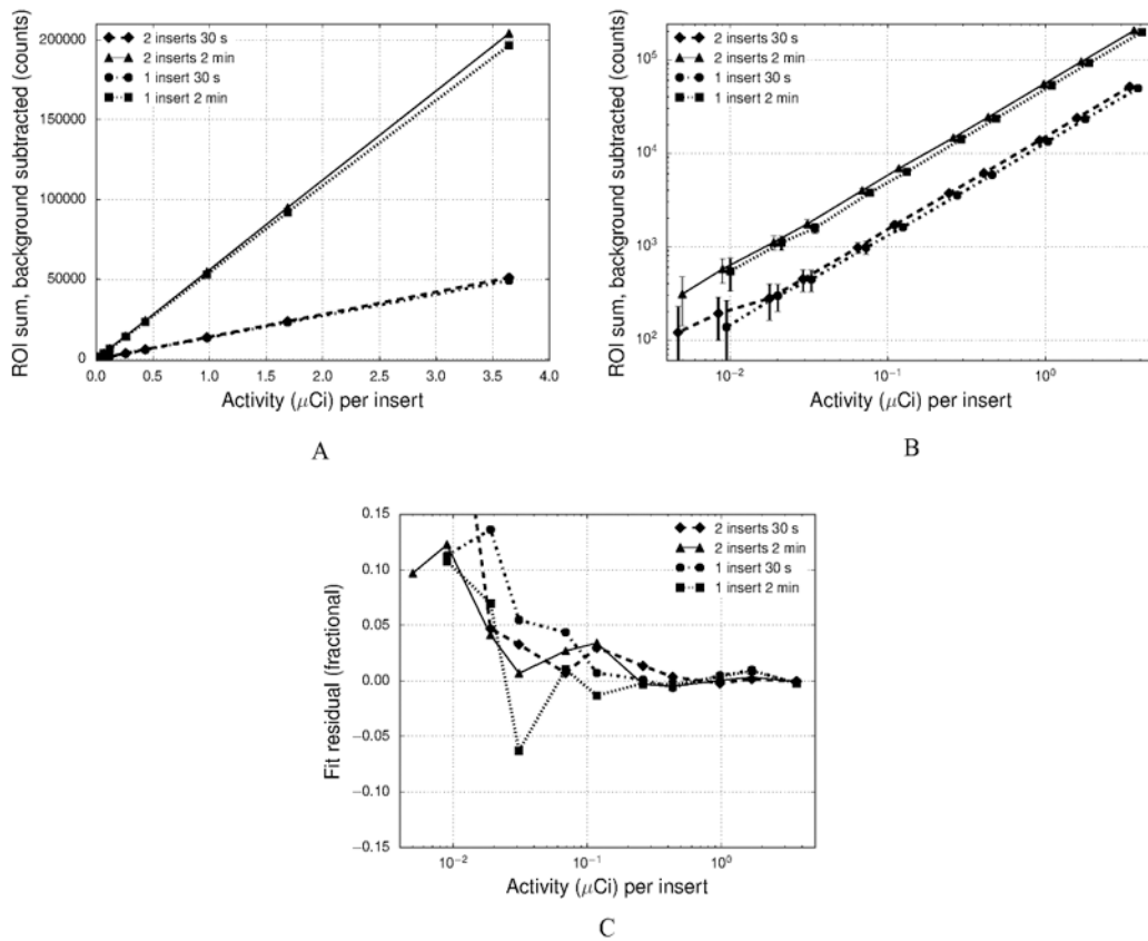
Figure 6. CLI background subtracted ROI values versus activity (A linear scale; B log-log scale, points slightly staggered for visibility), and residuals from a linear fit (C). The fits are not shown on the plots since they are indistinguishable from the data except for the lowest activity points. The fits are forced to go through the origin (i.e. fits are single parameter fits to lines of the form y=kx ). For the quantitative imaging limit definition used here of linearity within a fractional difference of 0.05 (i.e. 5%), the result here is 0.1 \mu\text{Ci} per insert.
