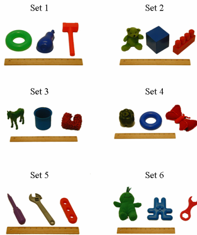
Figure 2: Objects used in the parent-child joint interaction study. The ruler shown in each set is 12'' in length.
