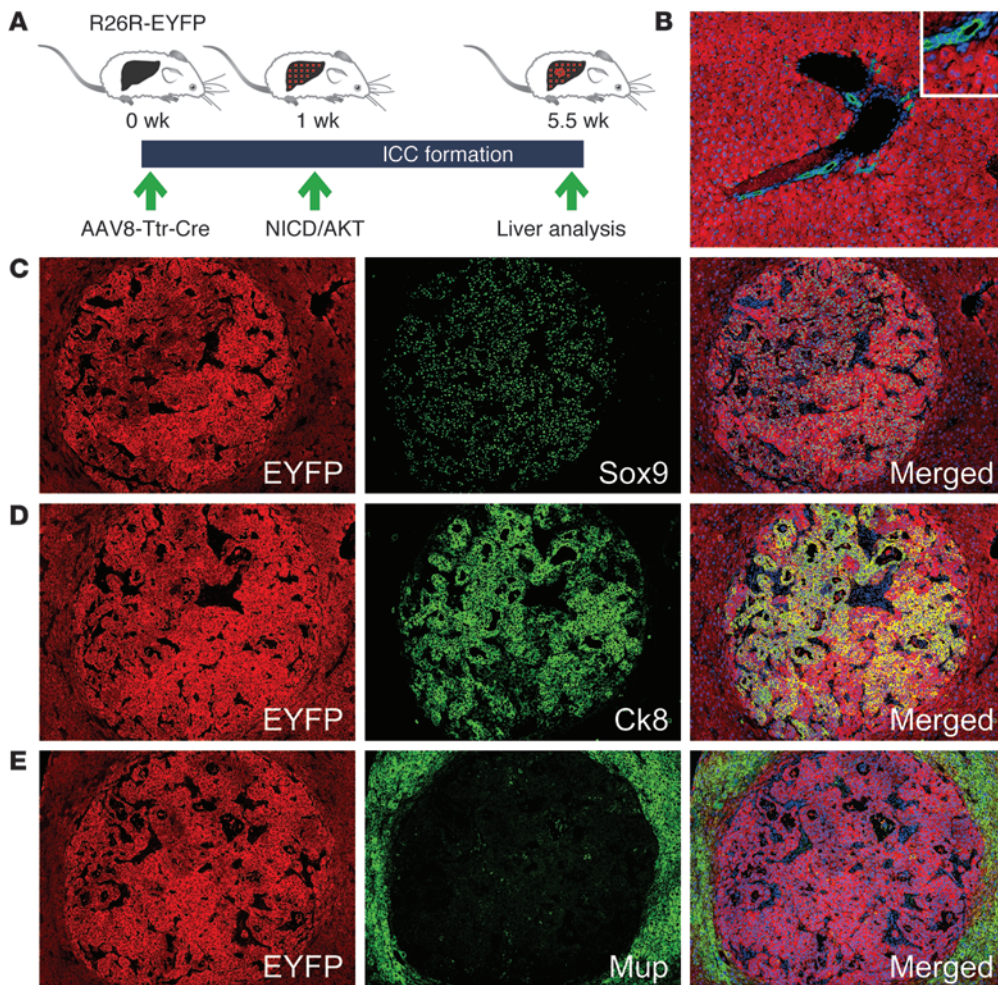
Figure 2 Hepatocyte origin of NICD/ AKT-induced ICCs. (A) R26R-EYFP mice were intravenously injected with 4 \times 10^{11} viral genomes of AAV8-Ttr-Cre, followed by hydrodynamic tail vein injection of the NICD/AKT plasmids 1 week later. Tumors were analyzed 4.5 weeks after plasmid injection. (B) Coimmunostaining for EYFP (red) and Ck19 (green) 1 week after AAV8-Ttr-Cre injection shows that all hepatocytes, but no BECs, express EYFP. (C–E) Immunostainings of tumors for EYFP (red) show that they originated from hepatocytes. Additional immunostainings (all green) for Sox9 (C) , Ck8 (D) , and Mup (E) show that tumors express biliary markers but lack hepatocyte differentiation. Nuclei were stained with DAPI (blue). Original magnification, \times 100 ; inset, \times 200 . At least 15 liver sections from 3 mice were analyzed for each immunostaining.
