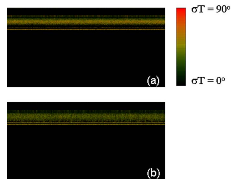
Fig. 2 Doppler variance images of the blood at HCT=40% for (a) normal and (b) dextran-treated blood. The axial axis represents scan depth (0 to 3.6 mm) and the horizontal axis represents 2000 A-lines.
