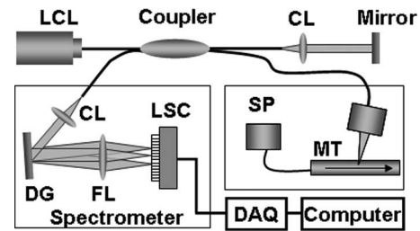
Fig. 1 Schematic diagram of the SDODT. Incident light was inclined by 5 deg from the vertical. CL, collimating lens; DG, diffraction grating; FL; focusing lens; LCL, low coherent light; LSC, line scan camera; MT, microtube; SP, syringe pump; DAQ, data acquisition.
