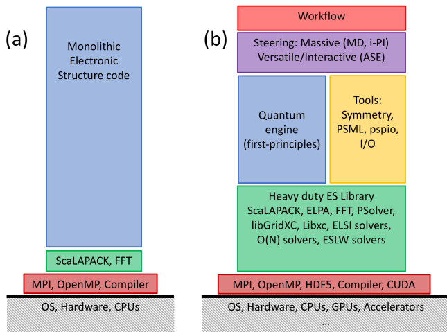
FIG. 1. Comparison of the traditional monolithic and the emerging modular paradigms in electronic structure coding. The acronyms in the figure indicate operating system (OS), fast Fourier transforms (FFT), input/output (I/O), molecular dynamics (MD), and linear scaling with the number of atoms, \mathcal{O}(N) , respectively, in addition to the central and graphical processing units, CPU and GPU, respectively. Steering upper-level drivers are distinguished between versatile toolkits such as ASE, and handlers of massive amounts of quantum-engine replicas, such as i-PI. In addition to the well-known MPI, OpenMP, CUDA, and HDF libraries, other acronyms and names relate to libraries described in Sections I, II, and IV.
