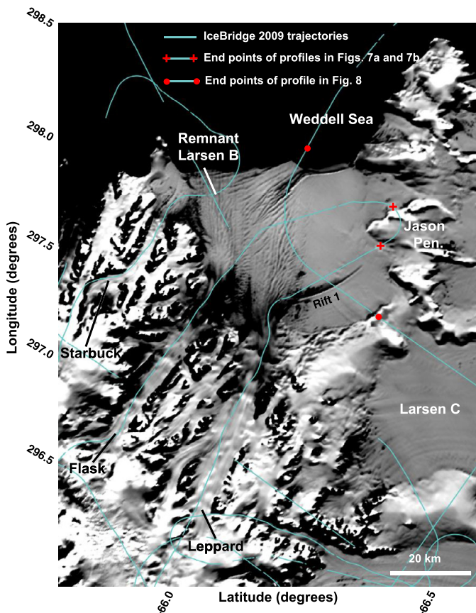
Fig. 6. The study area from the 2008–2009 MODIS Mosaic of Antarctica (MOA; Haran et al., 2014 ) showing the increased presence of fracture features compared with the 2003–2004 MOA image in Fig. 1 , in particular the widening and propagation of Rift 1.
