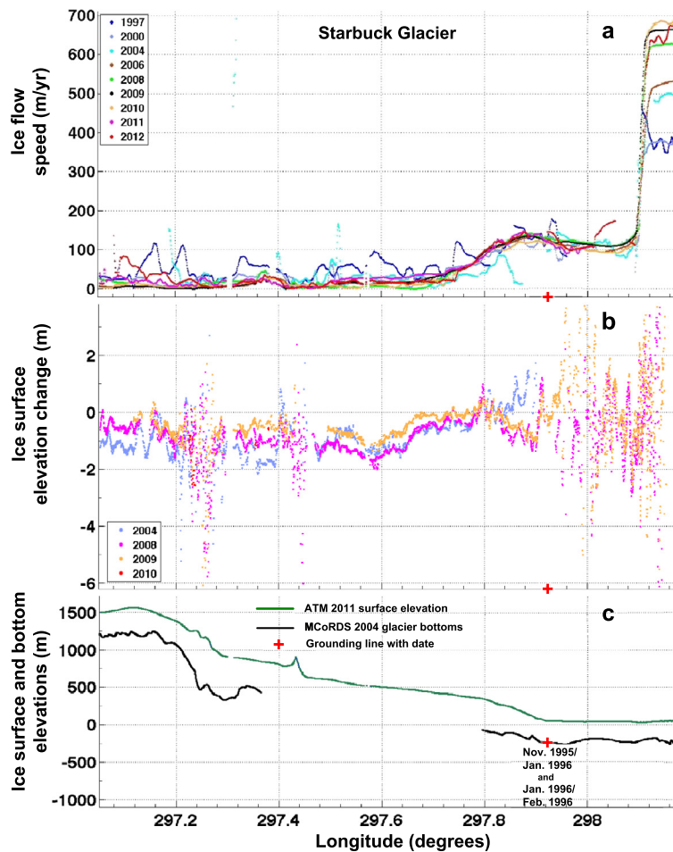
Fig. 4. Starbuck Glacier (a) InSAR surface flow speeds from 1997 to 2012 along the same ATM flight path shown in Fig. 1a. (b) Surface elevation changes from the grounding line to an altitude of ~1500 m above the WGS84 ellipsoid along the trajectory shown in Fig. 1a. Data show the elevation difference for each year in the legend relative to year 2011 (Starbuck was not surveyed in year 2011). (c) The surface elevation profile in year 2011 as measured by ATM along the flight path in Fig. 1a, and the corresponding MCoRDS depth-sounding radar glacier bed profile of the glacier. The MCoRDS soundings are from the 2004 IceBridge campaign. Both surface and bed elevations are relative to the WGS84 ellipsoid. In all panels, the red crosses mark grounding line locations as found by Rignot et al. (2011b).
