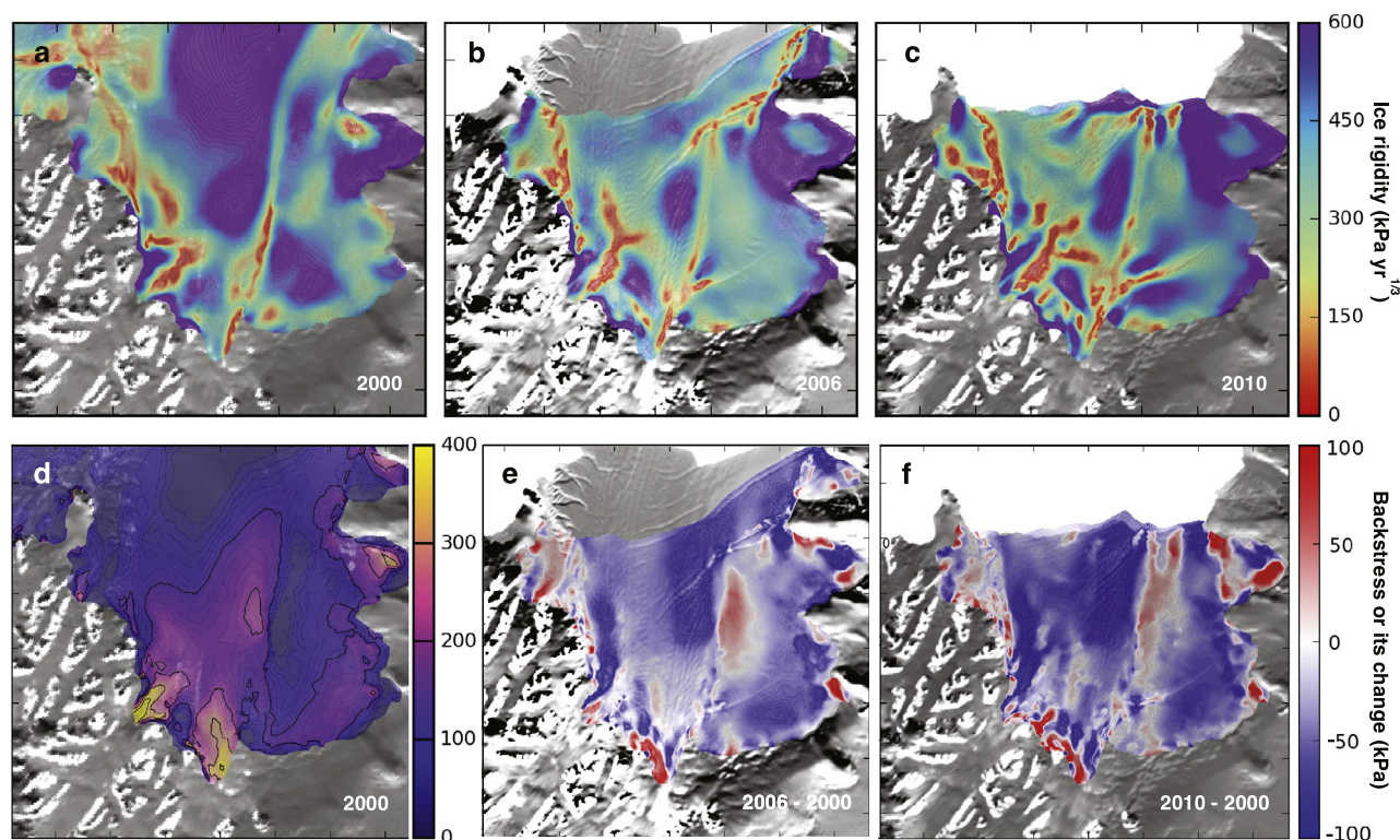
Fig. 5. The modeled rheology field in the area of the remnant LBI shelf revealing changes in the spatial pattern of ice rigidity among the three years shown. (a) Year 2000 before the disintegration of the ice shelf. (b) Year 2006 in the remnant LBI shelf after the 2002 collapse. (c) Year 2010 after further retreat of the remnant LBI shelf front. Background images in the panels are from (a) MODIS on 31 January 2002, (b) the 2003–2004 MODIS Mosaic of Antarctica (MOA; Haran et al., 2005), and (c) the 2008–2009 MOA (Haran et al., 2014). (d) The modeled spatial patterns of backstress in Year 2000. (e) The change in backstress: backstress in year 2000 subtracted from that of year 2006. (f) Backstress in year 2000 subtracted from that of 2010.
