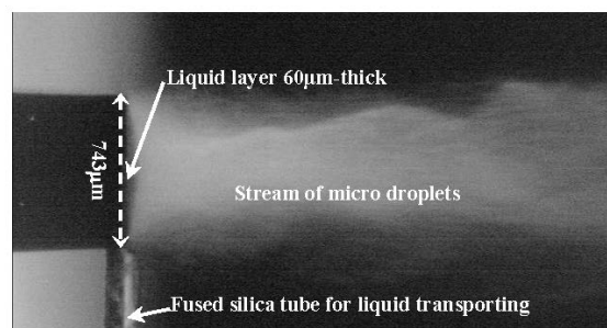
Figure 7. Droplet ejection from a 60 \mu\text{m} -water layer on the end face ( 743 \mu\text{m} \times 800 \mu\text{m} ) of a 2.0 MHz 4-Fourier horn nozzle at 200 \mu\text{L}/\text{min} output rate and 0.15 W electrical drive power.
