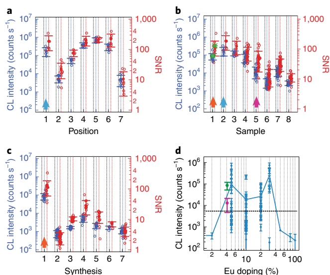
Fig. 3 | Variability of CL brightness and SNR. In all experiments, \text{NaGdF}_4:5\% \text{Eu}^{3+} nanoparticles were \text{BF}_4^- -exchanged and spin-coated on a Si substrate. a–c , CL variability and SNR are shown in a for the same sample (sample 2 in b ) of the brightest synthesis run (synthesis 1 in c ), in b for synthesis 1 but for a different sample preparation, and in c across different synthesis runs. Identical samples are marked with two blue arrows in a and b and with two orange arrows in b and c . The data used in Fig. 1c are highlighted in b with green stars and in d with a green data point (sample average). The data from Fig. 2 are highlighted with a magenta arrow in b and a magenta data point in d . Open circles represent the brightness (Gaussian amplitude) in counts per second (blue, left y axis) and the respective CL SNR (red, right y axis) for individual nanoparticles. Filled circles represent the corresponding average values. d , Average single nanoparticle brightness (each point represents a 1 \mu\text{m}^2 field of view) as a function of \text{Eu}^{3+} doping. Green and magenta data points represent data used in Fig. 1c and Fig. 2 (data points are offset to the left for visibility and correspond to 5\% \text{Eu}^{3+} ). The data include all measured samples (including different syntheses, different samples but the same synthesis, and different regions of the same sample). The solid blue line represents an average of intensities for each \text{Eu}^{3+} doping. The black horizontal dashed line represents the average noise level from a–c ( 5,449 \text{ counts s}^{-1} ) to illustrate the marginal CL intensity. All error bars correspond to one standard deviation.
