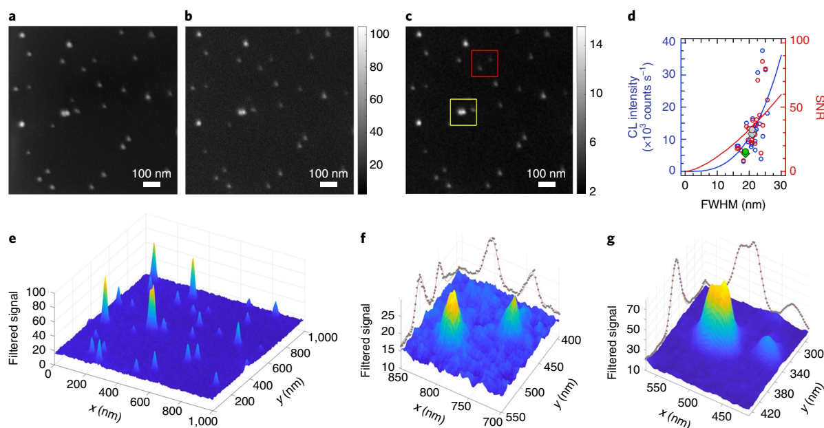
Fig. 2 | CL imaging of single NaGdF 4 :5% Eu 3+ . The nanoparticles were BF 4 -exchanged and spin-coated on a Si substrate. a,b , Raw SE image ( a ) and corresponding CL signal (detected photons) ( b ). Images have an area of 1 μm 2 , the pixel pitch is 1.95 nm, the beam energy is 5 keV, the pixel dwell time is 2 ms (8 min 44 s image acquisition time) and the beam current is ~400 pA. c , Fourier-filtered CL image of b using a Gaussian smoothing function of \sigma = 7.16 nm. d , CL intensity (blue, left axis) and CL SNR (red, right axis) for all the single nanoparticles from a and b , plotted as a function of the nanoparticle SEM FWHM ( 2.35\sigma ) of the 2D Gaussian distribution fitted to each nanoparticle CL signal. (Note that the TEM diameter ( 13.9 \pm 5.0 nm) is a more accurate measurement of the particle diameter than SEM, which can be skewed by charging and contamination; see Fig. 1b and Supplementary Fig. 4 for TEM data.) e , 3D representation of c . f,g , Images of the zoomed-in red ( f ) and yellow ( g ) regions in c . The data points for the nanoparticles in f are highlighted with diamonds (CL signal) and circles (CL SNR) in d . Grey corresponds to the brighter and green to the dimmer nanoparticle. A doublet of nanoparticles is shown in g . The dotted points on the sides of f and g correspond to a maximum intensity projection of the filtered CL signal. The red lines represent a guide to the eye (Gaussian fit).
