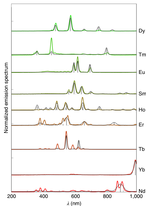
Fig. 4 | Multicolour imaging of lanthanide-based nanoprobcs. a , Emission spectra of ensemble samples of n -hexane-washed \text{NaGdF}_4 (solid coloured lines) nanoparticles doped with different lanthanide ions ( 20\% doping for \text{Er}^{3+} ; 15\% doping for the others) dropcast on a Si substrate. The data were acquired at 5 \text{ keV} electron beam energy and corrected for spectrometer efficiency. Grey bars correspond to the Judd–Ofelt calculations (see Methods section ‘Simulations of nanoparticle spectra’ and Supplementary Fig. 31). Grey lines correspond to fitted spectra using linewidth as the only fitting parameter.
