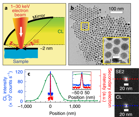
Fig. 1 | CL microscopy concept. a , Illustration of a CL instrument that uses an electron beam to induce emission of photons by nanoparticles (shown in b ). CL emission is collected by a parabolic aluminium mirror and focused onto a photon-counting photomultiplier module. b , TEM image of NaGdF 4 :5% Eu 3+ nanoparticles. Inset, Magnified version of the region highlighted with a yellow square. c , Simultaneous SEM and CL imaging of the particle highlighted with green stars in Fig. 3b. Cross-sectional line profiles of SE (red, right axis) and CL (blue, left axis) scans of a single BF 4 - -exchanged NaGdF 4 :5% Eu 3+ nanoparticle spin-coated on the Si substrate, imaged in parallel. The pixel pitch is 1.95 nm, the beam energy is 5 keV, the pixel dwell time is 2 ms and the beam current is ~400 pA. A cross-sectional line profile of a confocal light microscopy scan of a NaYF 4 :18% Yb 3+ , 2% Er 3+ nanoparticle of similar size is shown in green (left axis). The excitation wavelength is 980 nm, and a water immersion objective with 1.27 numerical aperture is used. Inset, The same data, but with a zoomed-in x axis. Raw SE and CL data are shown on the right. All cross-sectional line profiles are fitted to a single-Gaussian model.
