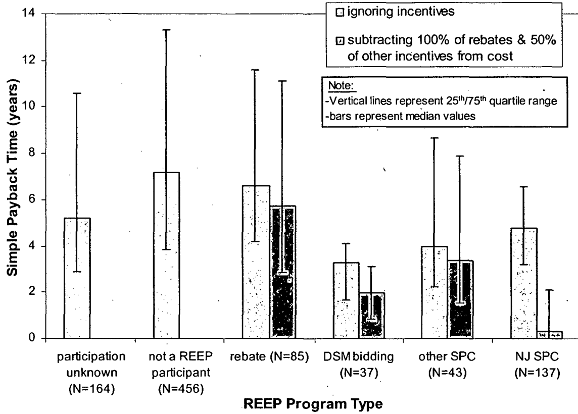
Figure 5-5. Impact of Ratepayer-Funded Energy-Efficiency Program Incentives on SPT
