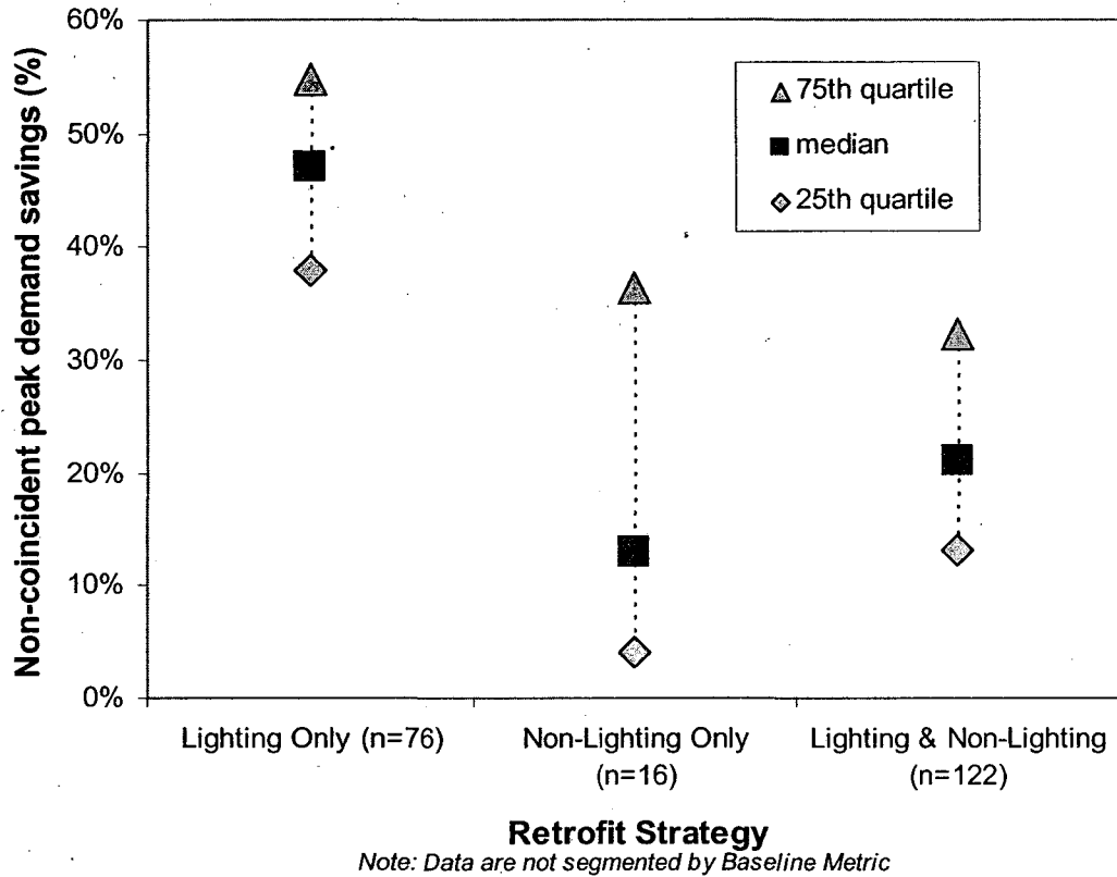
Figure 4-4. Non-Coincident Peak Demand Savings (%)
