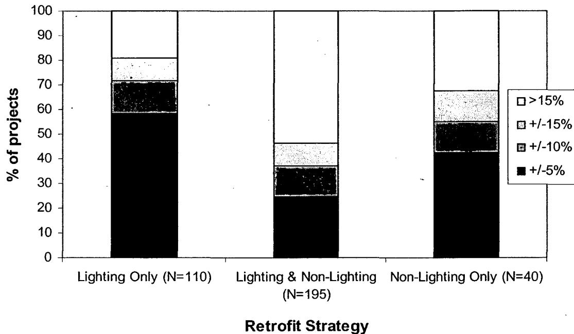
Figure 4-7. Difference Between Predicted and Actual Savings by Retrofit Strategy
