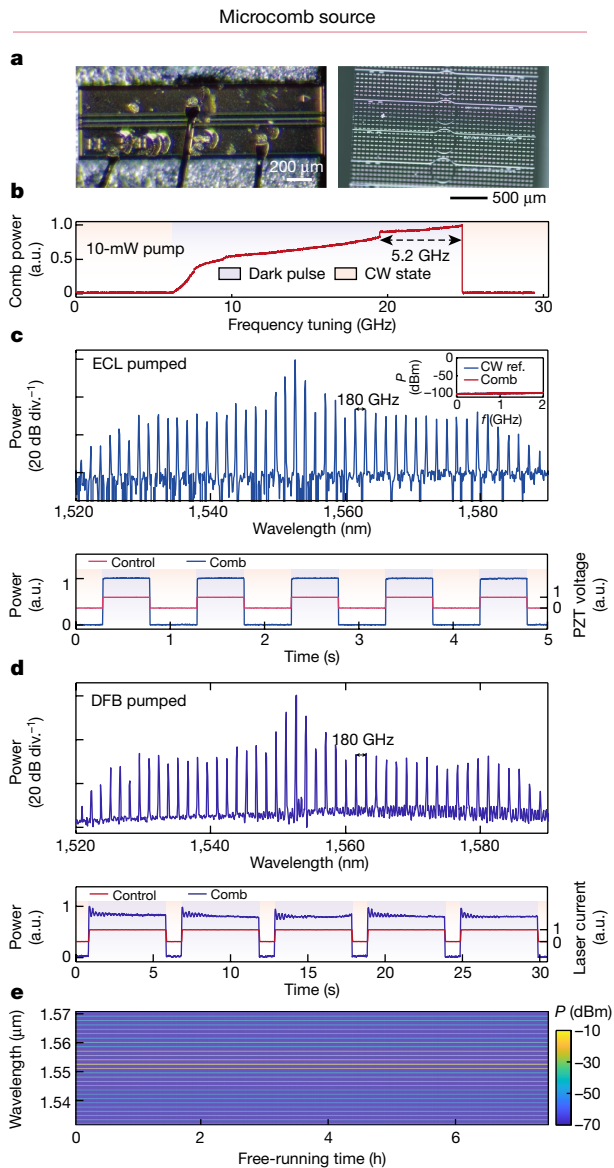
Fig. 2 | Comb generation and fundamental characteristics. a , Optical image of the InP DFB laser chip and the AlGaAsOI microresonators for dark-pulse generation. b , Normalized comb power when tuning the pump frequency across the resonance at around 1,552 nm. With 10-mW pump power, a dark-pulse Kerr comb could be accessed in a large frequency window (tens of gigahertz). CW, continuous wave. c, d , Two-FSR dark-pulse spectra (top) and the ‘turnkey’ behaviours (bottom) pumped by a commercial external laser ( c ) or a DFB laser chip ( d ) with an equal on-chip power of 10 mW. A pair of flat wings besides the pump is formed in both spectra, exhibiting typical profile of
