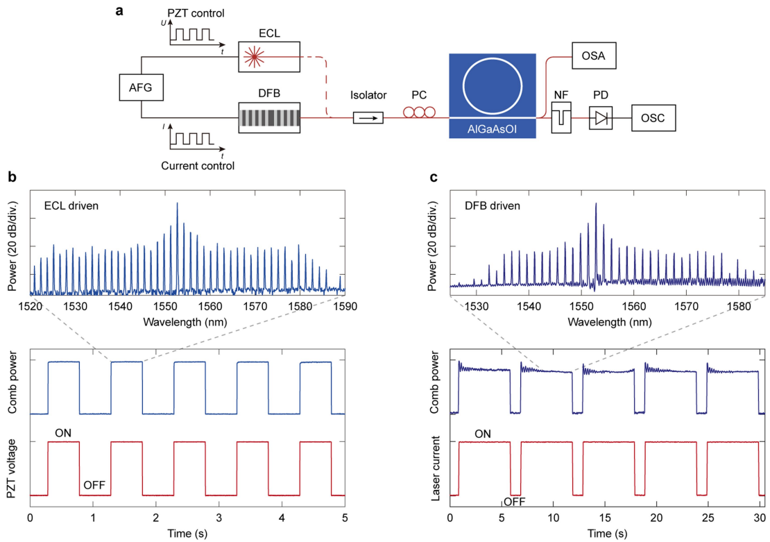
Extended Data Fig. 2 | Turnkey AlGaAs dark-pulse microcomb generation. a , Experimental setup. b , ECL and c , DFB laser chip driven comb spectra and the comb power variations along with the control signal in five consecutive switching tests.
