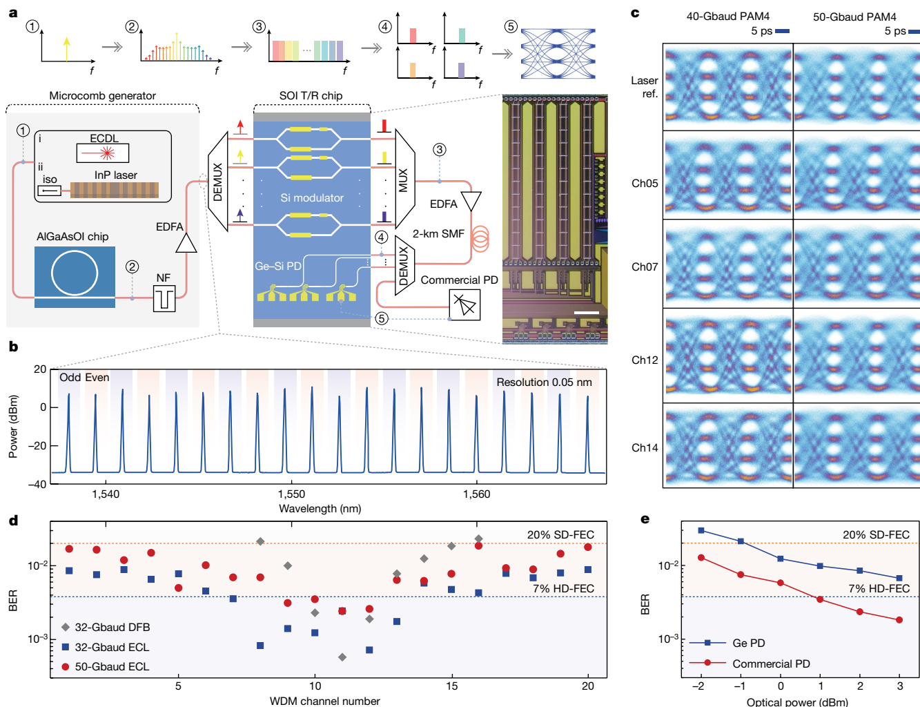
Fig. 3 | Transmission results. a , Schematic of the microcomb-based data transmission set-up. The dark-pulse Kerr comb source is pumped by a continuous-wave laser, which can be generated by a commercial external cavity diode laser (ECDL, i) or a distributed feedback laser chip (ii). The generated comb is then sent into a SiPh T/R chip. iso, isolator; NF, notch filter; DEMUX, demultiplexer; MUX, multiplexer. Scale bar, 500 \mu\text{m} . b , A 20-line comb spectrum in the C band as the multiwavelength source before injection into the SiPh T/R chip. c , Typical eye diagrams of the chosen channel after modulation by SiPh modulators at different symbol rates (32 Gbaud, 40 Gbaud and 50 Gbaud). d , BER for each comb line. The blue squares and red circles indicate the ECL-pumped comb data transmission results at symbol rates of 32 Gbaud
