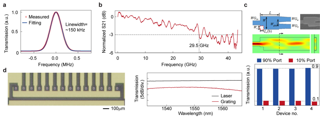
Extended Data Fig. 1 | Performance of building block devices. a, Measured linewidth of the DFB laser. b, The measured 3dB bandwidth of the Si-Ge PD photodiode. c, Design, fabrication and measurement results of the 10:90
