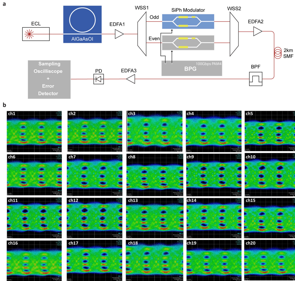
Extended Data Fig. 3 | Detailed information for data transmission. a, Detailed experimental set-up for the odd/even test band for the comb-based silicon photonics data link. b, measured 100 Gbps PAM-4 eye diagrams from the sampling oscilloscope for each channel at receiving end.
