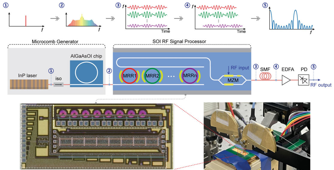
Extended Data Fig. 5 | Dispersive delay-line MPF. Experimental setup of the second dispersive delay-line scheme based TDL-MPF.
