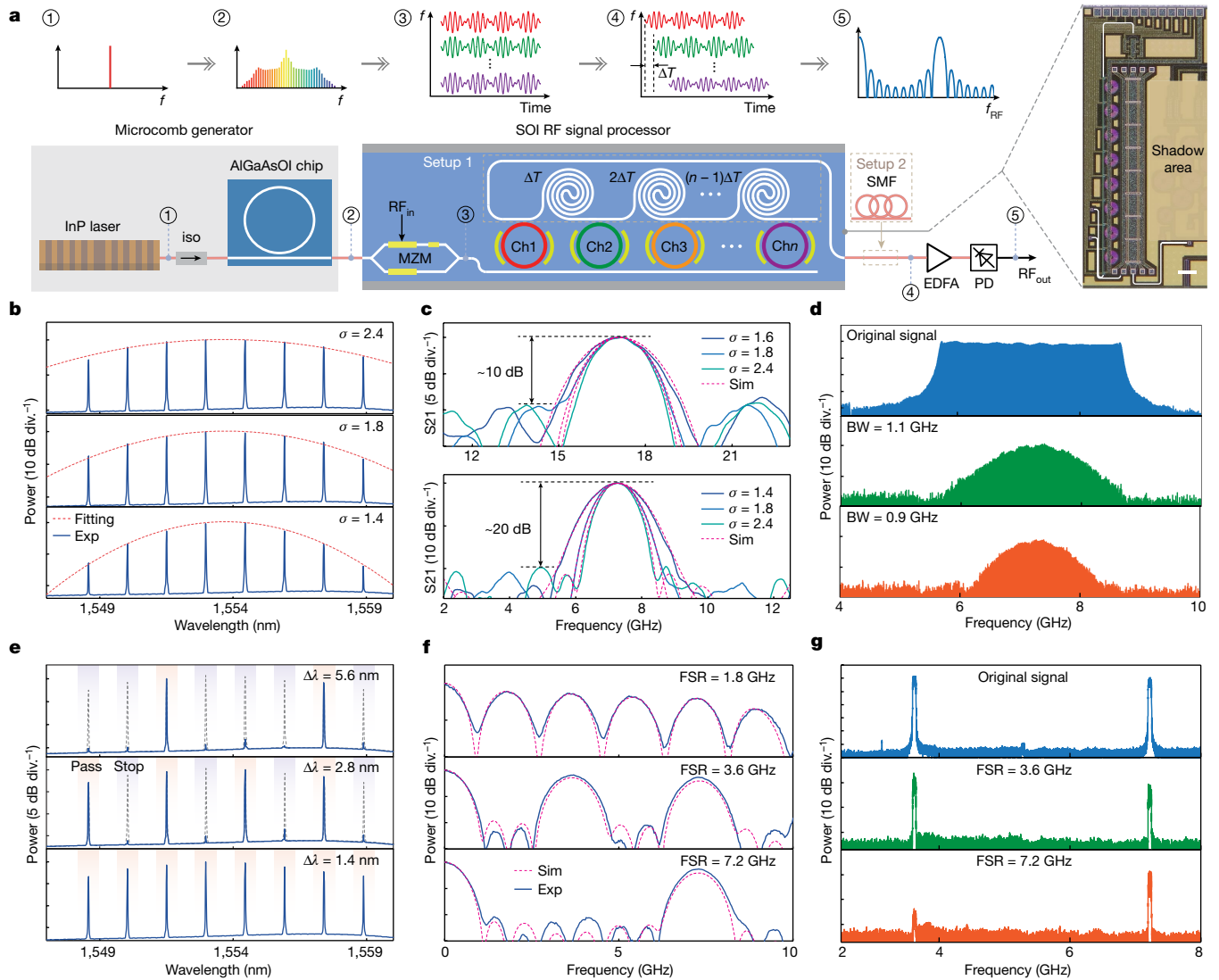
Fig. 4 | Reconfigurable MPF results. a , Schematic of the setup to perform microcomb-based reconfigurable MPF. The time delays between comb lines are produced by on-chip spiral delay lines (setup 1) and dispersive propagation from a spool of SMF (setup 2). Scale bar, 200 \mu\text{m} . b , Optical spectra of Gaussian-apodization comb lines for BW programming ( \sigma , Gaussian factor; blue, experiment (Exp); red, Gaussian fitting). c , RF filtering responses of the MPF with various passband BWs, based on the setup 1 (top) and setup 2 (bottom). The red dashed curves show the theoretical fitting results (Sim.) (Supplementary Note III). d , Proof-of-concept demonstration of RF filtering of
