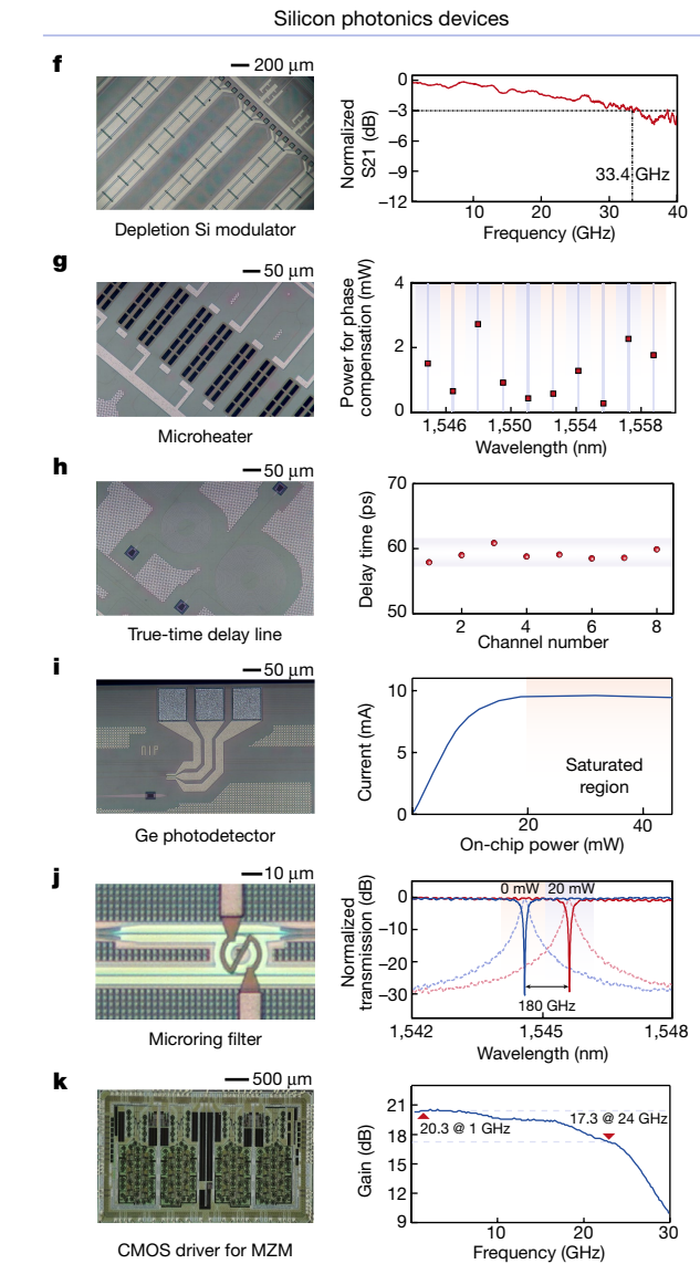
the coherent dark-pulse microcombs. Inset: comb intensity noise (resolution BW of 100 kHz). The intensity noise of the dark-pulse Kerr comb is at the same power level as the electrical spectrum analyzer background. P, power; f, frequency; PZT, lead zirconate titanate. e , Long-term stability of a free-running comb. f–k , Optical images and main performance of several Si-based fundamental devices, including a depletion-mode Si MZM ( f ), a TiN microheater ( g ), a Si spiral waveguide delay line ( h ), a vertical epitaxial Ge PD ( i ), a microring filter ( j ) and a CMOS driver for MZMs ( k ). More details can be found in Methods.
