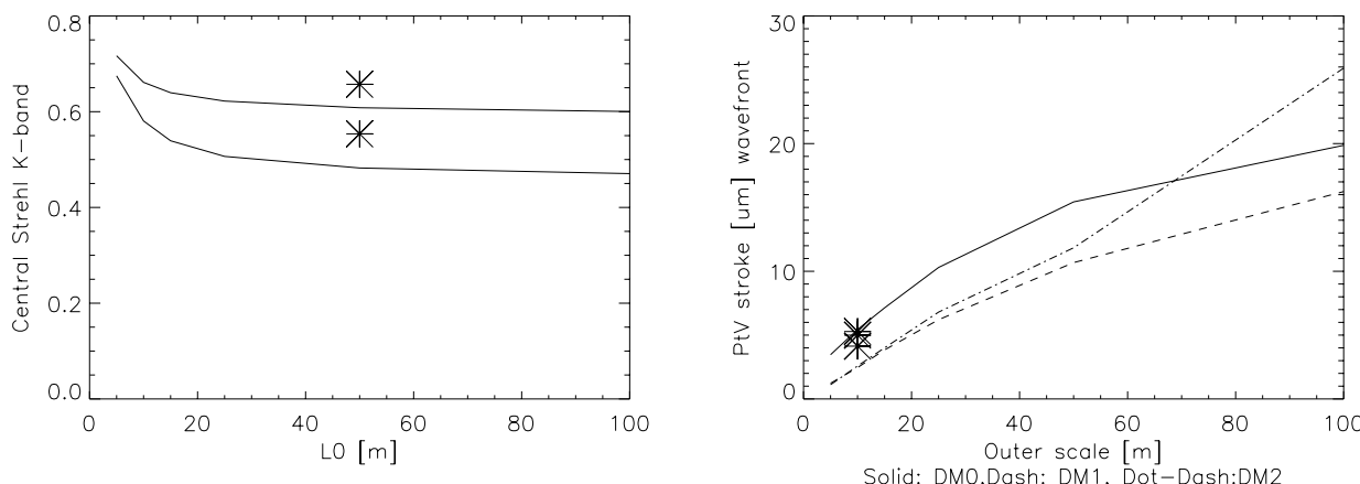
Figure 10: On the left, MCAO performance (on-axis on top, and median of field at the bottom) as a function of outer scale. The Stars represent the cases with the L_0(h) profile of Figure 11. The lines are for L_0(h) = \text{constant} (represented on the X axis). On the right, the peak-to valley stroke (wavefront) over the whole mirror (tip-tilt included) for the different cases (PtV stroke was measured by simply taking the min-max of the DM surface).
