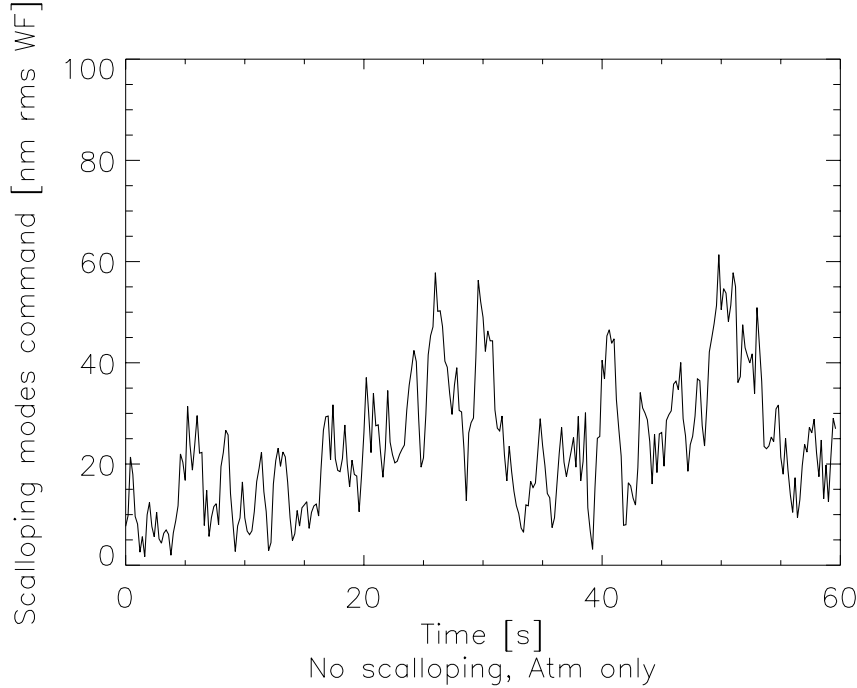
Figure 8: Scalloping coefficient (residual) as a function of time, when there is no scalloping initially.
