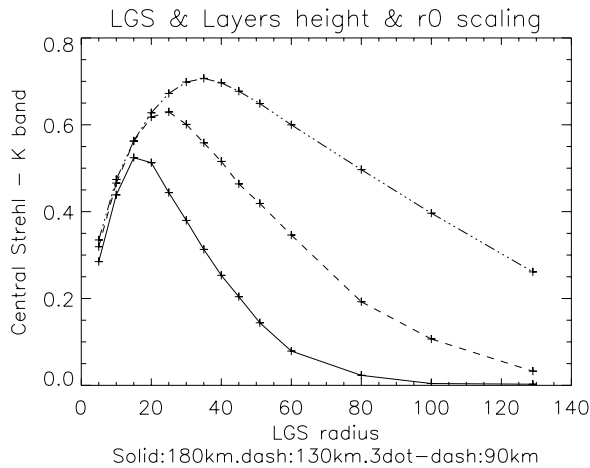
Figure 12: LTAO performance for 3 different zenith angles (0, 30 and 60 degrees). The corresponding LGS heights are at 90km, 130km and 180km, respectively.
