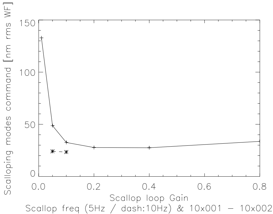
Figure 6: Scalping residuals (averaged between t=10s to t=60s ) as a function of scalping loop gain. The solid curve is for 5Hz, the dashed on for 10Hz.
