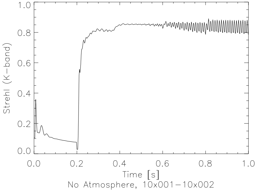
Figure 7: AO closed loop, with the default amount of input scalloping, when there is no atmosphere. This is the Short exposure Strehl
