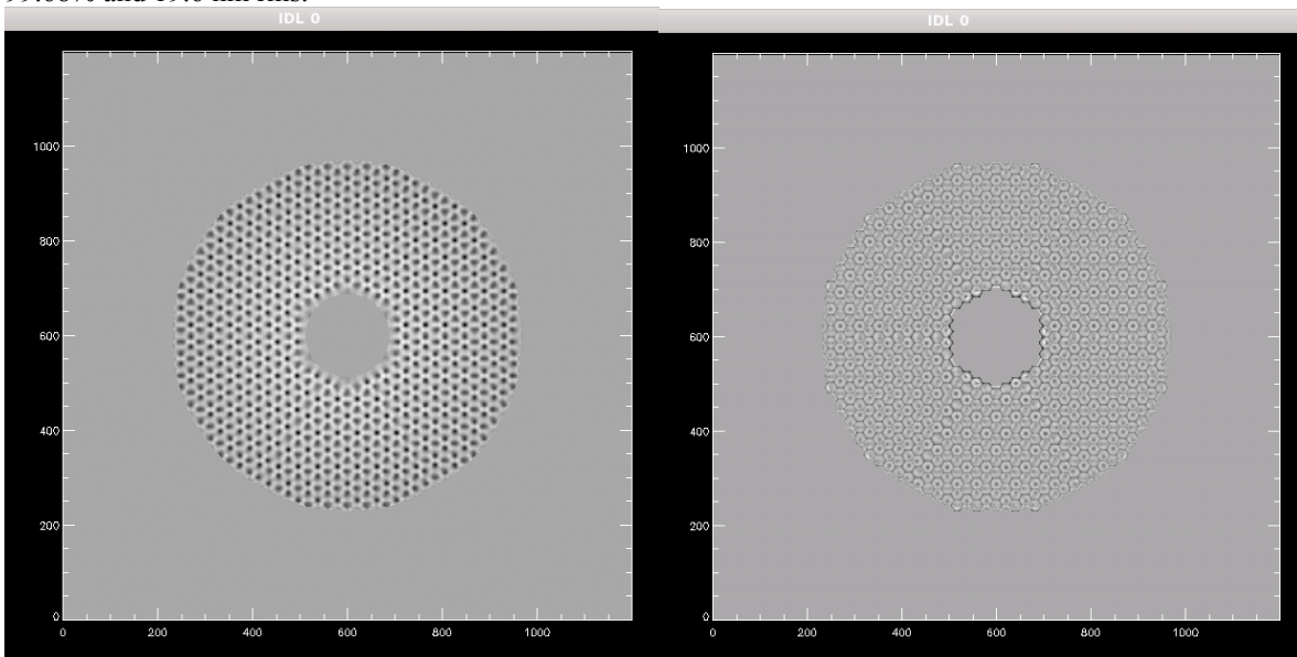
Figure 2: DM shape (on the left) and residual phase after fitting by the M4 (right), for screen002.
