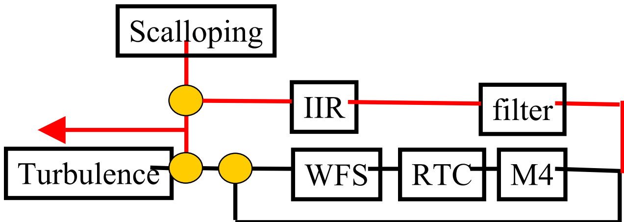
Figure 3: Schematic representation of the scalloping loop. The grey lines are the AO loop, the red lines the scalloping part. The red arrow represents the tap point for the scalloping residuals.
