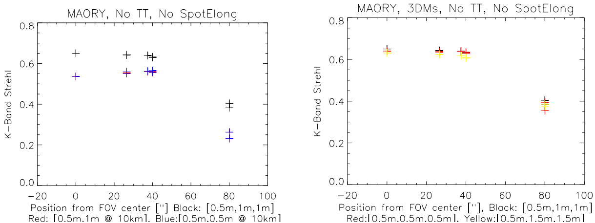
Figure 9: MCAO number of DMs & pitch. On the left, Number of DMs & pitch. On the right, for 3 DMs, impact of the pitch of the DMs.
