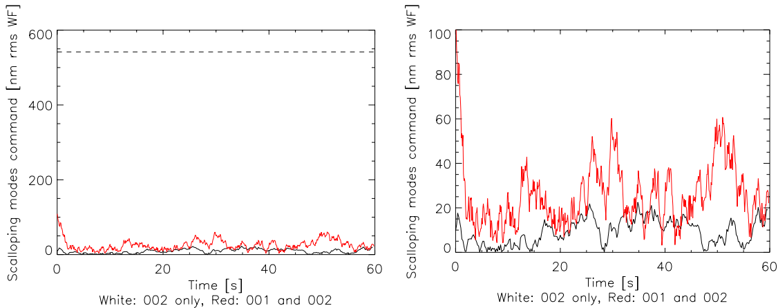
Figure 5: Scalloping residuals as a function of time (in nm rms). The dashed line shows the original input value. Black line is when only 10^*002 is sent at the beginning and only mode 002 is corrected (other mode has a gain of zero). The red curve is when 10^*001 - 10^*002 is introduced and both modes corrected. On the right, is a zoom of the same curve as on the left.
