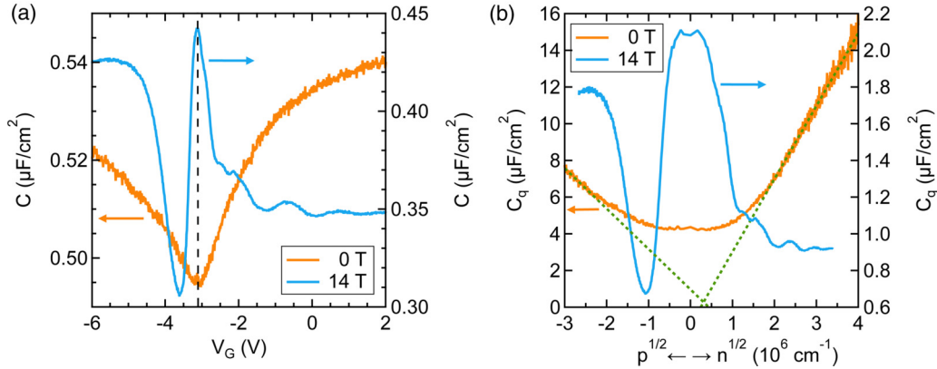
FIG. 5. C - V characteristics. (a) Capacitance of sample A measured as a function of gate voltage with and without an applied magnetic field of 14 T. (b) Quantum capacitance extracted from the data shown in (a), as a function of the square root of the modulated carrier density. The dotted lines are a fit to the data at zero magnetic field.
