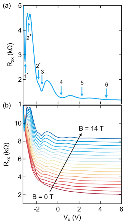
FIG. 3. SdH oscillations as a function of V_g for sample A. (a) R_{xx} as a function of V_g at 14 T. Landau level indices of the minima are indicated. (b) Magnetic field behavior of the SdH oscillations, offset for clarity. Data were symmetrized using the relation [R_{xx}(B) + R_{xx}(-B)]/2 .
