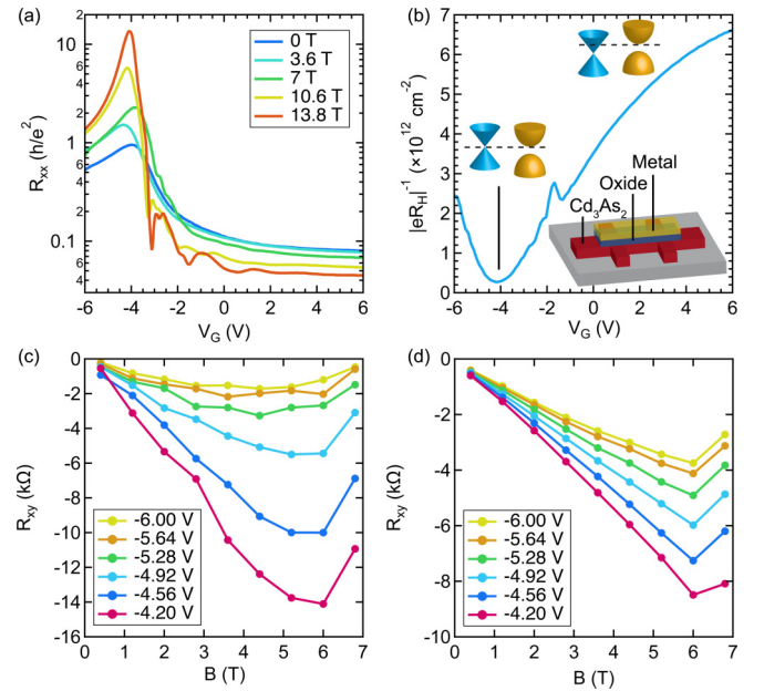
FIG. 2. Magnetotransport behavior of the gated devices. (a) R_{xx} of sample A as a function of gate bias ( V_{\text{g}} ) for different magnetic fields. (b) |eR_{\text{H}}|^{-1} extracted from the low-field Hall effect as a function of V_{\text{g}} for sample A. (c) and (d) R_{xy} of samples A and B, respectively, as a function of the magnetic field, for large negative values of V_{\text{g}} (Fermi level below the CNP of the two-dimensional states). Data were anti-symmetrized using the relation [R_{xy}(B) - R_{xy}(-B)]/2 , to suppress contributions from the noise and intermixing of R_{xx} and R_{xy} signals. The inset in (b) shows a schematic of the gated Hall bar structure (bottom) and sketches that illustrate the tuning of the Fermi level (dashed line) with respect to the two-dimensional states (blue) at different V_{\text{g}} . Bulk states are shown in gold.
