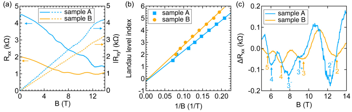
FIG. 1. Magnetoresistance and quantum Hall effect of samples A and B (with gate dielectric). (a) R_{xx} and R_{xy} as a function of magnetic field, showing SdH oscillations in R_{xx} and incipient quantum Hall plateaus in R_{xy} . (b) Landau fan diagrams. (c) SdH oscillations after background subtraction. Lifting of the twofold degeneracy can be seen above 9 T for sample A but not sample B.
