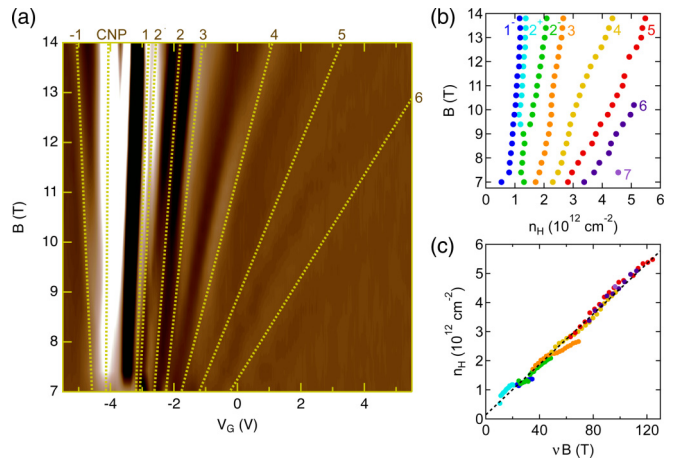
FIG. 4. Fan diagram. (a) Plot of \frac{d^2 \log R_{xx}}{dV_g^2} (arbitrary units) as a function of B and V_g for sample A. A smoothing procedure prior to each differentiation was performed to increase the signal to noise ratio. (b) Position of the maxima in (a), as extracted with a peak finding algorithm, as a function of the carrier density n_H , determined from the Hall effect, as shown in Fig. 2. (c) Same data as in (b), but plotted as \nu B , where \nu is the filling factor, which collapse on a single straight line. Labels in (a) and (b) indicate the Landau level N .
