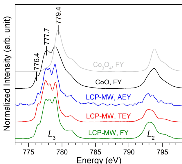
Fig. 5 Normalized soft XAS Co L_{2,3} -edge spectra of LCP-MW recorded in the AEY (blue), TEY (red), and FY (green) modes in comparison to the FY modes of the reference compounds CoO (black) and \text{Co}_3\text{O}_4 (grey). The energies corresponding to \text{O}_h \text{Co}^{2+} (776.4 eV), \text{Co}^{2+} (777.7 eV), and \text{Co}^{3+} (779.4 eV) are indicated.
