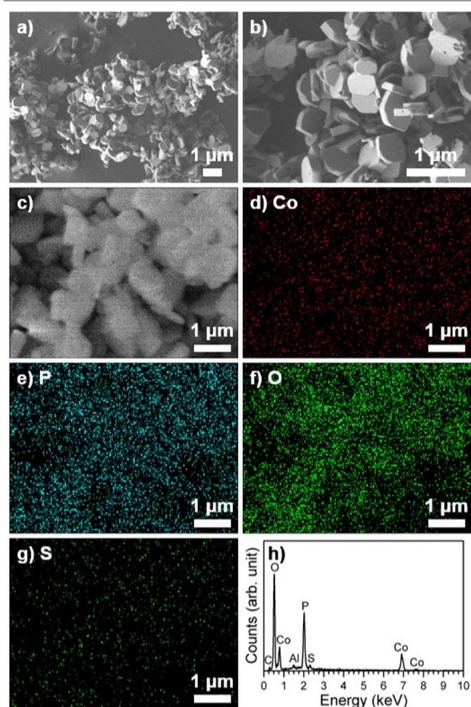
Fig. 3 (a,b) SEM images of LCP-MW recorded at 1 keV (GB mode), (c,d,e,f,g) SEM image and EDS maps for Co, P, O, and S obtained at 15 keV to optimize EDS signals, and (h) representative EDS spectrum. The C and Al signals derive from the carbon tape and the aluminum holder used for the measurement.
