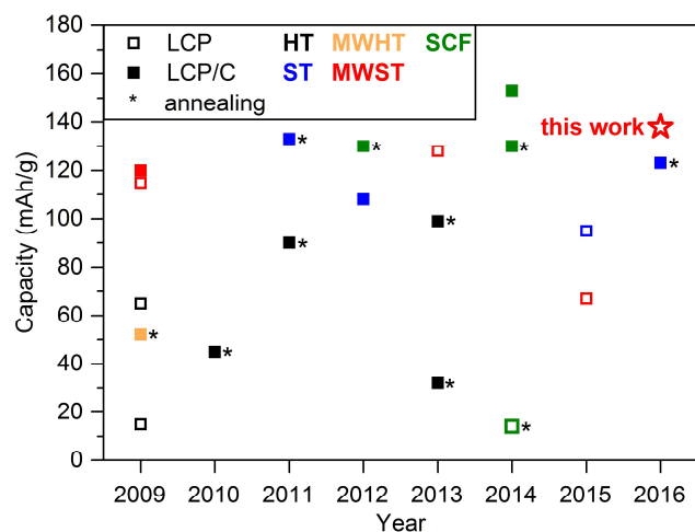
Fig. 7 Comparison of the initial discharge capacities obtained for \text{LiCoPO}_4 and carbon-coated \text{LiCoPO}_4/\text{C} materials synthesized via hydrothermal (HT), 38-40, 42 solvothermal (ST), 42-44, 53, 90 microwave-assisted hydro- (MWHT) 47 and solvothermal (MWST), 48, 50, 51 and supercritical fluid (SCF) 28, 29, 55, 78 procedures as reported between 2009 and 2016. Asterisks mark materials that underwent additional post-heat treatments at high temperatures. The star represents the capacity reached in this work using a MWST approach, which is the best reported for an untreated LCP-type material to date.
