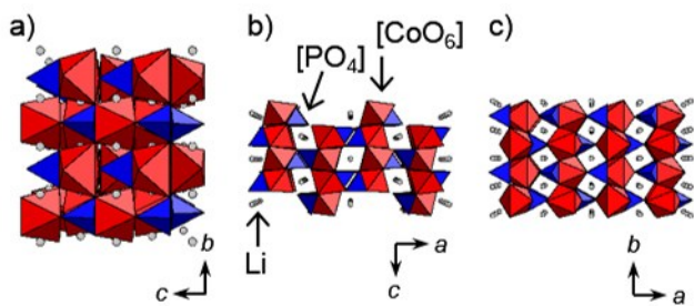
Fig. 1 Projections of the crystal structures of olivine-type \text{LiCoPO}_4 (space group Pnma ) along the three crystallographic axes: (a) [100], (b) [010], and (c) [001]. [\text{CoO}_6] octahedra are drawn in red, [\text{PO}_4] tetrahedra in blue, and Li ions in grey.
