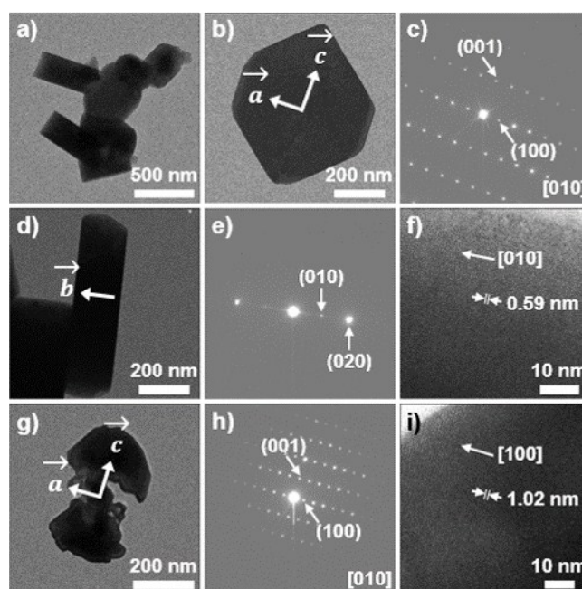
Fig. 4 TEM images, corresponding SAED (selected area electron diffraction) patterns, and HRTEM images of LCP-MW: (a) overview image, (b,c) frontal view of a hexagonal platelet, (d,e,f) side view of a platelet, and (g,h,i) particle with a porous structure as a result of the removal of the water soluble \text{Li}_2\text{SO}_4 impurity.
