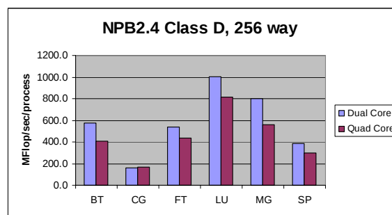
Figure 4. Comparison of NPB 2.4, Class D, 256 way benchmark performance between dual core and quad core nodes on Franklin.
