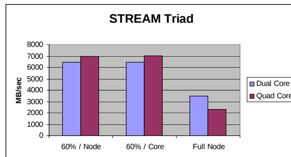
Figure 3. Comparison of STREAM Triad benchmark performance between dual core and quad core nodes on Franklin.
