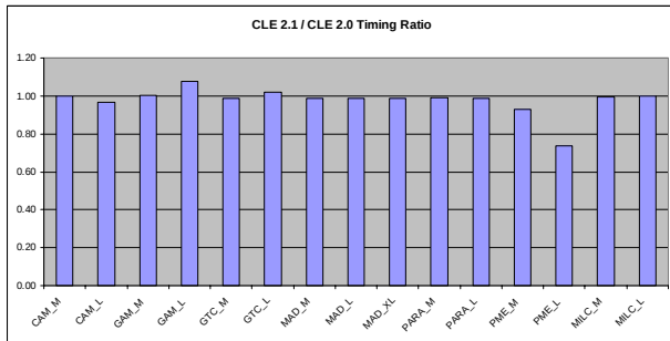
Figure 12 CLE 2.1 to CLE 2.0 run time ratio of application benchmarks on Franklin.
