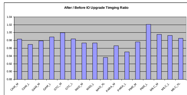
Figure 17. After and before IO upgrade run time ratio of application benchmarks on Franklin.
