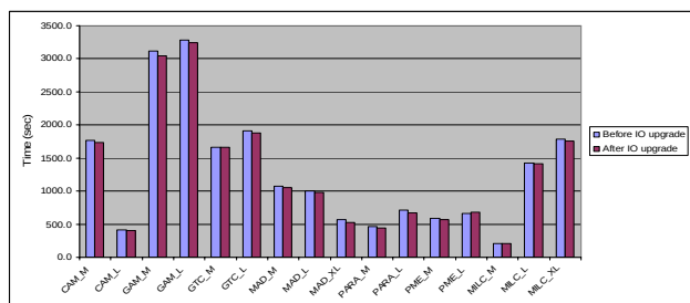
Figure 16. Comparison of application benchmarks performance before and after IO upgrade on Franklin.
