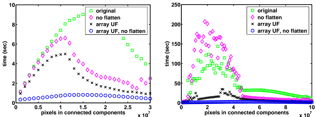
Figure 6. Timing results of four implementations of Fiorio’s algorithm. The algorithms with array based Union-Find (marked ‘Array UF’) clearly require less time the those with pointers.
