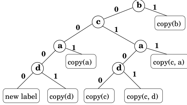
Figure 2. The decision tree used in scanning for 8-connected neighbors.
