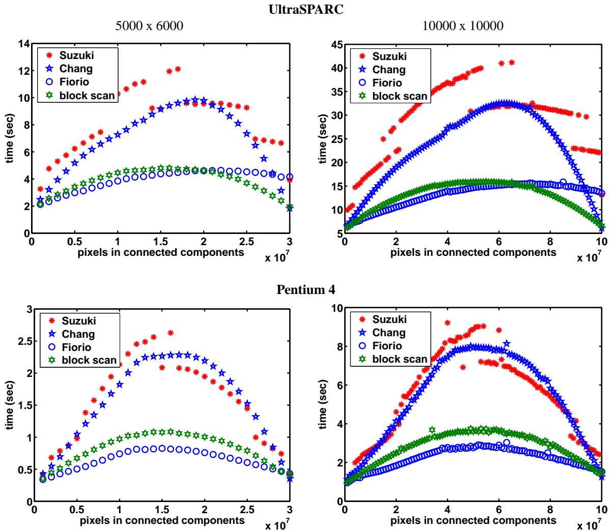
Figure 7. Timing results of four different algorithms, the modified version of Suzuki’s algorithm, the version of Fiorio’s algorithm with the array based Union-Find and without flattening, the in-place version of Chang’s algorithm, and a block scan algorithm.
