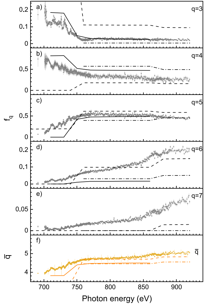
Figure 5. Product charge-state fractions f_q populated by photoionization of \text{Fe}^{2+} for panels (a) q = 3 , (b) q = 4 , (c) q = 5 , (d) q = 6 , and (e) q = 7 : experimental results (gray symbols) are compared to our MCDF computations (full lines) and to the theoretical results by Kaastra & Mewe (1993, dashed lines) and by Kučas et al. (2019, 2020, dashed-dotted lines), both weighted by the subshell-specific photoionization cross sections of Verner et al. (1993) that are displayed in Figure 3. There is no full line in panel (e) since our MCDF cascade model does not predict any seven-fold charged product ions. Panel (f): mean charge state derived from the experimental data (orange symbols) and our cascade calculations (full line). The dashed lines and dashed-dotted lines result from the subshell specific charge fractions of Kaastra & Mewe (1993) and of Kučas et al. (2019, 2020), respectively, in combination with the subshell specific ionization cross sections of Verner et al. (1993).
