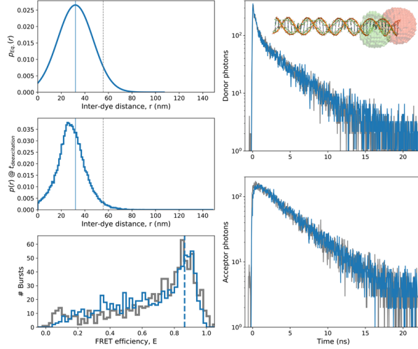
Figure 7: Fitting results to measurements of dsDNA with donor and acceptor separated by 7 bp. nsALEX smFRET measurements of a dsDNA labeled with ATTO 550 and ATTO 647N as donor and acceptor dyes, separated by 7 bp (d7 molecule) were taken. The experimental results are shown in grey and the best fit MC-DEPI simulation of a Gaussian distance distribution is shown in blue. The best fit parameters are a single Gaussian p_{Eq.}(r) with \mu=32 \text{ \AA} and \sigma=15 \text{ \AA} , together with distance dynamics \tau_c=0.93 \text{ ns} corresponding to D=484 \text{ \AA}^2/\text{ns} (using the transformation in Eq. 12). Additionally, the best fit parameter values of the acceptor photoblinking were \tau_{triplet}=2.04 \text{ ms} with blinking probability p_{Blinking}=0.0295 . The single Gaussian p_{Eq.}(r) is shown (Left-top). Note that the distribution of distances at the time of donor de-excitation, p(r)@t_{deexcitation} , is different than the one at the time of excitation (in equilibrium), p_{Eq.}(r) , mainly at the long distance range, due to the diffusion-enhanced effect. These results fit well with the FRET histogram (Left-bottom) and with the donor and acceptor fluorescence decays (Right-top and bottom, respectively). Note that here the simulated fluorescence decays are shown after convolution with the experimental IRFs. The depiction of the dsDNA molecule with donor and acceptor dyes separated by 7 bp (shown are the dyes available volumes in green and red, respectively), is shown in the inset of the Right-top panel.
