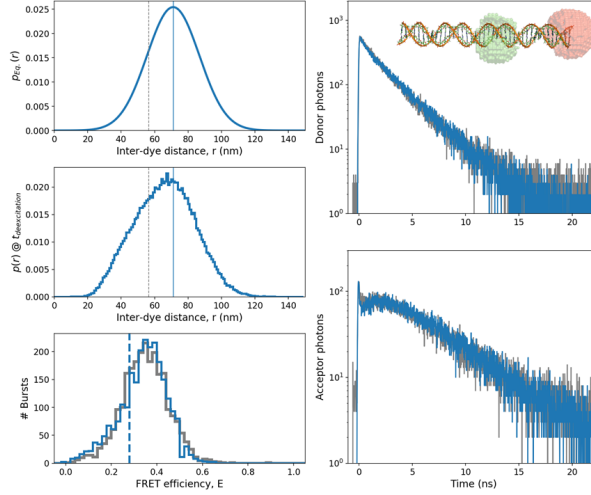
Figure 8: Fitting results to measurements of dsDNA with donor and acceptor separated by 17 bp. nsALEX smFRET measurements of a dsDNA labeled with ATTO 550 and ATTO 647N as donor and acceptor dyes, separated by 17 bp (d17 molecule) were taken. The experimental results are shown in grey and the best fit MC-DEPI simulation of a Gaussian distance distribution is shown in blue. The best fit parameters are a single Gaussian p_{Eq.}(r) with \mu=71.1 \text{ \AA} and \sigma=15.7 \text{ \AA} , together with distance dynamics \tau_c=1.21 \text{ ns} corresponding to D=407 \text{ \AA}^2/\text{ns} (using the transformation in Eq. 12). The single Gaussian p_{Eq.}(r) is shown (Left-top). Note that the distribution of distances at the time of donor de-excitation, p(r)@t_{deexcitation} , is different than the one at the time of excitation (in equilibrium), p_{Eq.}(r) due to the diffusion-enhanced effect. These results fit well with the FRET histogram (Left-bottom) and with the donor and acceptor fluorescence decays (Right-top and bottom, respectively). Note that here the simulated fluorescence decays are shown after convolution with the experimental IRFs. The depiction of the dsDNA molecule with donor and acceptor dyes separated by 17 bp (shown are the dyes available volumes in green and red, respectively), is shown in the inset of the Right-top panel.
