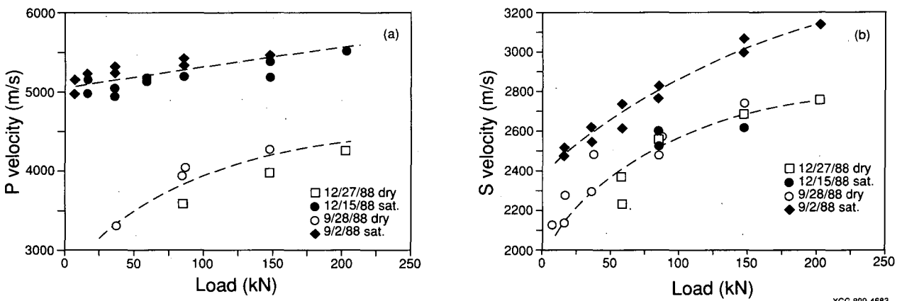
Figure 3.17. Comparison of velocities for dry and saturated conditions, fractured specimens, low frequency transducers; (a) P-wave; (b) S-wave.
