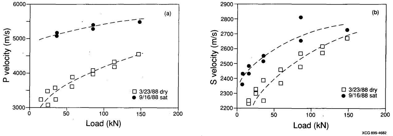
Figure 3.16. Comparison of velocities for ambient and saturated conditions, intact specimens, low frequency transducers; (a) P-wave; (b) S-wave.
