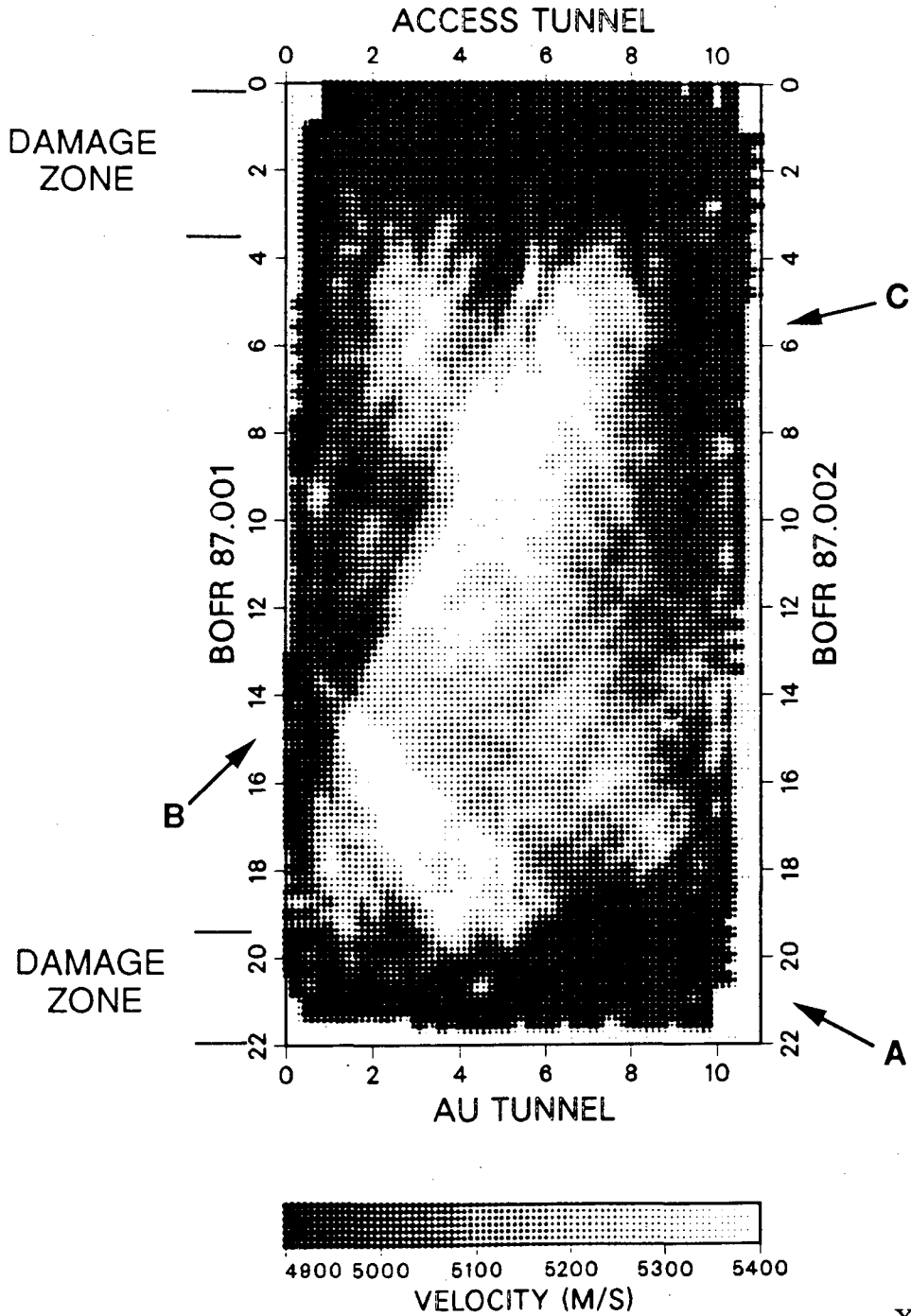
Figure 4.10. The final 1987 inversion after correcting for anisotropy.
