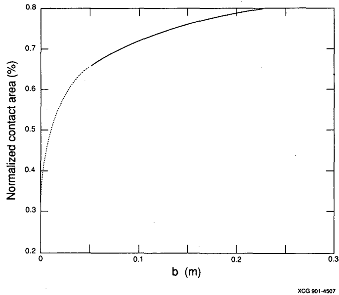
Figure 6.10. Normalized contact area of fracture faces as a function of crack half spacing b for a deformation of 1.42 \times 10^{-6} m.
