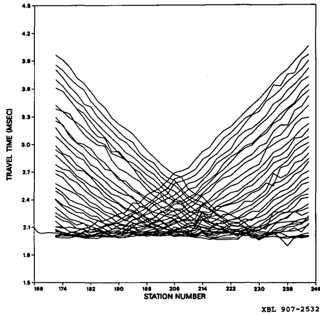
Figure 4.5. The travel time versus station number for the 1987 crosshole data, compare to Figure 4.6a.
