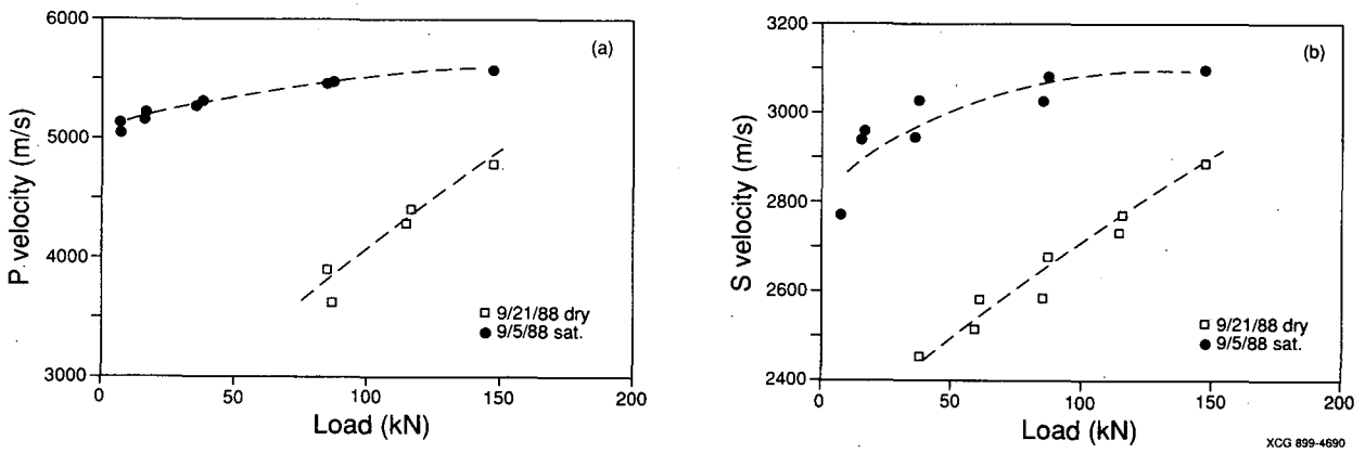
Figure 3.19. Comparison of velocities for dry and saturated conditions, fractured specimens, high frequency transducers; (a) P-wave (b) S-wave.
