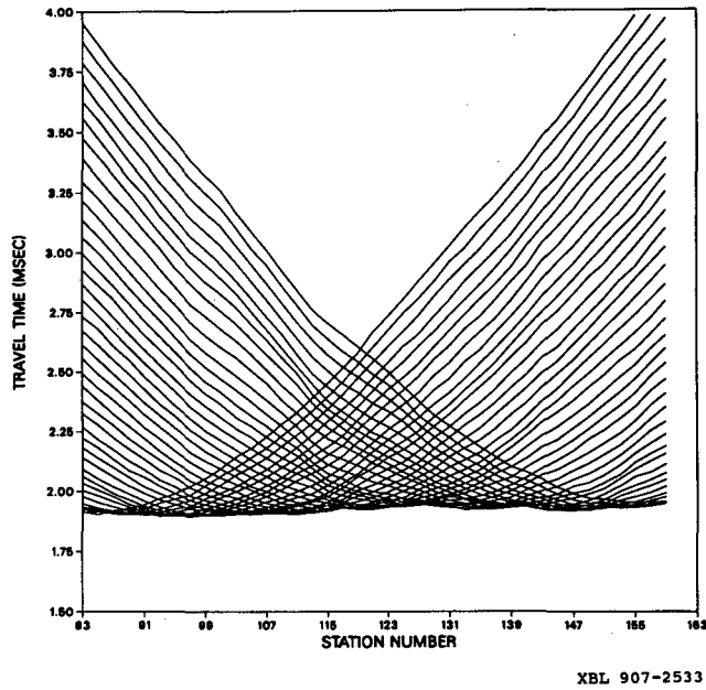
Figure 4.6a. Travel time versus station number from the 1988 crosshole paths for rays actually used in the final inversion.
