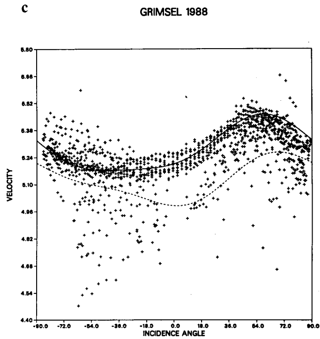
Figure 4.4. (a) 1988 travel time versus distance data; (b) 1988 velocity versus distance data; and (c) 1988 velocity versus incidence angles. The dashed line is the least square fit of the data for the 1987 data, the solid line is the fit for the 1988 data, compare to Figure 4.3 for 1987 data.
