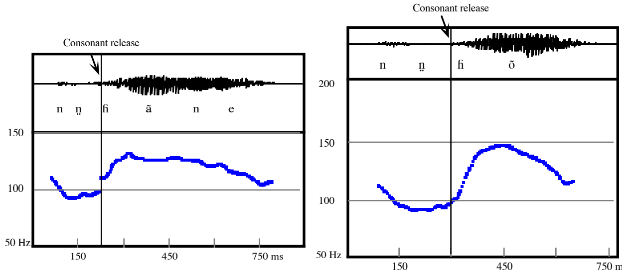
Figure 14. Pitch effects of depressor nasals in the Giriyama words /nhane/ ‘eight’ (left panel) and ideophone /nho/ (right panel). Recording courtesy of Constance Kutsch Lojenga.
