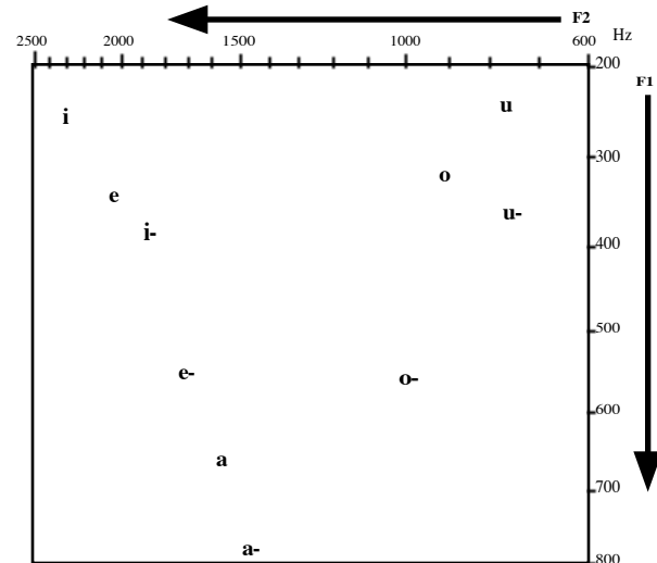
Figure 7. Nande vowel formant means. Each point represents the mean of between 6 and 21 tokens of phonetically long vowels in penultimate position in words spoken by a male speaker. Data from Ngessimo Mutaka; measurements by the author.
