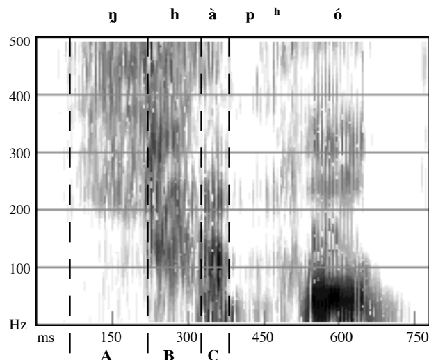
Figure 22. Spectrogram of the Nyamwezi word /ŋapo/ “basket”. See text for discussion of the phonetic segmentation.
