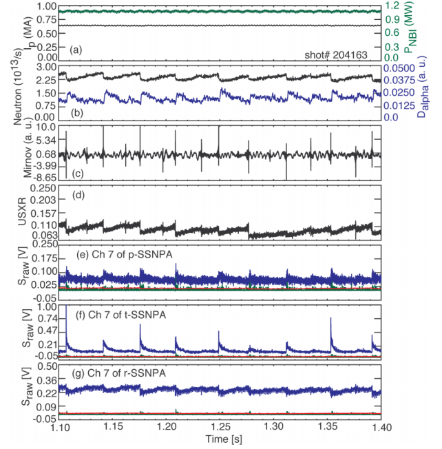
FIG. 5. Temporal evolution of (a) plasma current and injected NB power, (b) neutron rate and midplane D_{\alpha} , (c) low frequency ( <50 kHz) Mirnov signal, (d) soft x-ray, (e) channel 7 of p-SSNPA, (f) channel 7 of t-SSNPA, and (g) channel 7 of r-SSNPA. The “blind” detector signal and the estimation of x-ray induced noise are also shown in (e)-(g) with green and red curves, respectively.
