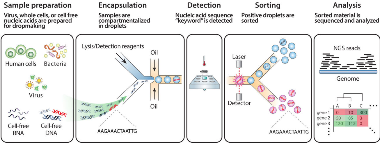
Figure 1. Nucleic acid cytometry is a general method for isolating nucleic acids based on the presence of a keyword sequence. The workflow encapsulates material, detects specific DNA or RNA sequences, and sorts droplets containing those sequences. Sorted droplets are amenable to numerous downstream analysis techniques.
