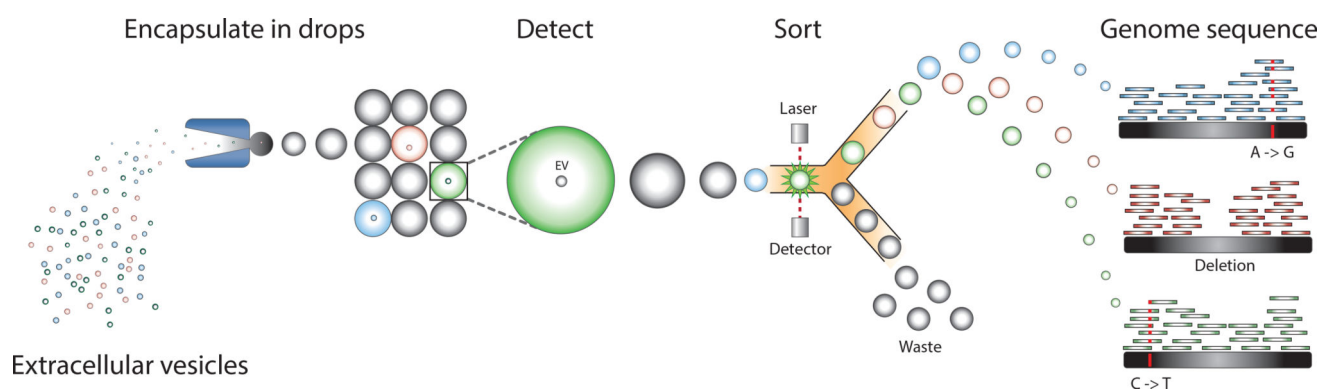
Figure 4. Sorting and sequencing of extracellular vesicles. EVs are sorted based on the presence of miRNA and genome sequenced, revealing the genotype of their cellular origin.
