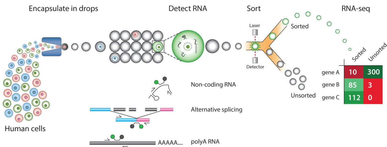
Figure 3. Sorting and sequencing cells based on specific RNA expression. Whole cell nucleic acid cytometry encapsulates single cells in droplets and detects RNA using reverse transcription PCR. Sorting and RNA-seq on positive drops is used to understand the transcriptional landscape of cells with disease-specific transcription, alternative splicing, or non-coding RNA.
