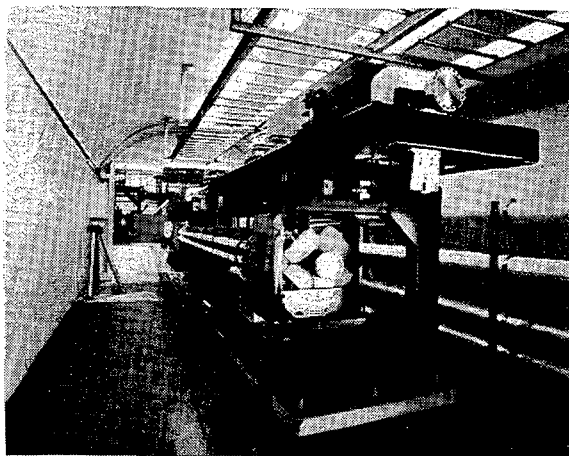
Fig. 1 Mockup of PEP-II magnets and supports.
