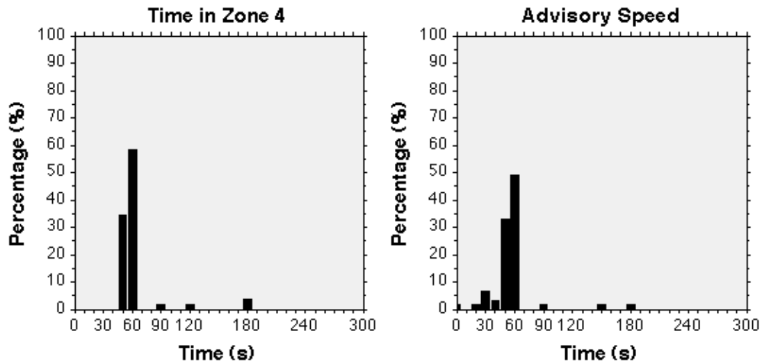
Figure 6.12: Duration of Time in Zone 4 and Time that the Advisory Speed was Constant in Zone 4.
