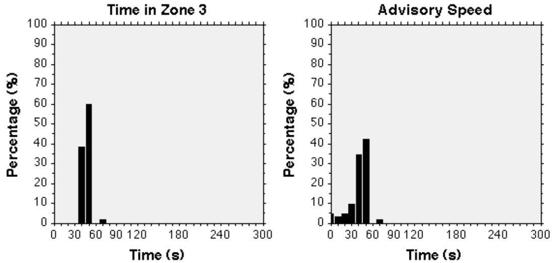
Figure 6.11: Duration of Time in Zone 3 and Time that the Advisory Speed was Constant in Zone 3.
