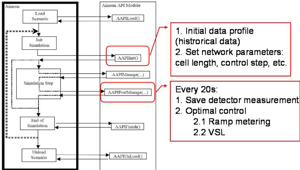
Figure 5.8. Software structure
