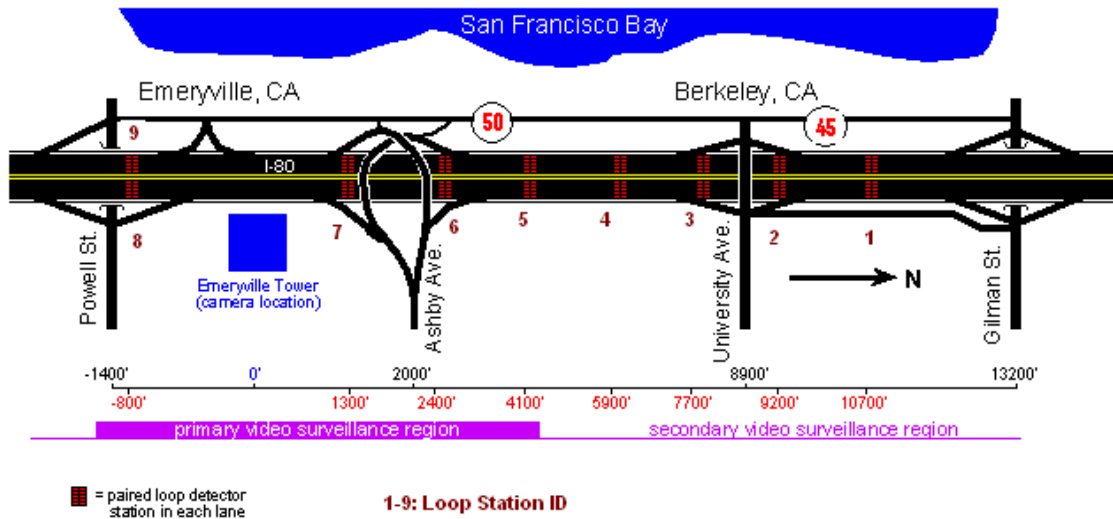
Figure 4.2. BHL Section of I-80 with Two VSL Sign Locations
