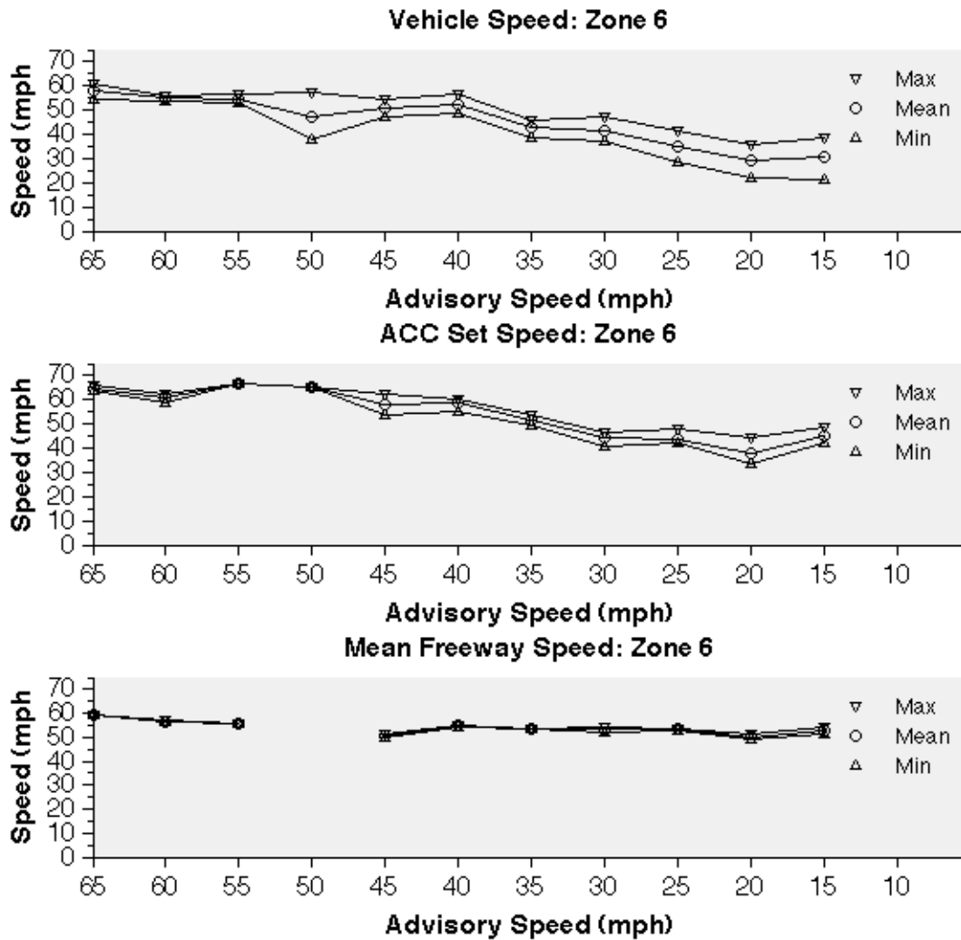
Figure 6.20: Driver Compliance with Advisory Speeds in Zone 6.
