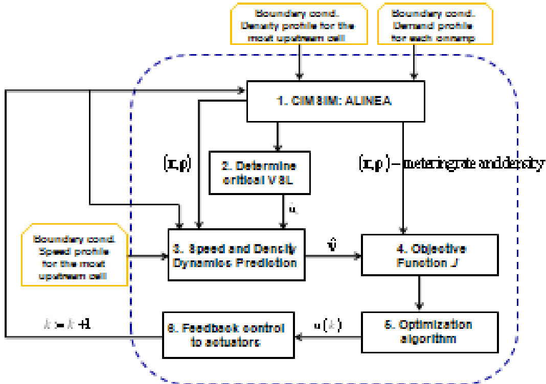
Figure 4.1. MPC Scheme to Determine VSL
