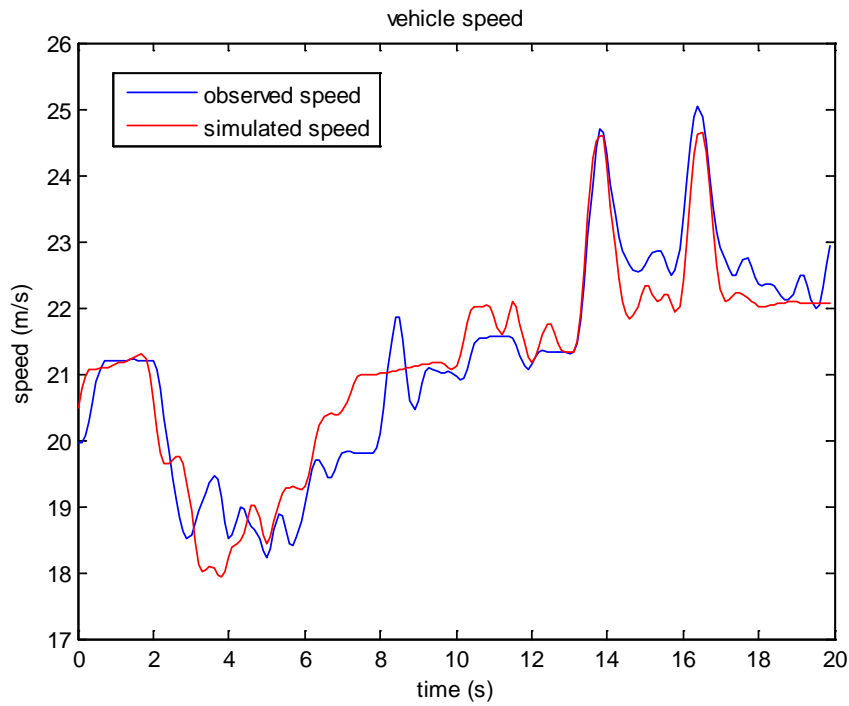
Figure 5.5a Example of Simulated and Observed Speed in the Calibration
