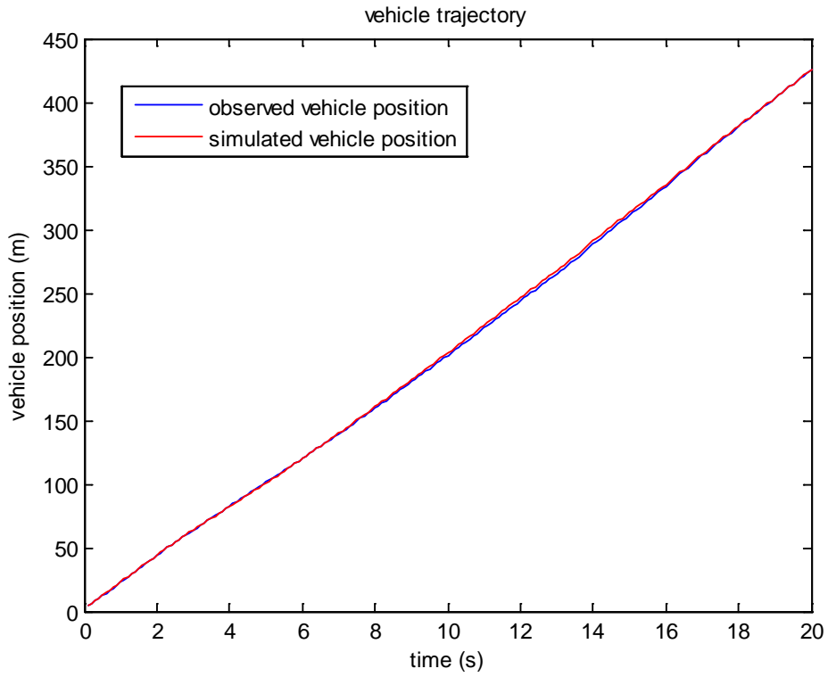
Figure 5.5b. Example of Simulated and Observed Trajectory in the Calibration
