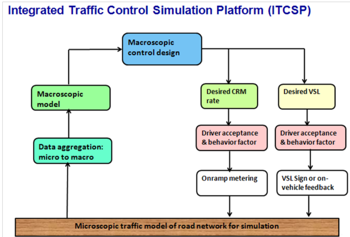
Figure 5.4. Overall Structure of ITCSP
