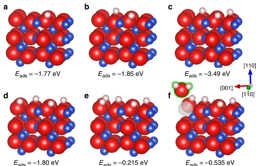
Fig. 6 DFT modeling of \text{H}_2\text{O} formation on \text{CuO} . a–e Minimum-energy structures of the \text{CuO} ( \bar{2}20 ) surface with the sequential adsorption of H atoms to form OH groups that remain stable at the surface. f Adsorption of the sixth H atom results in the formation of an \text{H}_2\text{O} molecule that spontaneously desorbs from the surface, resulting in an oxygen vacancy at the surface. Blue, red, pink, and gray balls represent Cu, O, H, and O vacancy, respectively.
