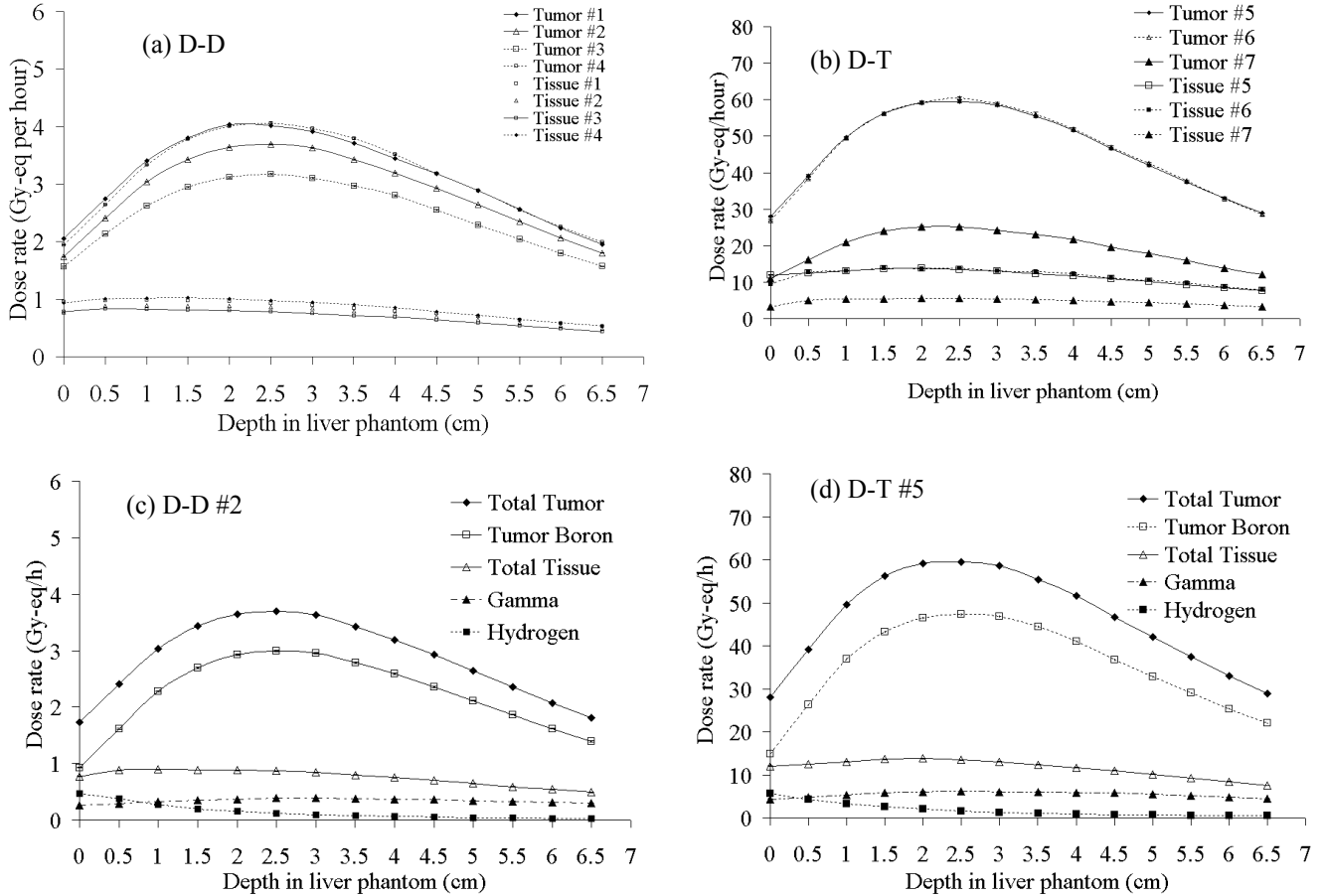
FIGURE IV. Total equivalent healthy tissue dose and tumor dose profiles in the liver phantom with the moderated D-D (a) and D-T neutron sources (b). Materials of moderator 1, 2, 4, 5, and 6 can be found in table II. In figure (c) is shown tissue and tumor depth dose distributions with the D-D moderator #2 and (d) D-T moderator #5. Neutron yield of 1.2 \times 10^{12} n/s for D-D neutrons and 4 \times 10^{13} n/s for D-T neutrons was assumed.
