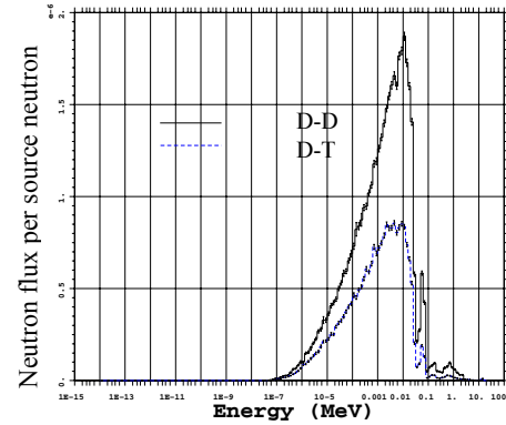
FIGURE III. Neutron energy spectra with the D-D moderator of 17 cm of Fe and 28 cm of Fluenta TM and D-T moderator of 28 cm of Fe and 30 cm of Fluenta TM .
