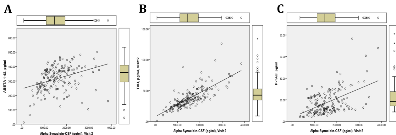
FIG. 1. Correlations among CSF alpha-synuclein ( \alpha -syn), beta-amyloid ( A\beta ) 1-42, tau, and phosphorylated tau (p-tau) in PD and healthy controls. Regression correlation among CSF \alpha -syn and A\beta 1-42, tau, and p-tau in BioFIND cohort ( n = 88 , healthy controls; n = 115 , PD). CSF \alpha -syn concentrations significantly correlate with all CSF biomarkers: (A) A\beta 1-42 ( r = 0.41 ), (B) tau ( r = 0.81 ), (C) p-tau ( r = 0.43 ); all P values < .001 . [Color figure can be viewed at wileyonlinelibrary.com ]
