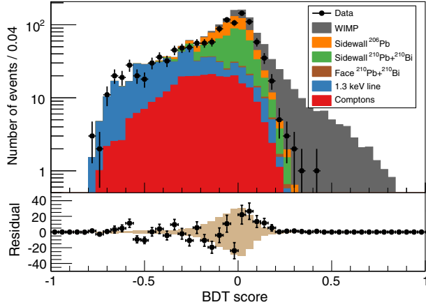
FIG. 2 (color online). Top: Stacked histogram showing the components of the background model passing the preselection criteria summed over all detectors (neutron backgrounds are negligible and not included). For comparison, a 10 \text{ GeV}/c^2 WIMP with cross section 6 \times 10^{-42} \text{ cm}^2 is shown on top of the total background. Events passing preselection criteria are overlaid (markers with statistical errors). A p -value statistic comparing the data to background model is 14% for this selection. Bottom: Difference between the data and the background expectation. Tan bars indicate the systematic uncertainty (68% C.L.) on the background estimate. Each component of the background model was computed prior to unblinding and was not fit or rescaled to match the data.
